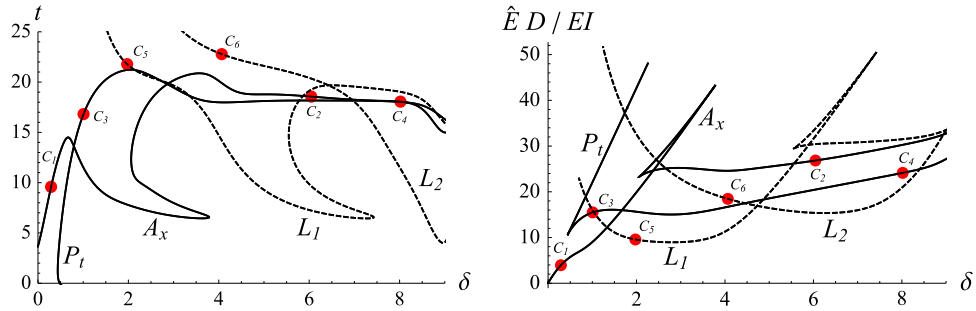
Fig. 5. Post-buckling paths: (left) force–displacement curves for f_\gamma = 20 , where t is the applied tension and \delta the end-shortening, and (right) energy \hat{E} D / EI as function of \delta . Solid lines represents both A_x configurations, where the beam shape is symmetric with respect to the axis joining the center of the disk (x_C, y_C) and the beam midpoint (x(\ell/2), y(\ell/2)) , and P_t configurations, where the beam shape is symmetric with respect to the beam midpoint P_t . Dashed lines correspond to L_1 and L_2 configurations.
