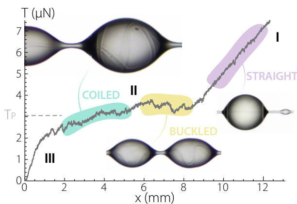
Figure 2. Shape-induced functionalization. Quasi-static force measurements on spider capture threads combined with microscopic observations demonstrate that the slack core filament is spooled into the droplets (typically 250–300 \mu\text{m} wide) along the force plateau T = T_P . For larger forces T > T_P , the fibre straightens and a spring-like behaviour is shown. The characteristic J-shape for this force-extension curve can be attributed to a shape-induced functionalization of the fibre by the glue droplets (see also Supplementary Video).
