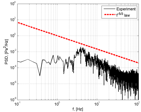
Fig. 242. Outlet log pressure power spectrum: Q = 20 [L/s]; Rm_s = 4.15
