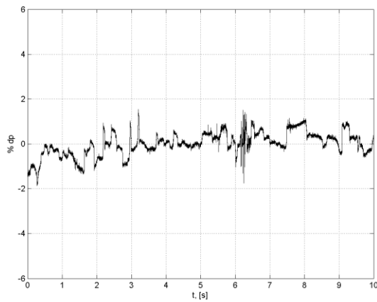
Fig. 189. Pulsations of developed pressure difference: N = 0.67 , Rm_s = 4.8 .
