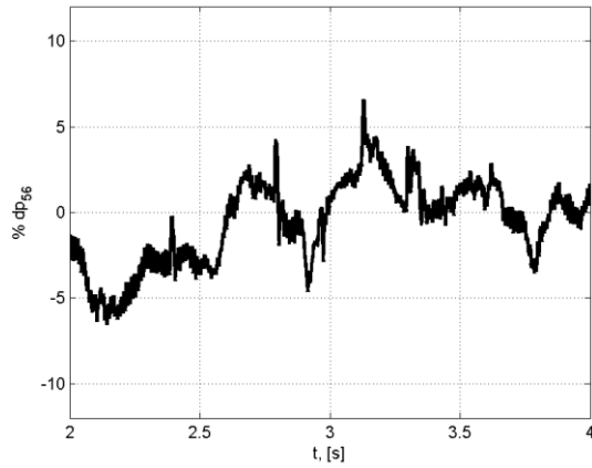
Fig. 149. Pulsations of developed pressure: Rm_s = 4.47 .
