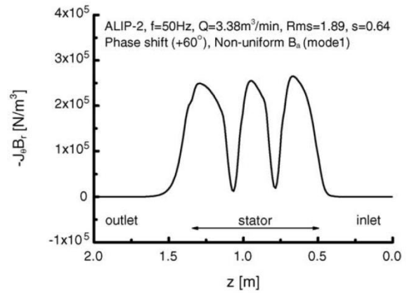
Fig. 29. EM force distribution Rms = 1.8 , non-uniform B_w , mode 1, phase shift +60^\circ . [25]
