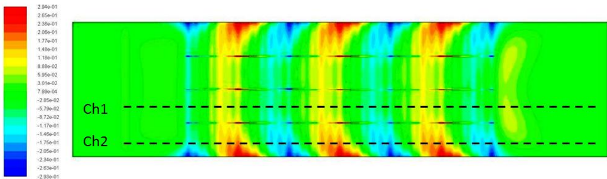
Fig. 115. Distribution of B_x [T]: Q = 45 L/s, Rm_s = 3.3 .
