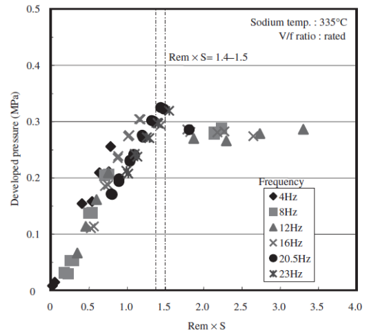
Fig. 35. Dependence of developed pressure on Rm_s . [36]
