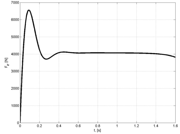
Fig. 82. Development of EM force z component: Rm_s = 1.78 ; N = 5.9 .
