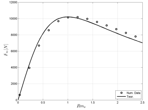
Fig. 99. Comparison of numerical and theoretical results of axial force F_z : N = 13.2 .
