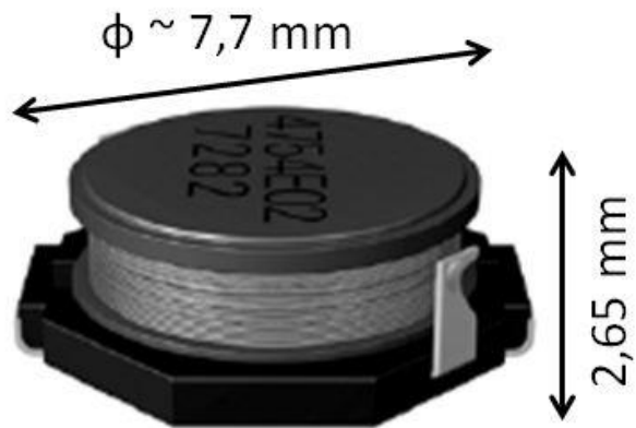
Fig. 160. EPCOS B882451N ferrite core coil.
