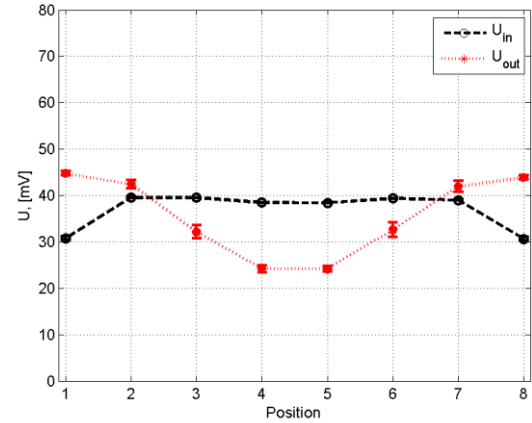
Fig. 147. Potential difference: Rm_s = 3.5 .
