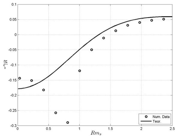
Fig. 94. Comparison of numerical and theoretical results of temporal development rate -\gamma_R : N = 1 .
