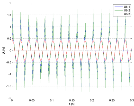
Fig. 184. Signal with sampler U8 over several periods, I = 200 [A].
