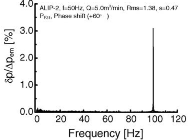
Fig. 31. Pressure pulsation spectrum: f = 50\text{Hz} , Rms = 1.38 , phase shift +60^\circ . [25]
