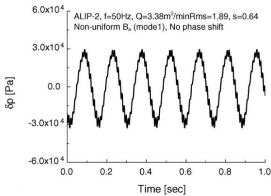
Fig. 53. Pressure pulsation at pump outlet: Rms = 1.89 , non-uniform B_a , Mode 1, no phase shift. [25]
