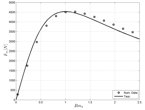
Fig. 97. Comparison of numerical and theoretical results of axial force F_z : N = 5.9 .
