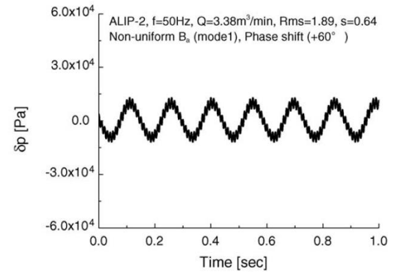
Fig. 54. Pressure pulsation at pump outlet: Rms = 1.89 , non-uniform B_a , Mode 1, phase shift +60^\circ [25]
