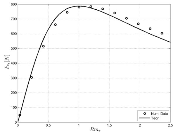
Fig. 95. Comparison of numerical and theoretical results of axial force F_z : N = 1 .
