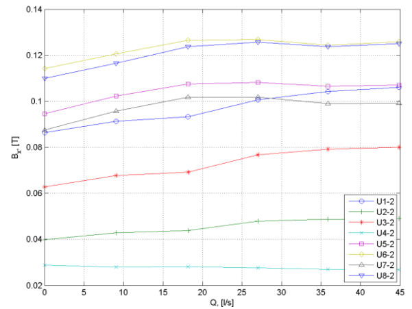
Fig. R 43. |B_x| for UX-2: N = 0.67 .
