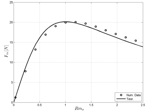
Fig. 91. Comparison of numerical and theoretical results of axial force F_z : N = 0.03 .
