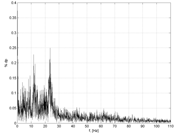
Fig. 200. Spectrum of pressure pulsations: N = 0.67 , Rm_s = 3.33 .
