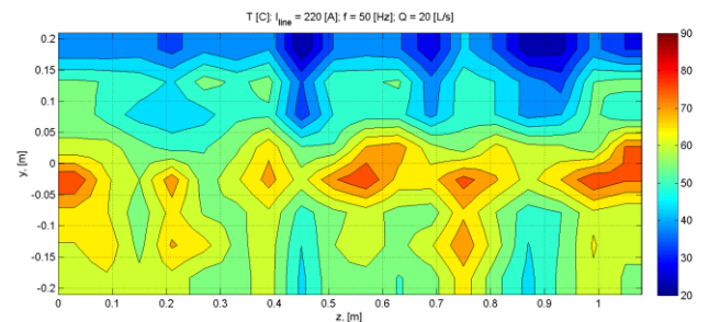
Fig. 248. T [C], Rm_s = 4.15
