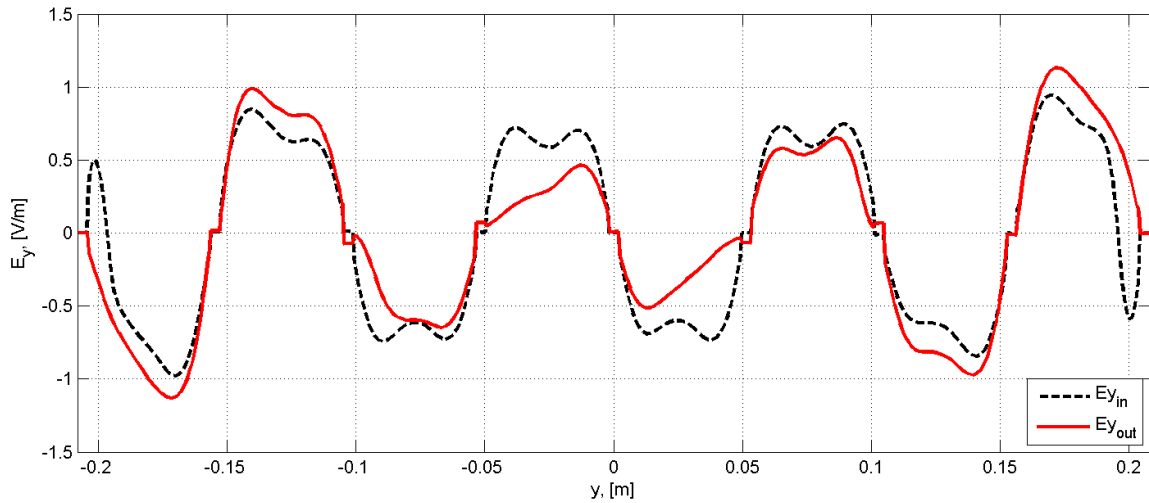
Fig. 143. Time averaged distribution of E_y [V/m]: Rm_s = 3.82 .
