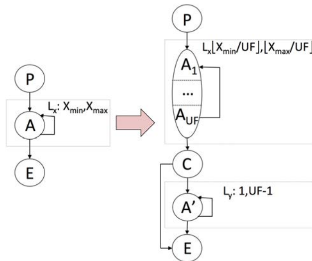
Figure 2.23 – CFG of loop unrolling example. The left part of the figure shows the original CFG, whereas the right part shows the optimized one.
