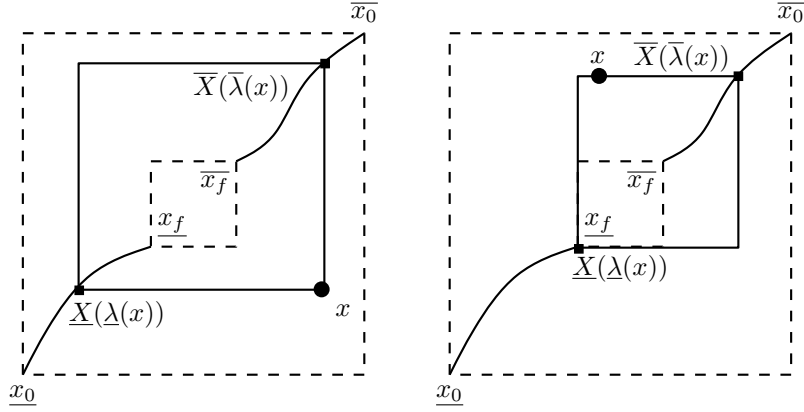
Figure 2.6 – Smallest element [\underline{X}(\underline{\lambda}(x)), \overline{X}(\overline{\lambda}(x))] of the parameterized family of robust controlled invariant intervals [\underline{X}(\lambda), \overline{X}(\lambda)] containing state x .
