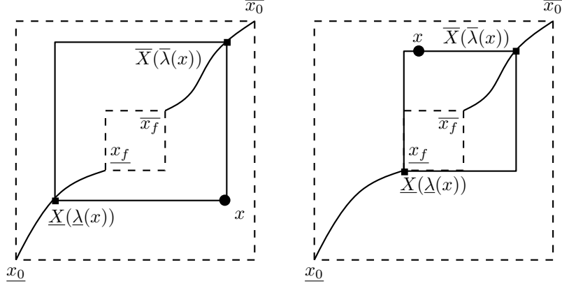
Figure 2.6 – Smallest element [\underline{X}(\underline{\lambda}(x)), \overline{X}(\overline{\lambda}(x))] of the parameterized family of robust controlled invariant intervals [\underline{X}(\lambda), \overline{X}(\lambda)] containing state x .
