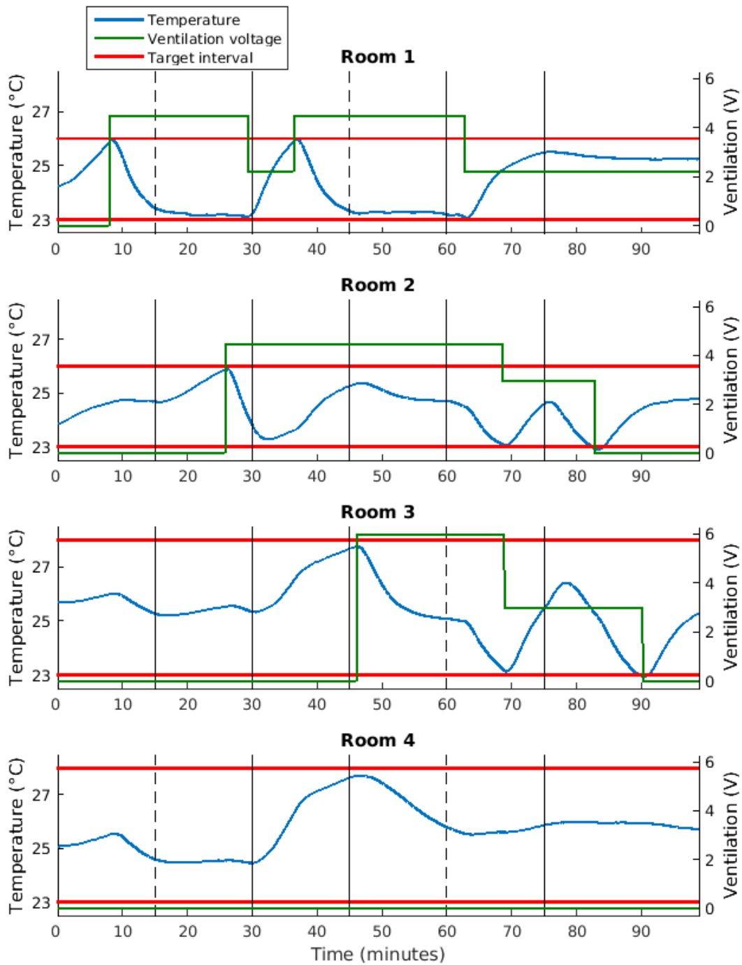
Figure 5.10 – UFAD experiment controlled with a compositional symbolic method using 1D subsystems, each with 20 symbols and 9 control values.
