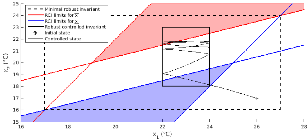
Figure 2.2 – Example 2.2: possible choices for a robust controlled invariant interval and bang-bang control.
