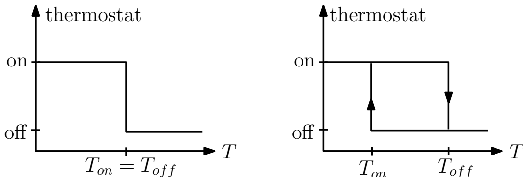
Figure 2.1 – On/off (left) and hysteresis (right) thermostat controller.
