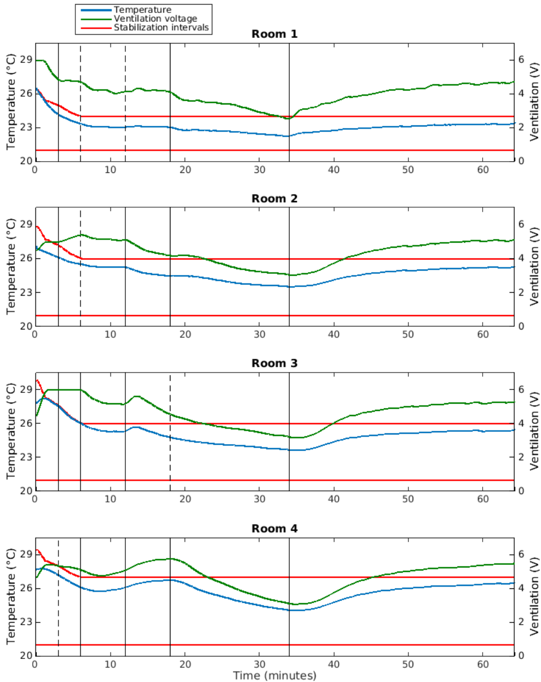
Figure 5.7 – Robust set stabilization and robust controlled invariance. Left axis: room temperature (blue) and stabilization intervals (red); right axis: fan voltage (green); vertical lines: switching times.
