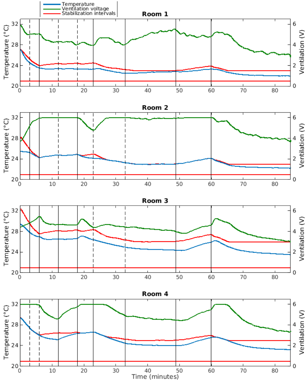
Figure 5.8 – Robust set stabilization for a non-robust controlled invariant interval (stabilization interval not strictly decreasing).
