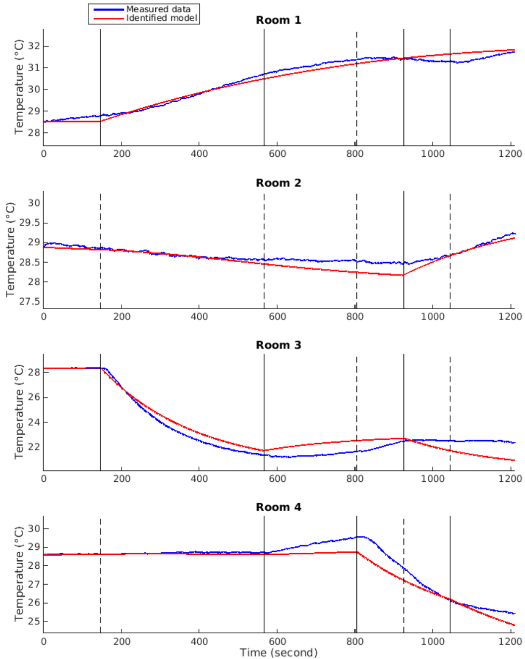
Figure 5.5 – Comparison between the identified model (red) and the experimental measurements (blue) for the evaluation scenario (events represented by vertical plain lines when linked to the room, dashed lines otherwise).
