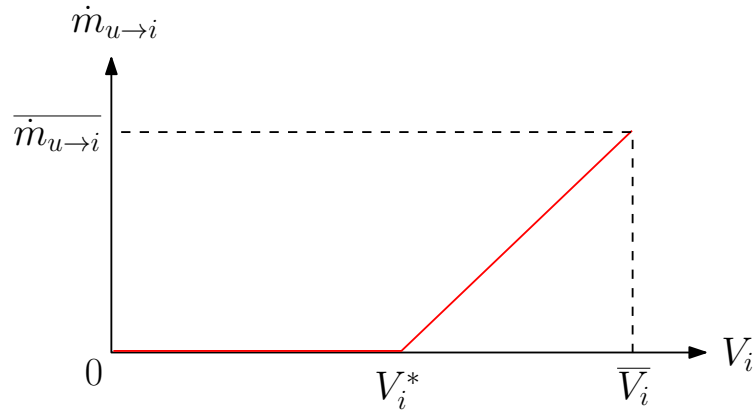
Figure 5.4 – Dry friction in the command of an underfloor fan.
