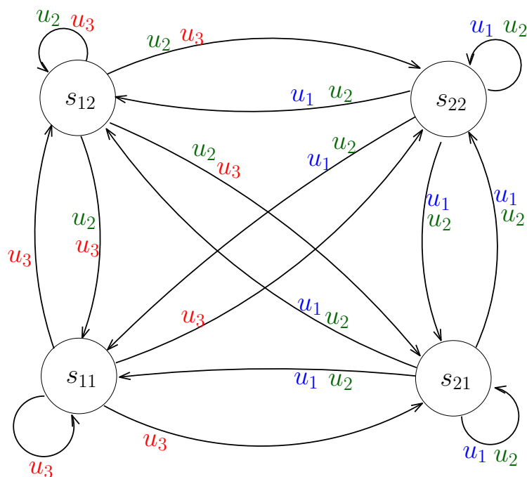
Figure 3.3 – Symbolic abstraction S_a constrained by the safety controller C_a .
