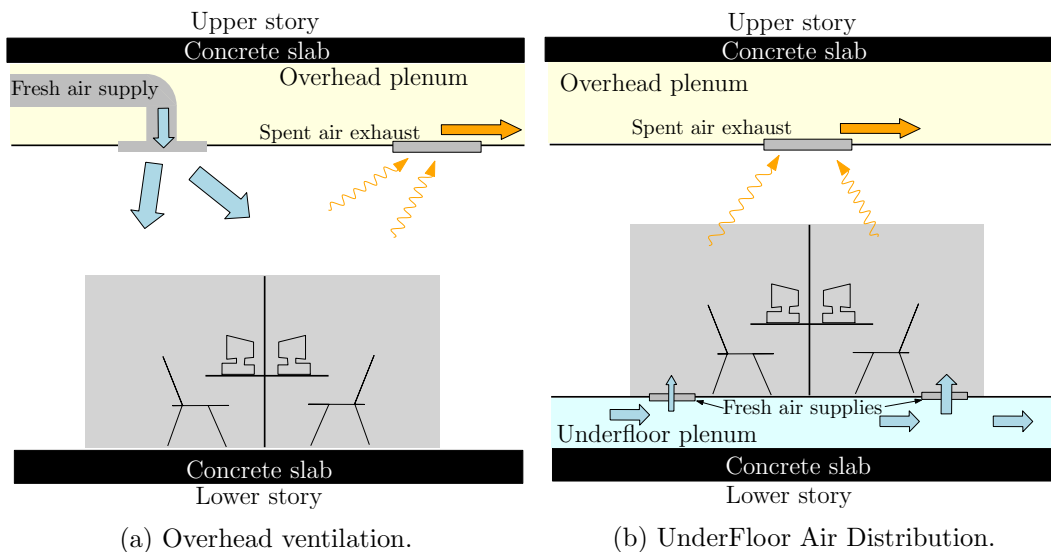
Figure 5.1 – Comparison of ventilation architectures.
