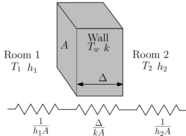
Figure 5.6 – Electrical analogy for thermal conduction and convection.
