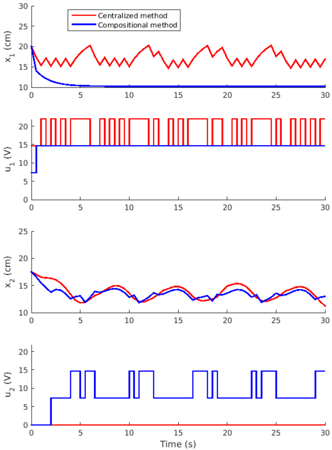
Figure 4.5 – State and control input of each tank, controlled with the centralized method (red curves) and the compositional method (blue curves).
