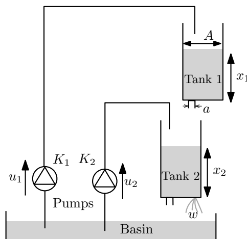
Figure 1.5 – Coupled-tank system with two pumps and a leak on tank 2.
