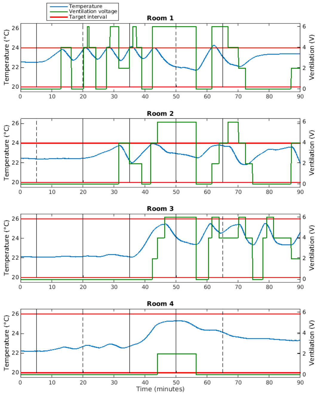
Figure 5.9 – UFAD experiment controlled with a centralized symbolic controller with 10^4 symbols and 4^4 control values. Control objective: minimize the control values, the control variations and the distance between the temperature and the center of the interval.
