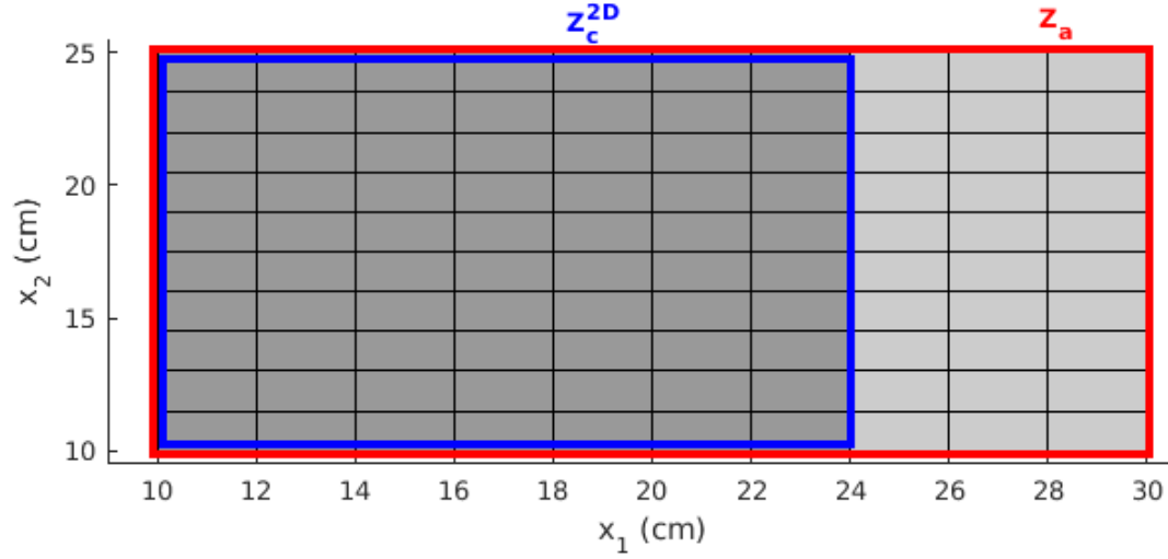
Figure 4.3 – Safe set Z_c^{2D} for the compositional approach with 2D subsystems (dark gray symbols in the blue rectangle) and safe set Z_a for the centralized approach (all symbols in the red rectangle).
