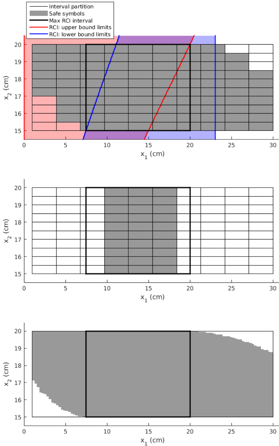
Figure 3.4 – Interval partition with safe symbols (gray), robust controlled invariance limits from Figure 2.4 (red and blue sets) and maximal robust controlled invariant sub-interval (thick black). Top: \alpha_x = 10 and \tau = 0.5 s. Center: \alpha_x = 10 and \tau = 0.1 s. Bottom: \alpha_x = 100 and \tau = 0.1 s.
