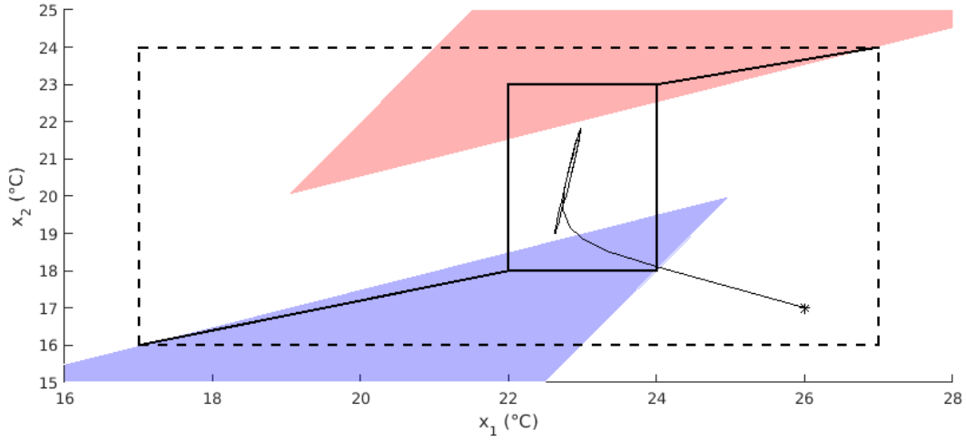
Figure 2.7 – Example 2.6: robust set stabilization with linear support functions.
