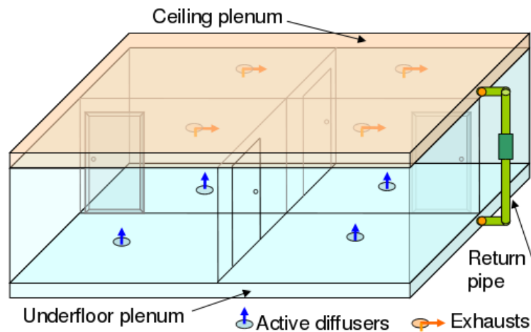
Figure 5.3 – Sketch of the 4-room UFAD building.
