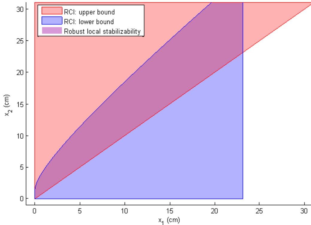
Figure 2.4 – Coupled tanks: allowed lower and upper bound for a robust controlled invariant interval (blue and red areas, respectively) and robustly locally stabilizable states (purple intersection).
