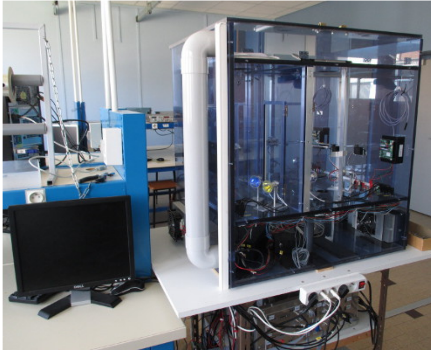
Figure 5.2 – Small-scale experiment of a flat equipped with UFAD.
