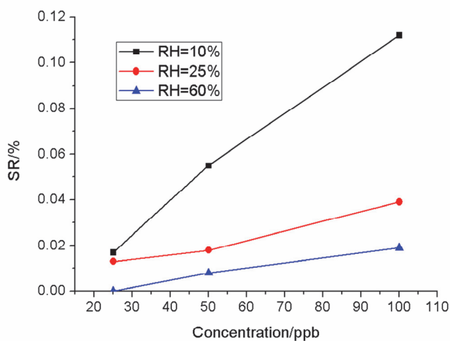
Figure 59. a) cav-Au-MWCNT sensor resistance response as a function of benzene concentration in air at 200 \text{ mL min}^{-1} with a R.H. of 25% in the background, and b) relative sensor response for benzene concentrations at different R.Hs.
