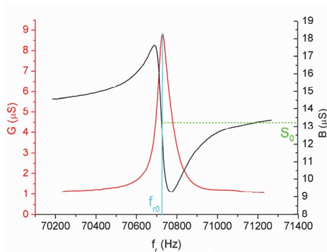
Figure 41: Resonance frequency scan measurement protocol
