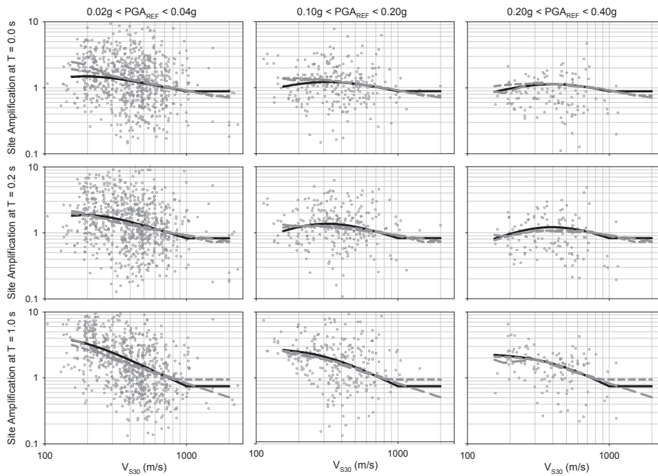
Figure 3. 5. Comparisons of the proposed site model (black solid line) with AS08 (short dashed gray curve) and BA08 (long dashed gray curve) together with the empirical data for T = 0.0\text{s} , T = 0.2\text{s} , and T = 1.0\text{s} (from top to bottom respectively). Each column represents different level of input rock motion, PGA_{REF} indicated at the top of figure.
