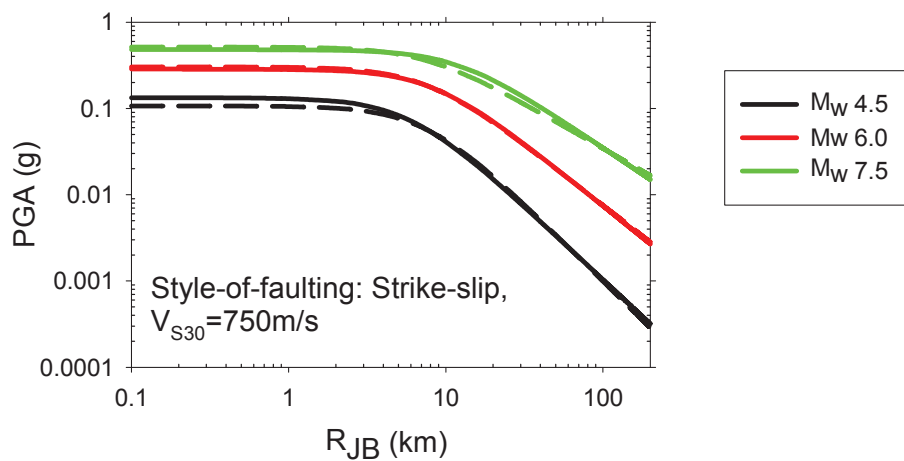
Figure 5. 2. Comparisons of magnitude-dependent and -independent distance saturation at different magnitudes for strike-slip style-of-faulting and a rock site of V_{S30} = 750 m/s. Solid and dashed lines represent with and without magnitude-dependent distance saturation, respectively.
