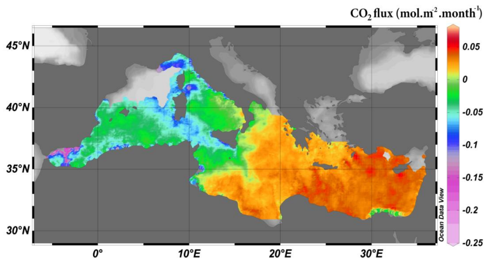
Figure 7. Air-sea CO 2 fluxes during May 2013 (using equations 1 and 2 and 3 and 8)
