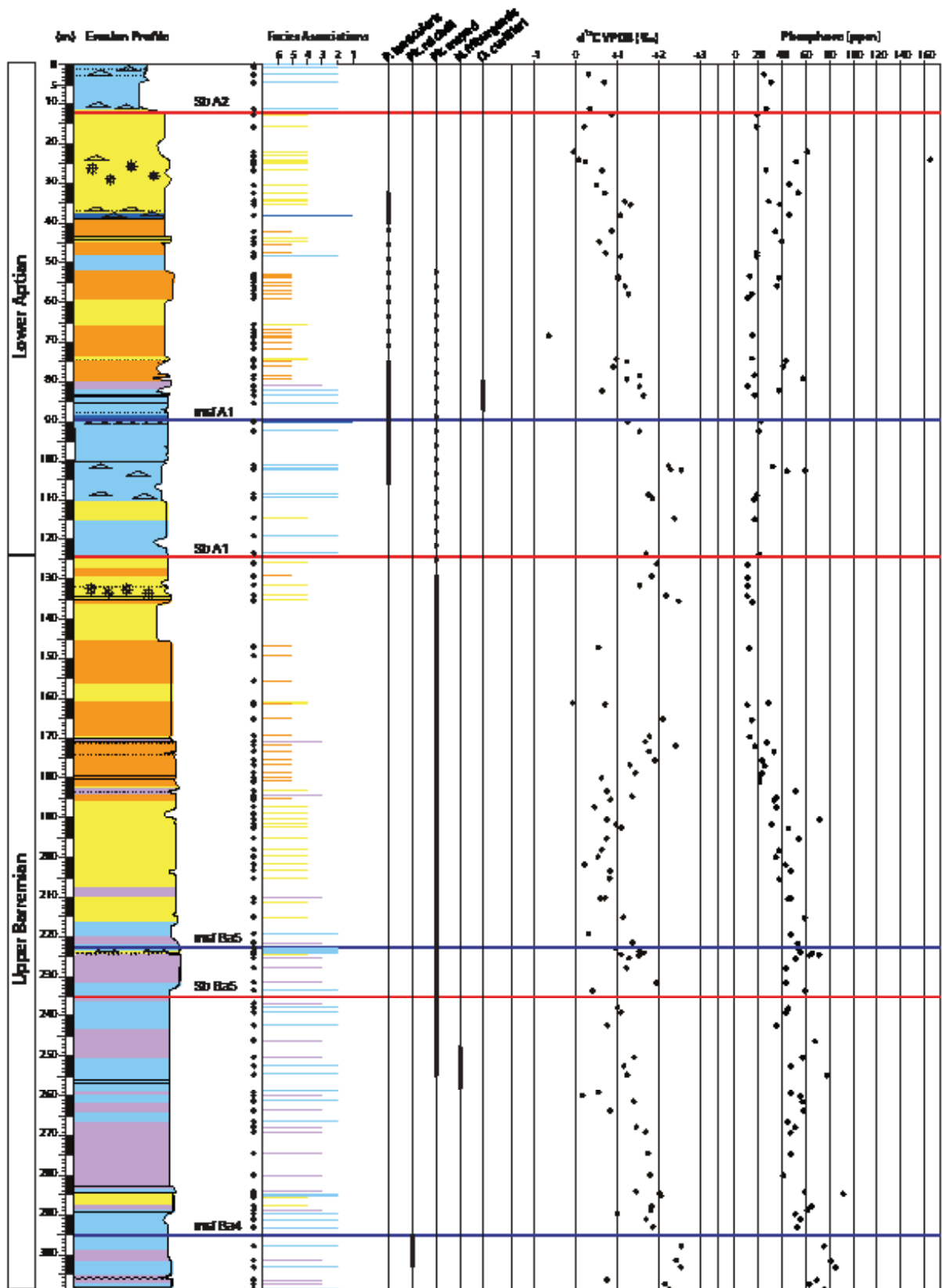
Figure 3-10 : Facies, sequence-stratigraphic subdivision, \delta^{13}C values and phosphorus concentration in the Fontaine section (Legend in Annex 1). For the colours facies legend, refer to the Figure 3-4, p. 79
