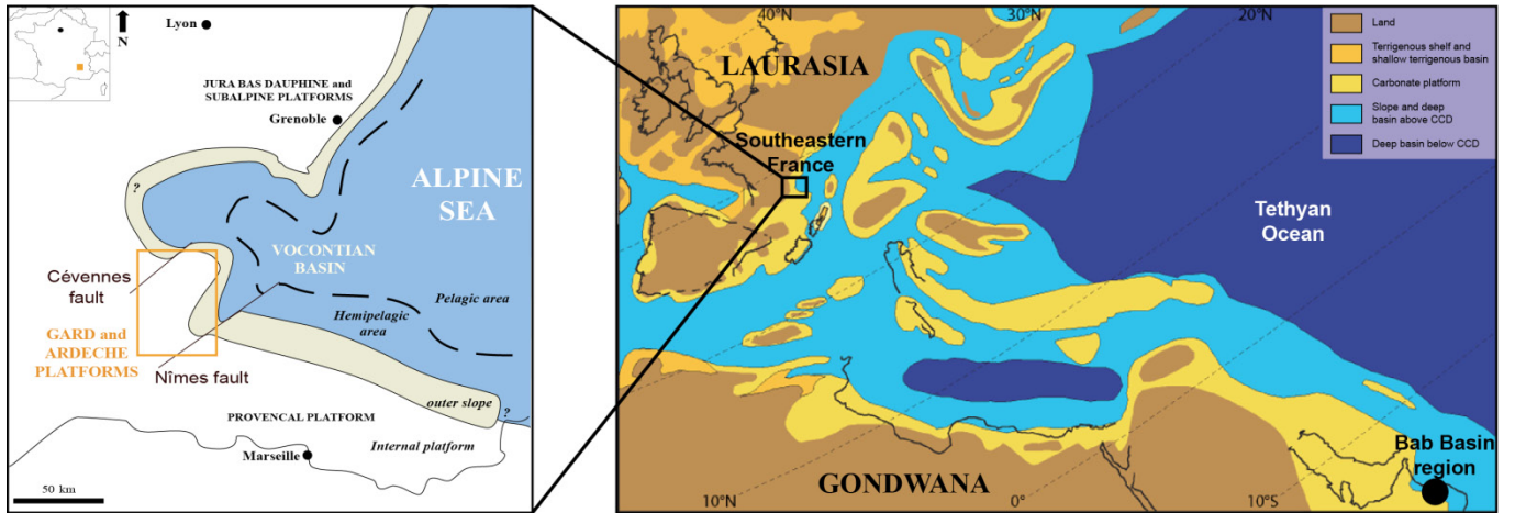
Figure 1: Paleogeography and location of the Gard and Ardèche Platforms in southeastern France in lower Aptian period, modified from H. Arnaud (1980) and Steuber et al. (2005)
