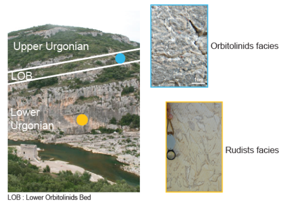
Figure 2: Stratigraphical and facies correspondance between the southeastern France Urgonian series and the Middle East KharaiB, Hawar and Shu'aiba members.
