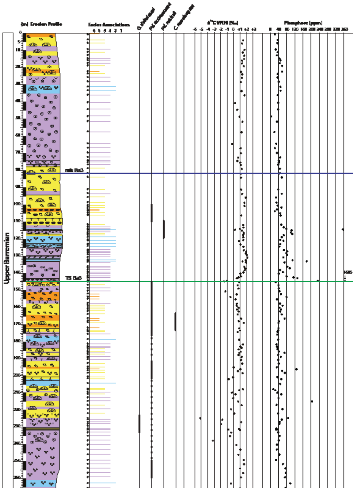
Figure 3-8 : Facies, sequence-stratigraphic subdivision, \delta^{13}\text{C} values and phosphorus concentration in the Pont de Laval section (Legend in Annex 1). For the colours facies legend, refer to the Figure 3-4, p. 79
