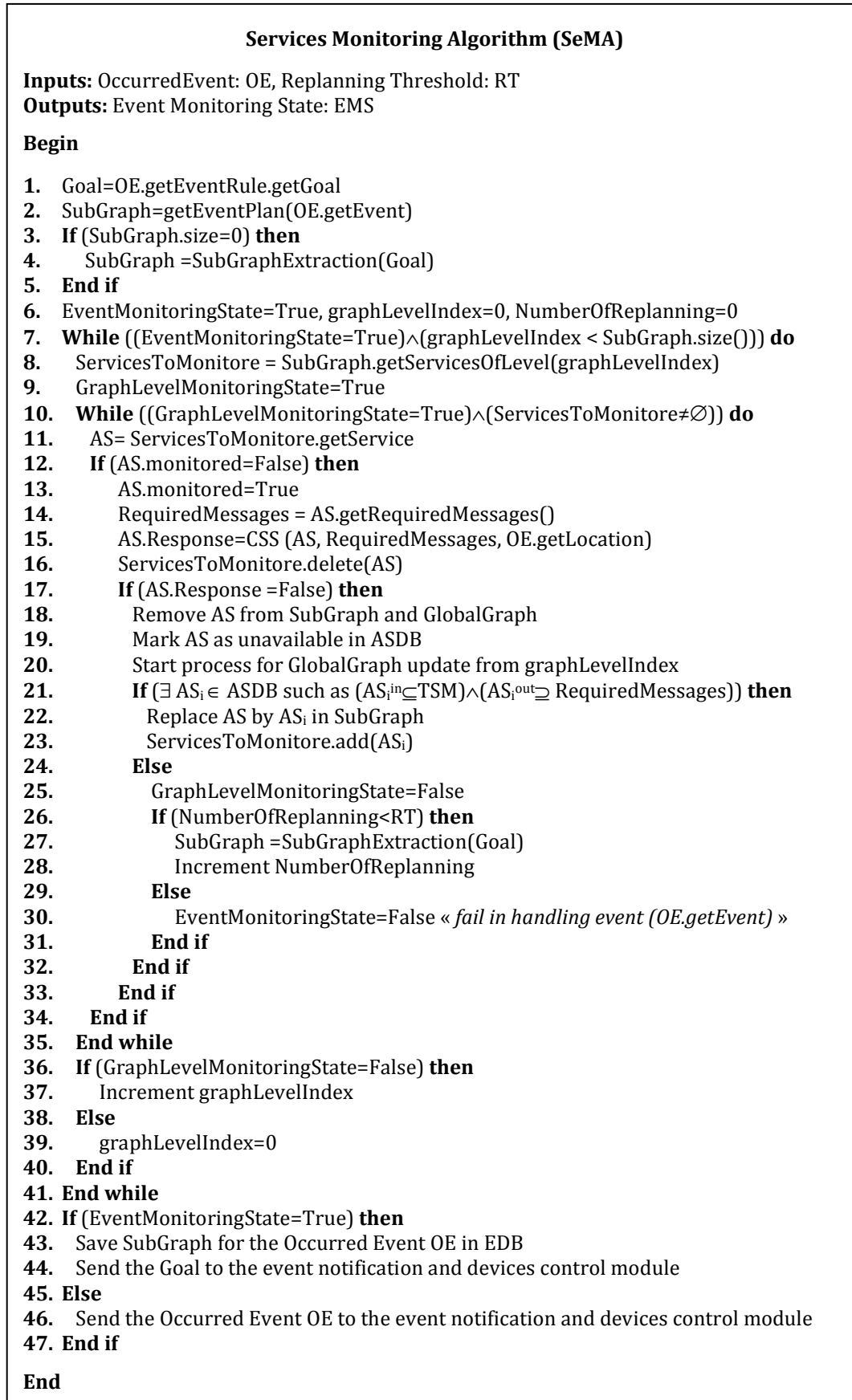
Figure 6.24 : Algorithmme de monitoring de services
