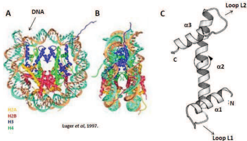
Figure 1. The nucleosome – basic unit of chromatin. (A and B) Crystal structure (at 2.8 Angstrom resolution) of the nucleosome core particle (NCP), containing 2 copies of each core histone H2A, H2B, H3 and H4 (color coded) around which 146 base-pairs of DNA double helix are wrapped. (B) Lateral view of the NCP. (C) The conserved histone fold domain. Three \alpha -helices ( \alpha 1 , \alpha 2 and \alpha 3 ) are connected by relatively unstructured linker loops (L1 and L2). Adapted from (Ramakrishnan 1997).
