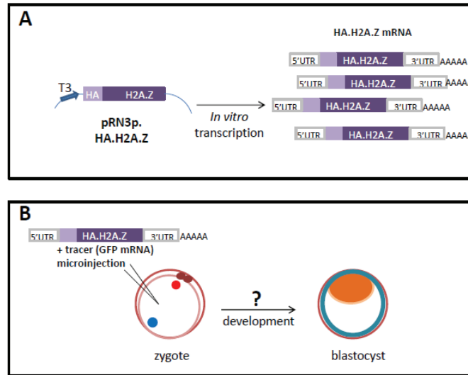
Figure 19. Experimental setup for investigating the effects of H2A.Z overexpression on embryonic development. (A) Coding sequence for mouse H2A.Z ( h2afz ) was cloned into pRN3P plasmid, with an N-terminal haemagglutinin (HA) tag. Viral T3 promoter is located upstream. mRNA was synthesized in vitro by mMessage Machine Kit using T3 polymerase. (B) HA.H2A.Z mRNA was injected into zygotes shortly after fertilization (~18 hours after hCG administration) together with mRNA coding for GFP, as a tracer. Injected embryos were placed in culture and development to blastocyst was monitored and scored.
