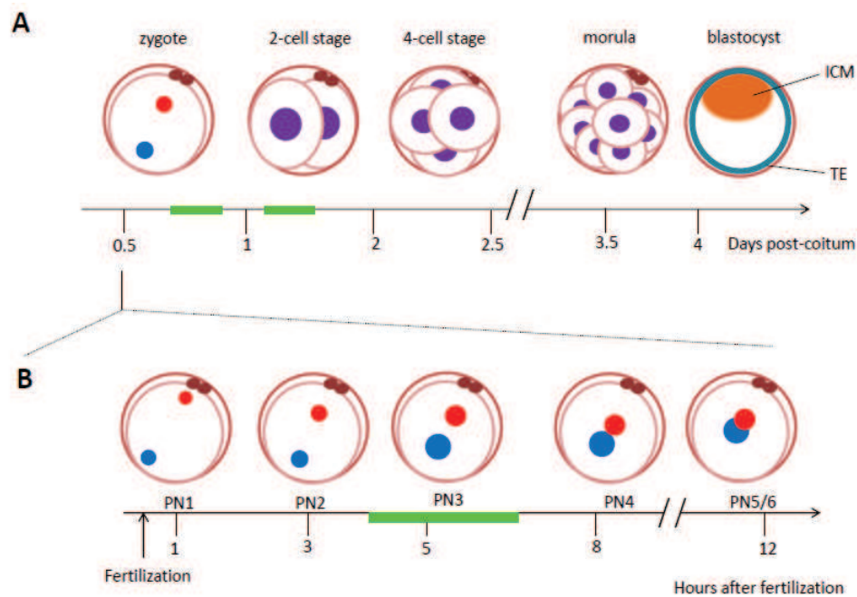
Figure 12. The stages of mouse preimplantation development. (A) Schematic representation of the stages of mouse preimplantation embryogenesis. Male and female pronuclei in the zygote are represented by blue and red circles, respectively. Green rectangle symbolises the S-phase. This figure is adapted from (Martin, Beaujean et al. 2006). (B) Schematic representation of pronuclear stages in the mouse zygotes. Positions of male (blue) and female (red) pronuclei relative to each other at different PN stages are shown. Timing of different pronuclear stages (relative to fertilization) is indicated. Green rectangle depicts S-phase, as above. Adapted from (Adenot, Mercier et al. 1997).
