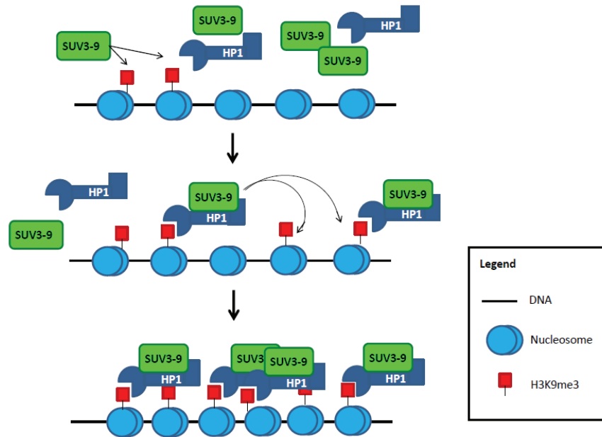
Figure 7. Deposition and spreading of H3K9me3 on chromatin. Suv3-9 represents the HMT responsible for H3K9me3 deposition. H3K9me3 is recognized by the chromodomain of HP1 proteins. HP1s can interact with Suv3-9 through their chromoshadow domain and recruit it to pre-existing H3K9me3. This feedback loop allows for spreading of H3K9me3 and expansion of heterochromatic domains.
