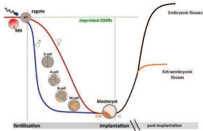
Figure 14. Levels of DNA-methylation after fertilization. Early developmental stages in mice are characterized by the sharp decrease in DNA-methylation levels, affecting both maternal and paternal DNA, and reaching lowest levels in the blastocyst. DNA-demethylation occurs genome-wide, but some regions of the genome (such as imprinted genes) retain their DNA-methylation. After implantation, DNA-methylation is re-established, particularly in embryonic tissues, and to some extent in extraembryonic tissues. Adapted from (Reik, Dean et al. 2001) and (Smallwood and Kelsey 2012).
