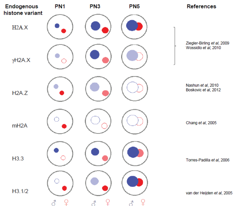
Figure 17. Profiles of endogenous histone variants during zygotic development. Localization and levels of endogenous histone variants obtained by immunostaining experiments in the zygote is shown. PN stands for pronuclear stage, 1 being the earliest after fertilization, 5 the latest. Male (♂) and female (♀) pronuclei are marked in blue and red, respectively. Levels of proteins in each pronucleus are colour-coded, from white (no protein) to dark blue/red (highest protein levels).
