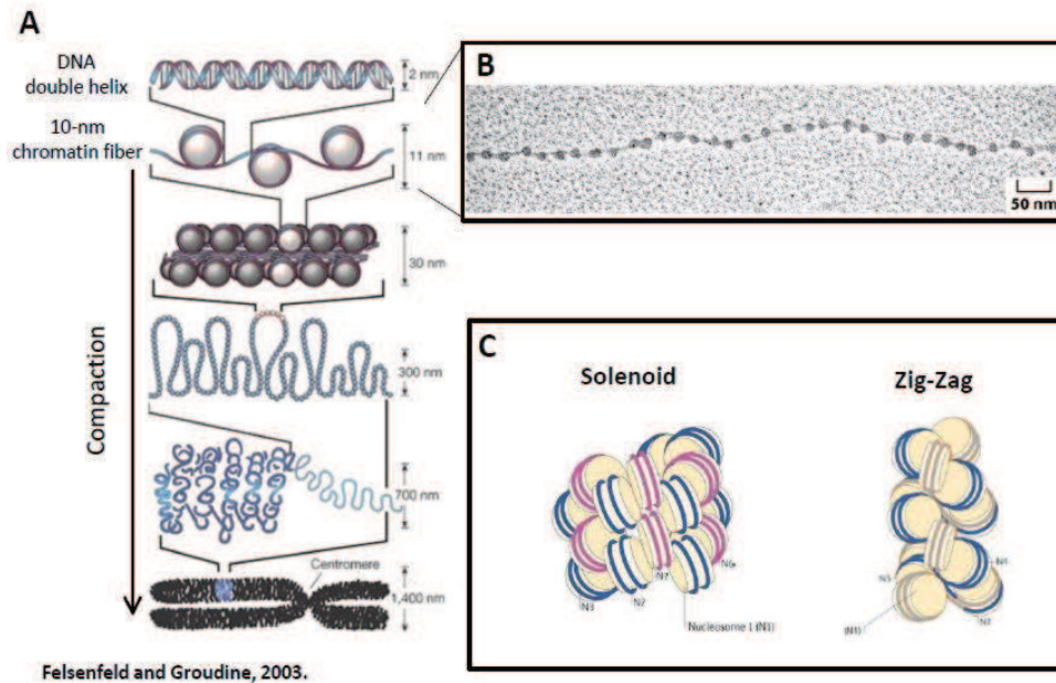
Figure 2. Levels of chromatin compaction. (A) Schematic representation of different levels of chromatin compaction, ranging from the extended 10-nm fiber, to the fully condensed mitotic chromosomes. (B) Electron micrograph of the so-called ‘beads on a string’ 10-nm fiber. From Alberts B et al , 2004. (C) Schematic of 2 proposed models of 30-nm fiber – the one-start solenoid model and the two-start zig-zag model. Adapted from (Luger, Dechassa et al. 2012).
