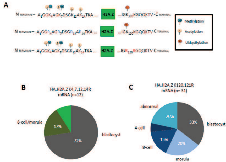
Figure 21. Effects of expression of H2A.Z point mutants on development. (A) Schematic representation of H2A.Z PTMs on N- and C-termini (top panel). Mutating N-terminal lysines 4,7,12 and 14 to arginine impairs H2A.Z acetylation (middle). H2A.Z unubiquitylatable form is obtained by mutating lysines 120 and 121 to arginine (bottom panel). (B) Developmental progression of zygotes injected with mRNA coding for unacetylatable H2A.Z. (C) Developmental progression of zygotes injected with mRNA coding for unubiquitylatable form of H2A.Z. (B and C) Experimental procedures were the same as described in figure 20. Number of injected zygotes is indicated. Development was scored at embryonic day 3.5.
