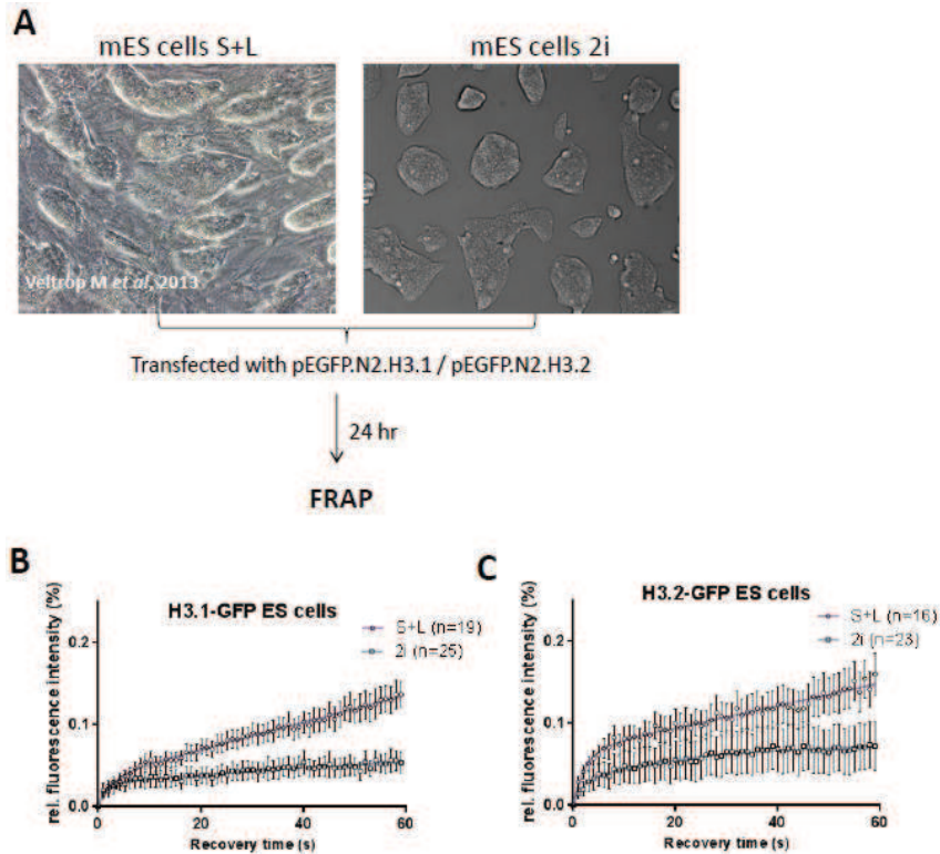
Figure 27. Investigating H3.1-GFP and H3.2-GFP mobility in mouse ES cells grown in different culture conditions. (A) Mouse ES (mES) cells, maintained either in standard (serum + LIF) or 2i (serum + 2 inhibitors) conditions were transfected with plasmids encoding for either H3.1-GFP or H3.2-GFP. FRAP experiments were performed 24 hours after transfection. (B) Recovery curves for H3.1-GFP in two ES cell populations. (C) Recovery curves for H3.2-GFP in two ES cell populations. (B and C) Shown are average values ( \pm SEM) of an indicated number of experiments. Mean recovery values were fit into a two-phase exponential association equation.
