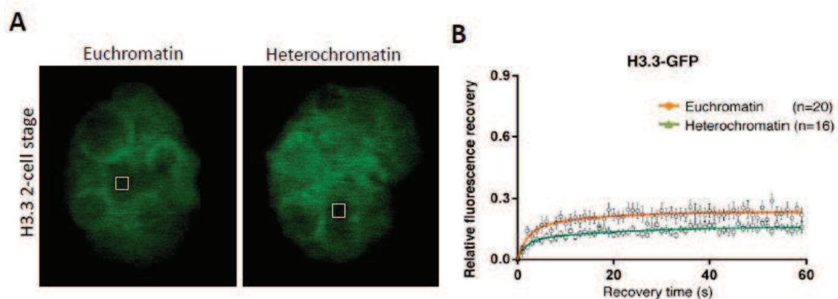
Figure 24. Region-dependent H3.3-GFP mobility at the 2-cell stage. (A) FRAP experiments for H3.3-GFP at the 2-cell stage, investigating small regions of interest (ROI) within the nuclei, to discriminate between mobilities in heterochromatin rings versus nucleoplasm (euchromatin). Mobility of H3.3-GFP was investigated in the ROI of 1 \mu\text{m}^2 . (B) Euchromatic pool of H3.3-GFP is more mobile, and displays slightly higher recovery kinetics, compared to heterochromatic H3.3-GFP. Mobile fraction of H3.3 in euchromatin was 14 \pm 6\% in the fast recovering fraction and 9.4 \pm 5\% in the slow recovering fraction, compared to 9 \pm 2\% (fast) and 7 \pm 1\% (slow) in heterochromatin.
