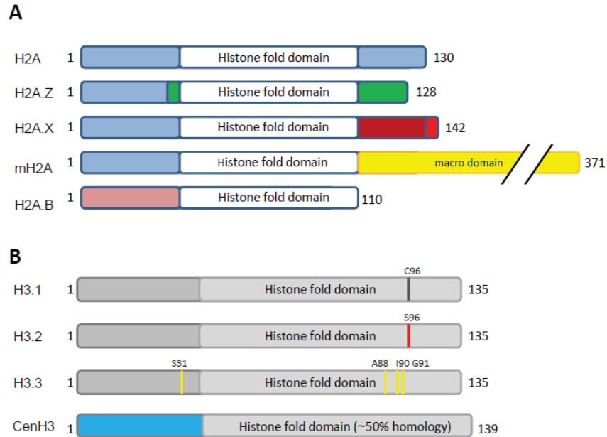
Figure 9. Schematic representation of different H2A and H3 variants. Upper panel (A) shows the 5 most studied somatic H2A variants. Regions of divergence between H2A variants are marked in different color compared to H2A. Lower panel (B) represents the main types of histone H3 variants in mammals. The aminoacids that differ in each of the H3 variants are annotated and numbered.
