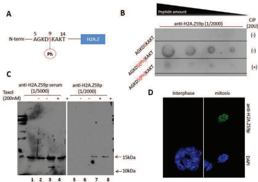
Figure 23. Characterization of anti-H2A.ZS9p antibody. (A) Schematic representation of H2A.Z and the peptide sequence used for antibody production. Serine residue, corresponding to serine 9 in H2A.Z, was phosphorylated in the peptide for antibody production. (B) Dot-blot experiment with non-phosphorylated (AGKDSKAKT) or phosphorylated (AGKDS(Ph)KAKT) peptide, using anti-H2A.ZS9p. Results reveal that antibody is specifically recognizing peptide, and the signal is lost after calf intestine phosphatase (CIP) treatment. (C) Western blot experiment using histone preparation from 3T3 mouse fibroblasts. Samples in lanes 3, 4, 7 and 8 come from cells treated with a cytostatic drug Taxol which blocks mitotic progression at anaphase. Samples in lanes 1, 2, 5 and 6 were obtained from asynchronous cells. Anti-serum against H2A.ZS9p as well as the anti-H2A.ZS9p antibody recognize a band at 15 kDa, and the signal is enriched in mitotic cells. (D) Immunofluorescence using the anti-H2A.ZS9p antibody on asynchronous 3T3 cells revealed a strong enrichment of signal on mitotic chromatin.
