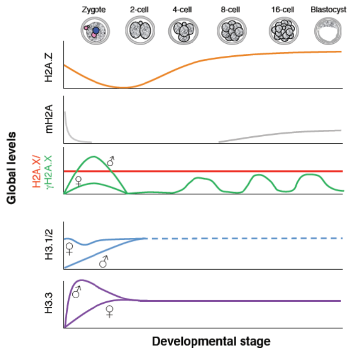
Figure 16. Global changes in the levels of histone variants during murine preimplantation development. The curves depict the schematic representation of global protein levels along development of the indicated histone variants or its modified forms ( \gamma H2A.X) as determined by immunofluorescence. In the zygote, differential accumulation of a histone variant in the female ( \text{♀} ) or the male ( \text{♂} ) pronucleus is illustrated by a double curve. The dotted line for H3.1/H3.2 indicates that their endogenous levels have not yet been determined at later stages.
