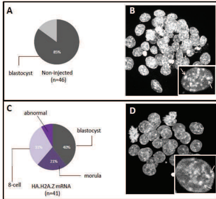
Figure 20. H2A.Z expression in the zygote delays developmental progression. (A) Development of non-injected embryos in culture is shown. 85% of embryos reached blastocyst stage by embryonic day 3.5. Number of embryos investigated is indicated. (B) DAPI-staining of a non-injected blastocyst, mounted onto a coverslip. White insert represents a magnification of a single nucleus of this blastocyst. Chromocenters are indicated by an arrow. (C) Developmental progression of HA.H2A.Z-injected embryos in culture. About 40% of embryos formed blastocysts by E3.5, while a significant proportion of H2A.Z-injected embryos were delayed or arrested at 8-cell and morula stage. (D) DAPI-staining of a H2A.Z-injected blastocyst, mounted onto a coverslip. White insert represents a magnification of a single nucleus of this blastocyst, as above. Nuclei of injected blastocysts contain fewer chromocentres (indicated by an arrow), which are smaller in size and intensity, compared to non-injected nuclei.
