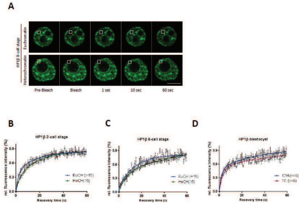
Figure 25. Mobility of HP1 \beta during preimplantation mouse development. (A) Representative FRAP experiments for HP1 \beta at the 8-cell stage. HP1 \beta dynamics were investigated in euchromatin (top panel) and heterochromatin (bottom panel). Bleached regions are shown by a rectangle. Scale bar = 15 \mu m. FRAP curves for HP1 \beta at the 2-cell stage (B) and the 8-cell stage (C) are shown. Green curves correspond to HP1 \beta mobility in heterochromatin and the blue curves to HP1 \beta recovery in euchromatin. (D) HP1 \beta recovery curves in different cell types of the blastocyst. ICM is represented by blue and TE by pink curves.
