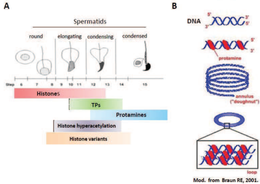
Figure 11. Changes in chromatin composition and genome packaging during spermiogenesis. (A) Sperm genome is packaged mostly by protamines. In elongating spermatids, histones get extensively acetylated and various histone variants become incorporated, leading to the overall destabilization of nucleosomes. Transition proteins (TPs) are expressed during this time and replace most of the histones. TPs are eventually displaced from sperm DNA by protamines. The figure is adapted from (Gaucher, Reynoird et al. 2010). (B) Histone-to-protamine transition in genome packaging ensures high condensation of sperm genome, in the toroidal ring structure, necessary for sperm maturation and fertilization competence.
