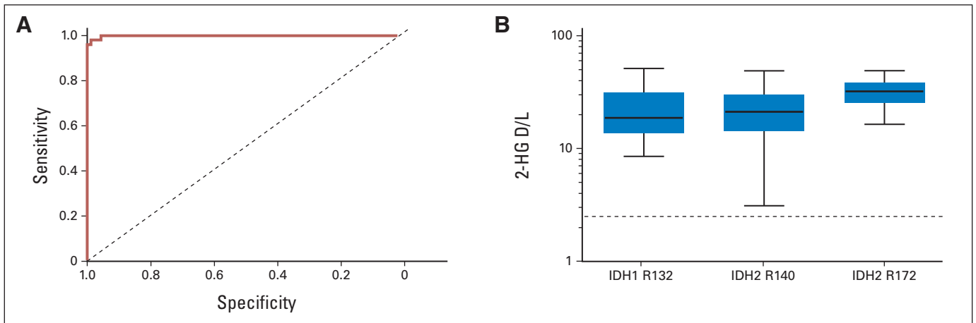
Fig A1. (A) Areas under receiver operator characteristic curve for 2-hydroxyglutarate (2-HG) and D to L ratio for patients with and without acute myeloid leukemia (AML) at diagnosis ( n = 150 ). (B) Comparison of D to L ratio in serum from patients with AML at diagnosis with different mutation sites: IDH1 R132 ( n = 20 ), IDH2 R140 ( n = 24 ), and IDH2 R172 ( n = 9 ).
