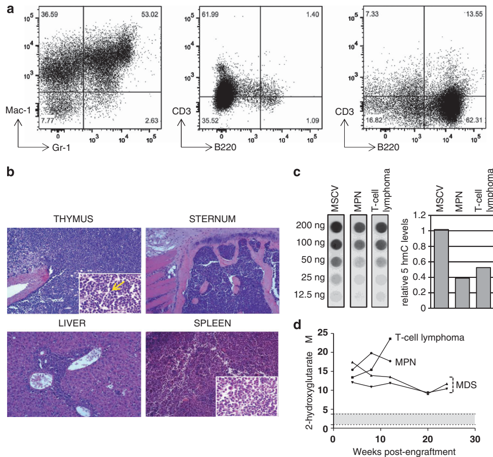
Figure 2. IDH2^{R140Q} promotes the development of hematological proliferations of myeloid or lymphoid origins in mice. (a) Representative FACS profiles of bone marrow cells from IDH2^{R140Q} -engrafted mice suffering from MPN (left panel), T-cell (middle panel) and B-cell (left panel) lymphoma. Live cells were gated using forward and side scatter and further gated on GFP-positivity. (b) Haematoxylin and eosin (H&E)-stained thymus, sternum, liver and spleen from mouse suffering from a T-cell lymphoma. Thymus; diffuse proliferation of malignant T cells with artery involvement ( \times 100 ); lymphoid cells with hyperchromatic nuclei and prominent nucleoli (apoptotic bodies are indicated by an arrow) ( \times 630 ). Sternum; homogeneous invasion of the medullar space by the T-cell proliferation ( \times 100 ). Liver; invasion of the portal space by the same proliferation. Spleen; persistence of a follicular-like structure within the T-cell proliferation ( \times 100 ); coexistence of the proliferation (left) and residual splenic tissue (right) ( \times 630 ). (c) Dot blotting with antibody against 5hmC of non-malignant (spleen; MSCV-engrafted mouse) and malignant cells (spleen; MPN and T-cell lymphoma-affected IDH2^{R140Q} -engrafted mice). Signal intensity of each dot was determined using the ImageJ software ( http://imagej.nih.gov/ij/ ). Histogram shows the relative levels of 5hmC in the three samples. (d) Serum samples from IDH2^{R140Q} -engrafted mice were analyzed for their content in 2-HG over time. The gray, dot-delimited region of the plot defines the normal range of 2-HG serum values (less than 4 \mu\text{mol/l} ) measured in non-leukemic mice. GFP, green fluorescent protein; 2-HG, 2-hydroxyglutarate; 5hmC, 5-hydroxymethyl cytosine; MPN, myeloproliferative neoplasm; MSCV, murine stem cell virus.
