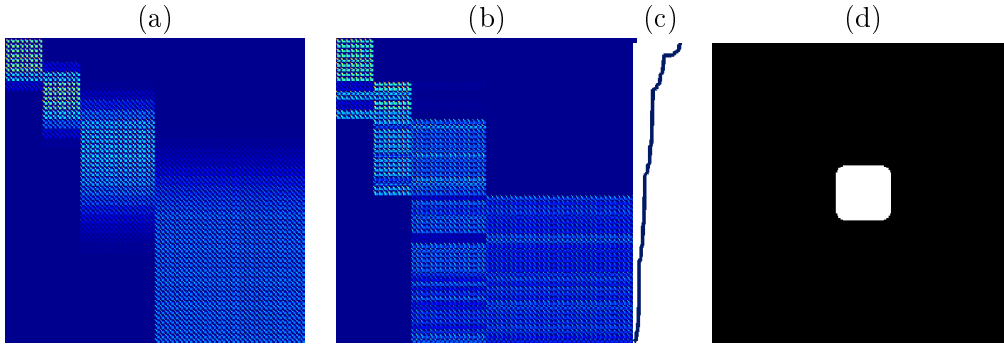
FIGURE 2.3: (a): Absolute magnitudes of \mathbf{A} for a 2D Symmlet basis with 10 vanishing moments and 3 levels of decomposition. (b): same quantities as in (a) but sorted by decaying \|a_i\|_\infty (i.e. by decreasing order). (c): decay of \|a_i\|_\infty . (d): Set \Omega_1 depicted in the 2D k -space.
