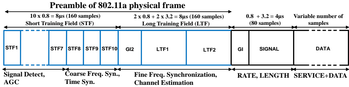
Figure 2.2. Structure of the IEEE 802.11a physical packet
