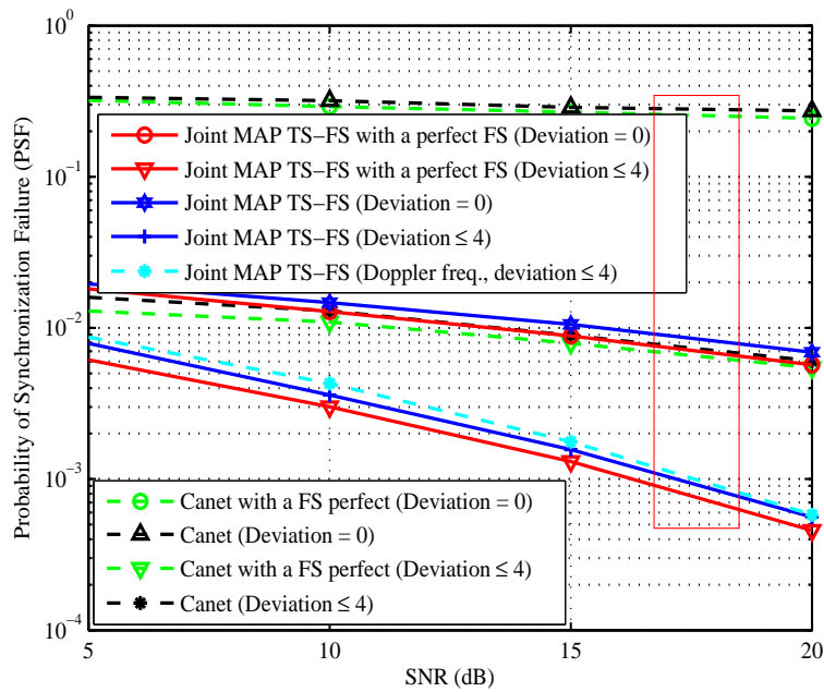
Figure 6.4. PSF of Canet [16] and Joint MAP TS-FS algorithms with |\epsilon| \leq 0.6 under COST207-RA channel model
