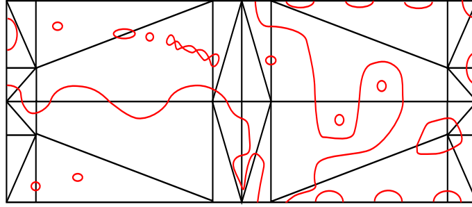
Figure 5.6 – The chart of P
