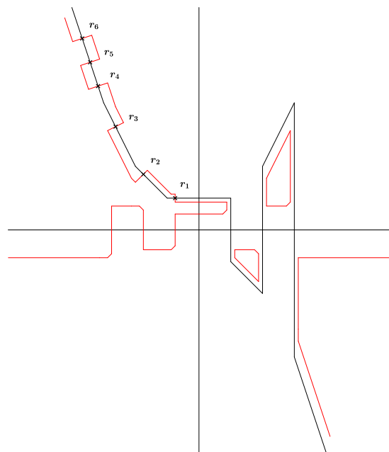
Figure 3.15 – \pi(T_3) \cup \mathbb{R}D_3
