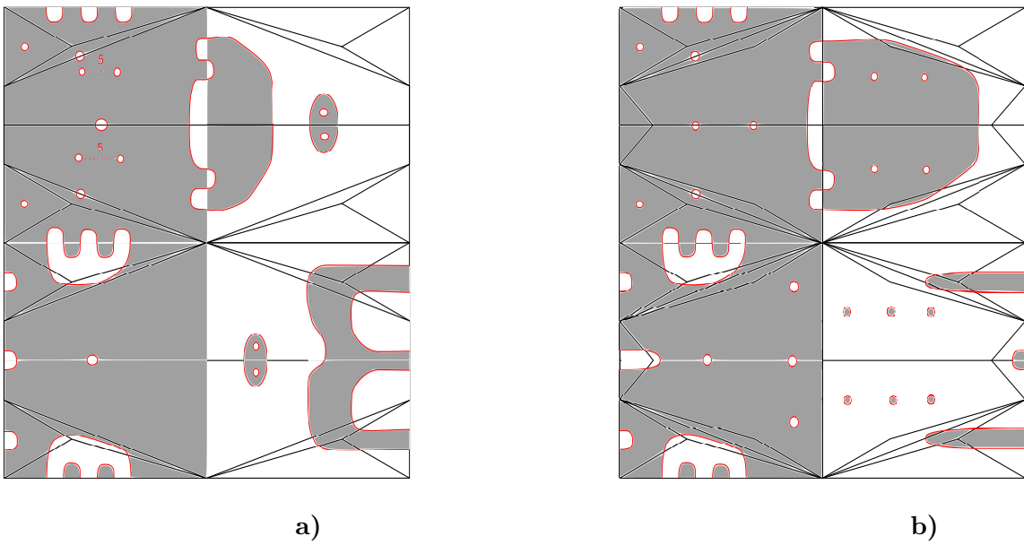
Figure 4.13 – a): (\widehat{A}(x, y)x < 0) b): (A(x, y)x < 0)
