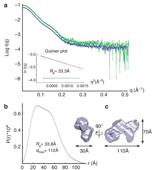
Figure 4 | SAXS analysis (a) PRORP1 and PRORP2 produce very similar intensity curves shown in green and blue, respectively. The inset Guinier plot indicates a gyration radius of 33.3 \pm 0.1 Å. (b) This value is confirmed by the distance distribution function P(r) , which also suggests that PRORP proteins are composed of two distinct domains and an extended tail ( d_{\max} > 100 ). (c) Molecular envelope of PRORP2 derived from SAXS data analysis.
