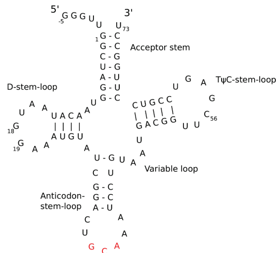
Figure 1.2: Secondary structure of mitochondrial precursor tRNA Cys from A. thaliana including the unpaired 5' leader.
