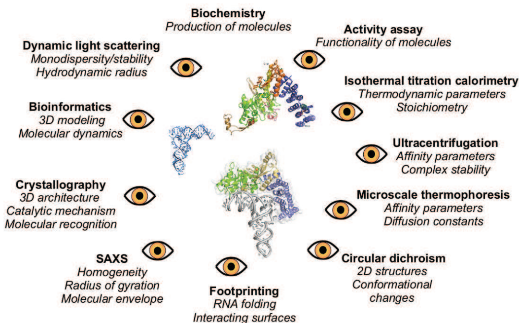
Figure 6.1: Biochemical and biological approaches used and during my thesis and information that could be obtained with each method.
