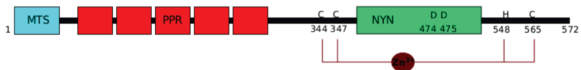
Figure 1.18: Schematic organization of PRORP1 from A. thaliana . MTS - mitochondrial targeting signal, PPR - pentatricopeptide repeat, NYN - Nedd4-BP1, YacP nucleases. A zinc binding motif is structurally connecting the bipartite central domain of PRORP1 which is illustrated by the four zinc chelating residues C344, C347, H548 and C565.
