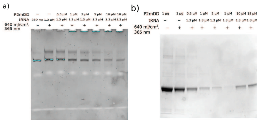
Figure 6.14: Crosslink of PRORP2mDD to L5T0 tRNA Cys at 365 nm, 640 mJ/cm 2 . a) RNA gel, 12 % PAA/8M urea, ethidium bromide staining. Irradiation at 365 nm, 640 mJ/cm 2 , 1.3 μM tRNA and increasing concentration of PRORP2mDD, b) 7.5 % TGX gel, Coomassie staining. Irradiation at 365 nm, 640 mJ/cm 2 , 1.3 μM tRNA and increasing concentration of PRORP2mDD.
