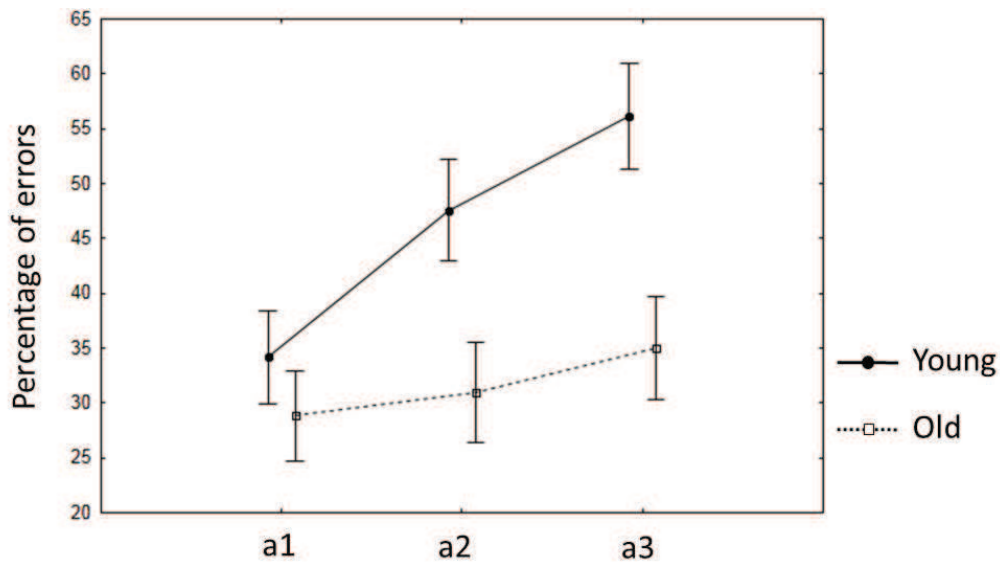
Figure 3. Interaction between age (young/old) and period (a1/a2/a3) on the percentage of errors.
