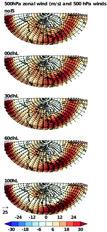
Figure 11: 500 hPa winter wind (arrows) and zonal wind (shaded) in \text{m}\cdot\text{s}^{-1}
