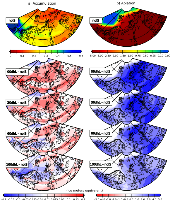
Figure 12: (a) accumulation computed by the ice-sheet model with the noIS experiment outputs, and anomaly of the accumulation between the xdhL experiment and the noIS experiment. (b) same for the ablation.
