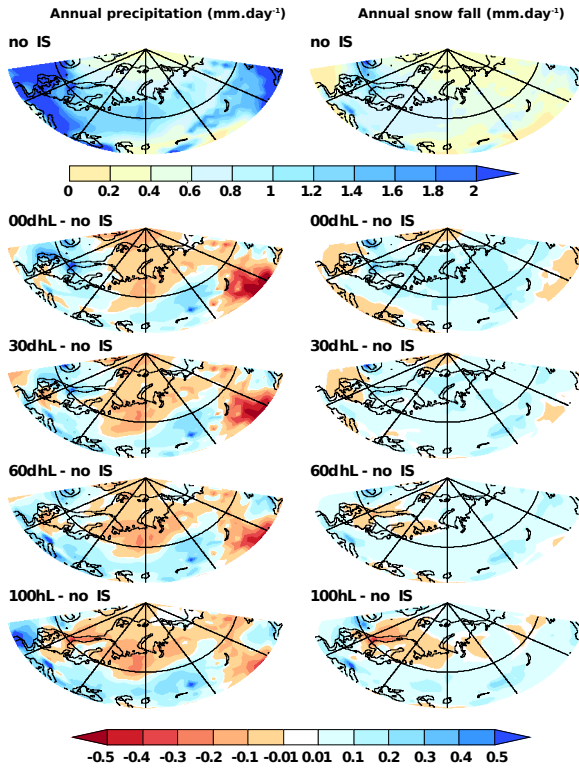
Figure 6: Same as figure 3 for annual precipitation (left column) and annual snowfall (right column)
