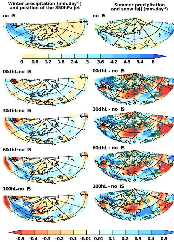
Figure 9: left column : same as figure 3 for winter precipitation (shaded) and position of the Atlantic jet stream without LIS (dashed) and for the corresponding experiment (continuous line). Right column: summer precipitation (shaded) and snowfall (contour every 0.1 mm/day, blue contour for positive values, orange for negative values).
