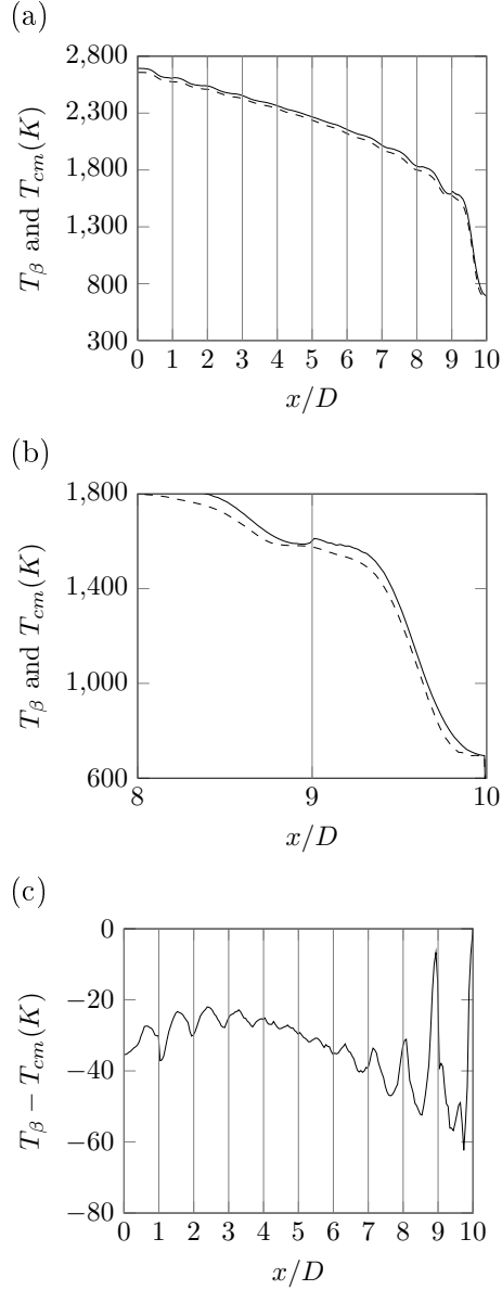
FIGURE 4.14 – (a) Comparison of the temperature profiles from the pragmatical model ( T_\beta , dashed curve) and complete model ( T_{cm} , solid curve) for a scattering and absorbing medium bounded by walls. (b) Zoom on the overheating region; (c) Absolute temperature difference between the pragmatical model ( T_\beta ) and the complete model ( T_{cm} ); \varepsilon_w = 0.8 ; \omega = 0.4 ; \phi_w = 50 \text{ kW m}^{-2} , T_0 = 300 \text{ K} .
