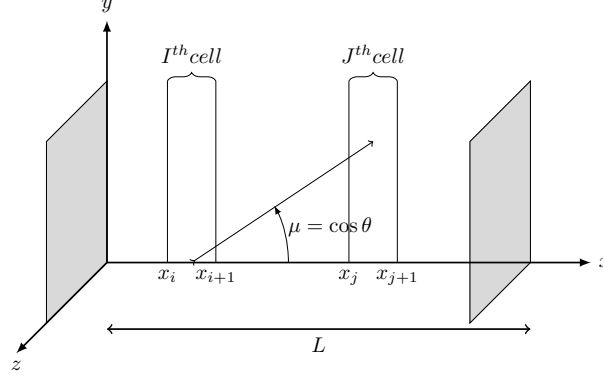
FIGURE 4.2 – 1D slab bounded by two gray opaque walls and divided in N_C cells along the x -axis.
