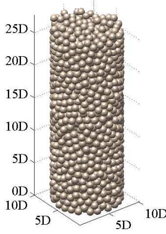
FIGURE 5.1 – Numerically generated packed bed.
