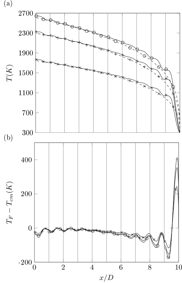
FIGURE 4.9 – (a) Temperature profiles in radiative steady state within a purely absorbing medium bounded by black walls : \varphi_w = 10 \text{ kW m}^{-2} ( \times ), \varphi_w = 30 \text{ kW m}^{-2} ( + ), and \varphi_w = 50 \text{ kW m}^{-2} ( \circ ) ; Results from the complete model T_{cm} (solid lines), and corresponding fitted profiles with an effective radiative conductivity T_F , (dashed lines) ; T_0 = 300 \text{ K} . (b) Residuals of the regression.
