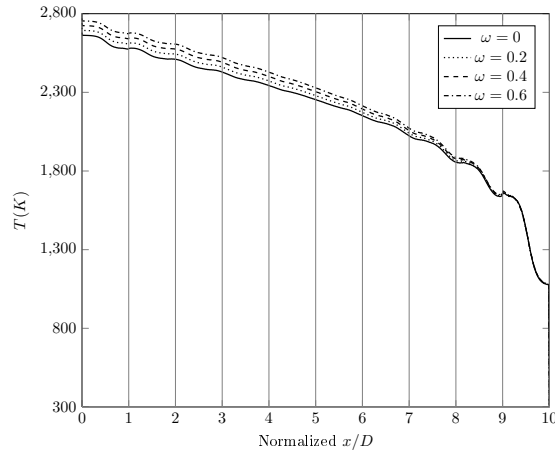
FIGURE 4.12 – Temperature profiles in a scattering and absorbing medium bounded by walls ( \varepsilon_w = 0.4 ) issued from the Monte Carlo approach for \varphi_w = 50kWm^{-2} for various albedo \omega values.
