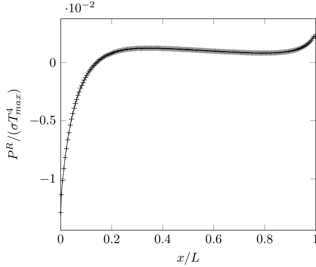
FIGURE 4.3 – Normalised radiative power within a slab of absorbing coefficient \kappa and thickness L ; \kappa L = 10 , \varepsilon_{w1} = \varepsilon_{w2} = 0.6 , \omega = 0 ; Linearly decreasing temperature profile between T(x=0) = T_{max} and T(x=L) = 0.5 T_{max} ; dx = 5 \cdot 10^{-3} L . Calculation from the Monte Carlo approach (+) with \mathcal{N} = 10^6 realizations per cell; analytical (solid line).
