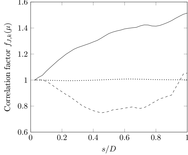
FIGURE 4.8 – Factor of correlation f_{J,k}(\mu) between the cell J in the range [x_{j+1} - dx, x_{j+1}] and the plane k of abscissa x_k = (x_{j+1} + \mu s) with dx = 2.5 \cdot 10^{-2} D ; x_{j+1} = D , \mu = -1 (solid curve); x_{j+1} = D , \mu = -0.5 (dashed curve); x_{j+1} = 5D , \mu = 0.05 (dotted curve).
