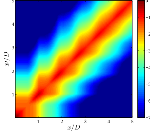
FIGURE 4.5 – \ln[\Pi(x)(1 - G_{ext}(x, \mathbf{u}, x'))] vs x/D and x'/D in the range [0, 5] for the specific directions \mathbf{u} = \pm \mathbf{x} . The upper left and bottom right triangles respectively correspond to \ln[\Pi(x)(1 - G_{ext}(x, \mathbf{x}, x'))] and \ln[\Pi(x')(1 - G_{ext}(x', -\mathbf{x}, x))] .
