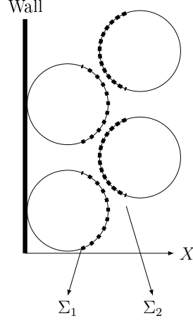
FIGURE 4.10 – Example of particles configuration in the vicinity of a wall.
