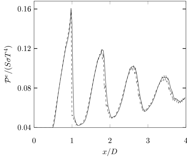
FIGURE 4.7 – Comparison between \mathcal{P}_I^{*e}(\mu)/\sigma T_I^4 given by Eq. 4.31 (solid line) and d\Phi_J^e(\mu=1)/\sigma T_I^4 , given by Eq. 4.12 (dashed line) : dx = 25.10^{-3}D , \omega = 0 , \varepsilon_w = 1 .
