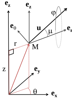
FIGURE 5.2 – Spatial and angular coordinates. The vector \mathbf{u} and angles (\mu, \varphi) are defined in the rotating frame (M, \mathbf{e}_r, \mathbf{e}_\theta, \mathbf{e}_z) .
