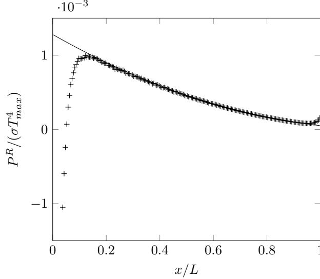
FIGURE 4.4 – Normalised radiative power within a slab of absorbing coefficient \kappa and thickness L ; \kappa L = 40 , \varepsilon_{w1} = \varepsilon_{w2} = 0.8 , \omega = 0.2 ; Linearly decreasing temperature profile between T(x=0) = T_{max} and T(x=L) = 0.2 T_{max} ; dx = 5.10^{-3}L . Calculation from the Monte Carlo approach (+) with N = 5.10^6 realizations per cell; Fourier law (solid line)
