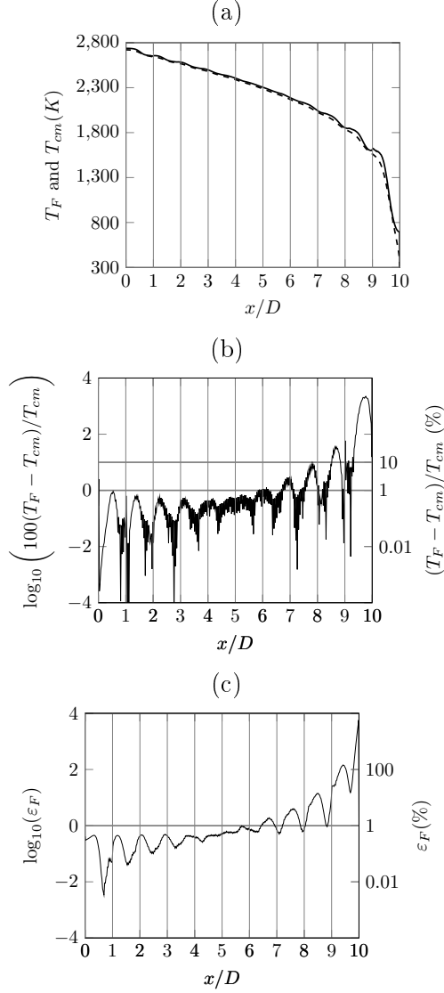
FIGURE 4.13 – (a) Comparison of the temperature profiles issued from a Fourier law ( T_F , dashed curve) and Monte Carlo calculations ( T_{cm} , solid curve) in a scattering and absorbing medium bounded by grey walls. (b) Logarithm of the relative discrepancy on the temperatures (c) Logarithm of the validity criterion of the Fourier law \log(\varepsilon_F) . The Fourier law is valid with a precision of (T_F - T_{cm})/T_{cm} < 1\% if \varepsilon_F < 1 . \varepsilon_w = 0.8 ; \omega = 0.4 ; \varphi_w = 50 \text{ kW m}^{-2} , T_0 = 300 \text{ K} .
