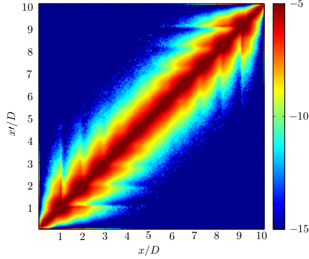
FIGURE 4.6 – Typical example of \ln(\mathcal{P}_{IJ}^{ea}) normalized matrix; \mathcal{N} = 5.10^5 realizations per cell; N_C = 200 , L = 10D , \omega = 0 and \varepsilon_w = 1 .
