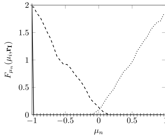
FIGURE 4.11 – Distribution of the normal for x_i = 0, \mu_i = 1 ( ++ ); x_i = 0, \mu_i = 0.5 (solid line); x_i = 5D, \mu_i = 1 (dashed line); x_i = 5D, \mu_i = -1 (dotted line).
