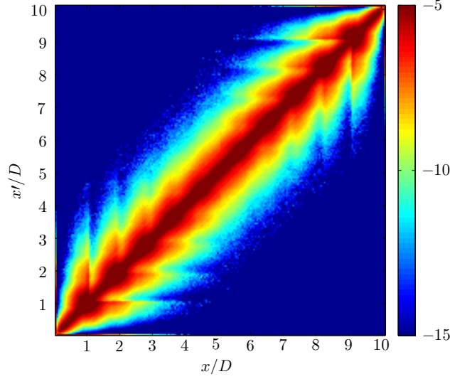
FIGURE 4.6 – Typical example of \ln(\mathcal{P}_{IJ}^{e,a}) normalized matrix; \mathcal{N} = 5.10^5 realizations per cell; N_C = 200 , L = 10D , \omega = 0 and \varepsilon_w = 1 .
