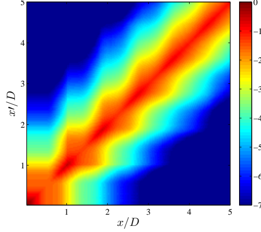
FIGURE 4.5 – \ln[\Pi(x)(1 - G_{ext}(x, \mathbf{u}, x'))] vs x/D and x'/D in the range [0,5] for the specific directions \mathbf{u} = \pm \mathbf{x} . The upper left and bottom right triangles respectively correspond to \ln[\Pi(x)(1 - G_{ext}(x, \mathbf{x}, x'))] and \ln[\Pi(x')(1 - G_{ext}(x', -\mathbf{x}, x))] .
