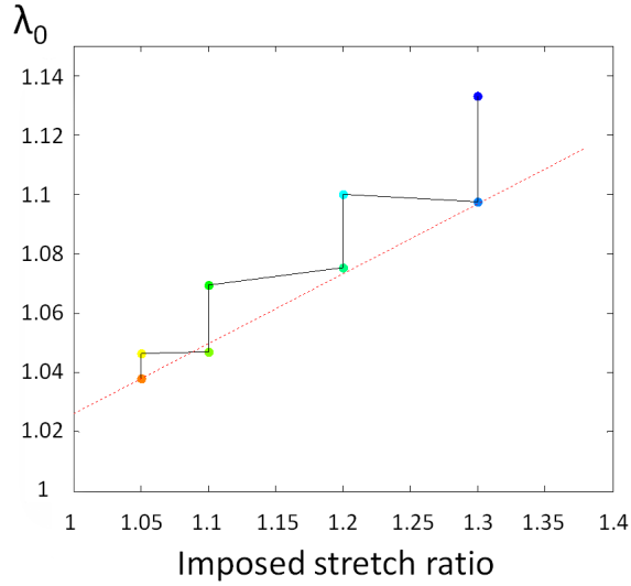
Figure III.15 – Stretch ratio for which the force first exceeded the sensor’s noise level, versus maximum imposed stretch ratio, for the same sample as in figure III.14.
