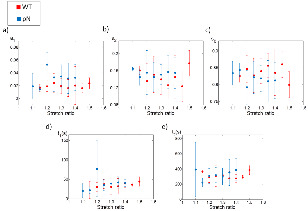
Figure IV.18 – Averaged values of the five parameters describing the relaxation behaviour of pN mice compared to WT mice: a) amplitude of short time relaxation a_1 , b) amplitude of long time relaxation a_2 , c) amplitude of the relative constant s_0 , d) short time t_1 (s) and e) long time t_2 (s). Error bars represent the standard error of the mean.
