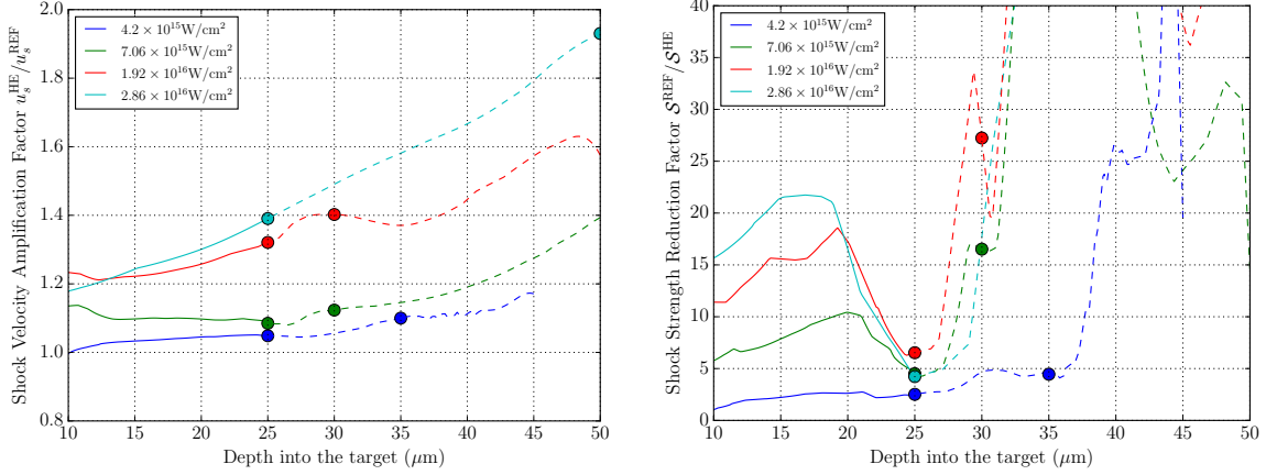
Figure 6-15 – Modification of the shock parameters due to the presence of LPI-generated HEs. [left] Shock velocity amplification factor u_s^{\text{HE}}/u_s^{\text{REF}} and [right] shock strength reduction factor \mathcal{S}^{\text{REF}}/\mathcal{S}^{\text{HE}} , as a function of the shock depth into the target, for all targets and intensities. Plain lines and dashed lines indicate the approximate regions where the shock is in the CH and in the tracers, respectively. The colored circles indicate the approximate location of the CH/tracer or tracer/tracer interfaces.
