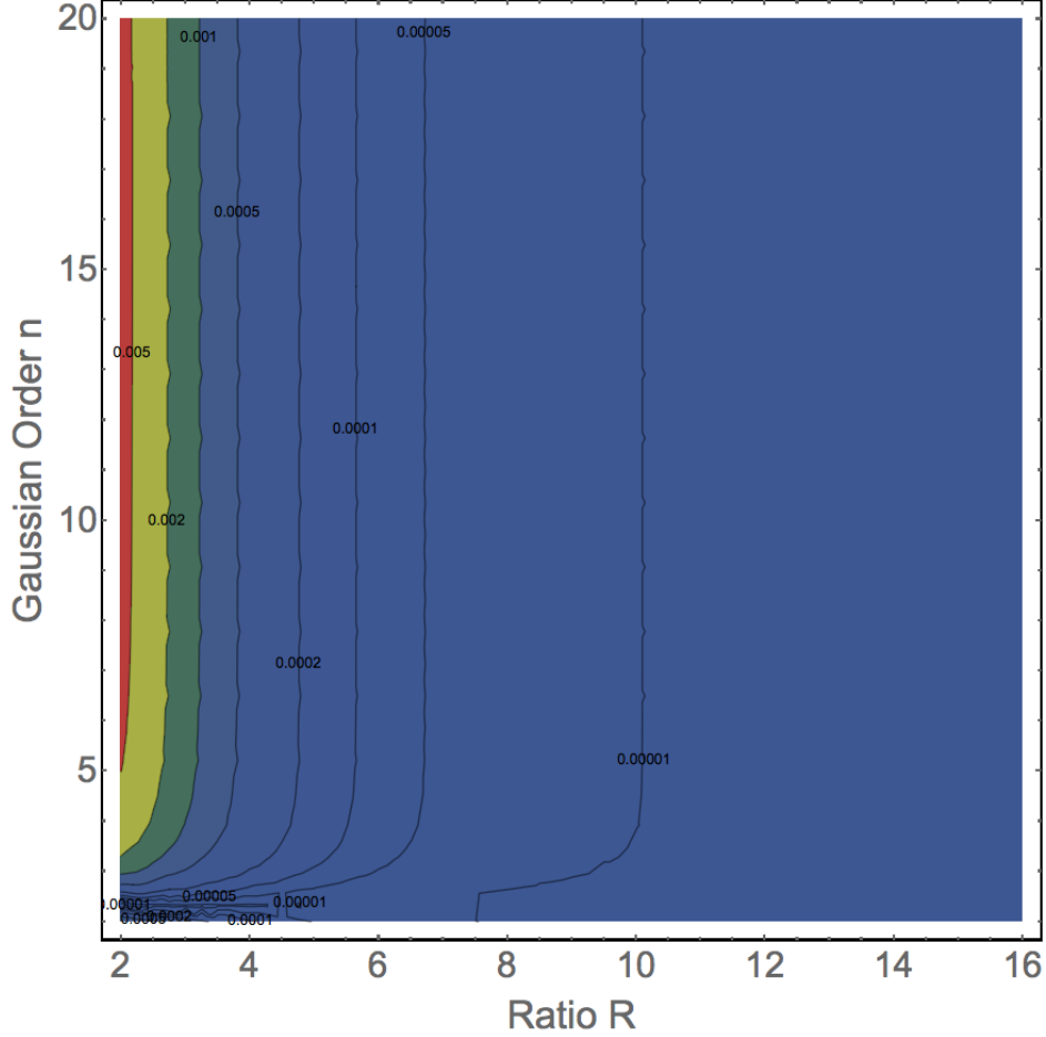
Figure B-1 – Mean Squared Error as a function of the super-Gaussian order n , and ratio \mathcal{R} , for N = 3\hat{\mathcal{R}} beamlets. Red indicates higher MSE and blue lower MSE.
