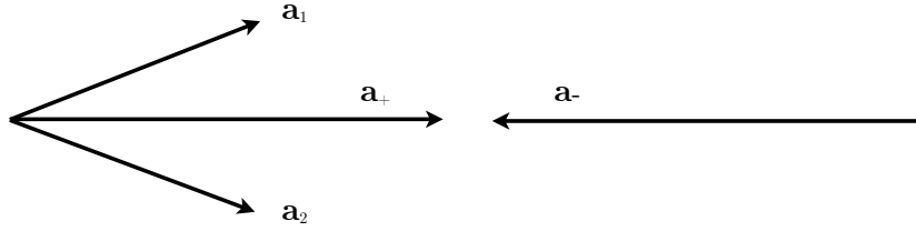
Figure 4-7 – Illustration of the EM waves described in HARMONY. The code is formulated for the propagation and interaction of counter-propagating waves a_- and a_+ . In our case, the a_- component is set to 0, and the a_+ term is decomposed in two co-propagating waves.
