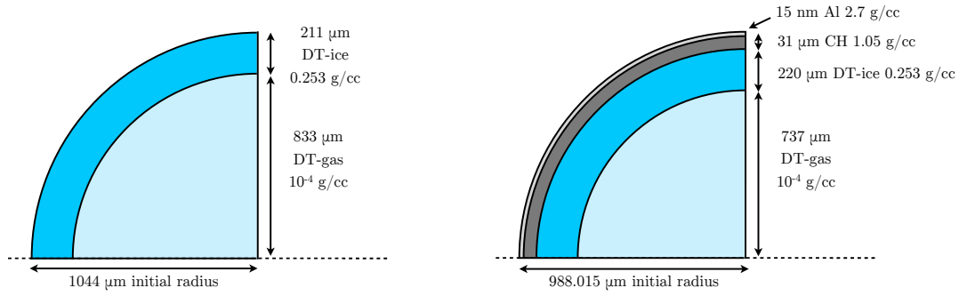
Figure 6-20 – Schematic of the two targets considered in the study. [left] Pure-DT target from the baseline HiPER project. [right] SI target recently designed at CELIA, with high yield and high safety margins with respect to the hydrodynamic instabilities.
