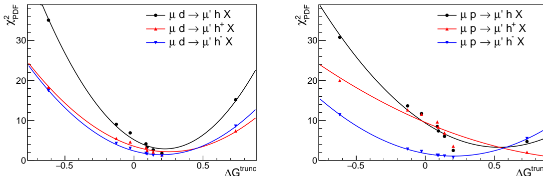
Figure 5.14: Illustration of \chi^2 minimisation to extract \Delta G_{data}^{trunc} based on DSS14 FFs set
