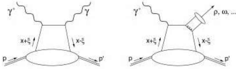
Figure 1.3: Feynman diagram for DVCS (left) and DVMP (right) processes
