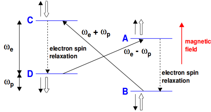
Figure 2.4: The four energy levels defined by the sin projections of an electron-nucleus system (electron spin with a single arrow and nucleon spin with a wide arrow)
