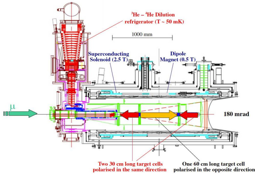
Figure 2.6: COMPASS polarised target for 2006-2007 and 2011
