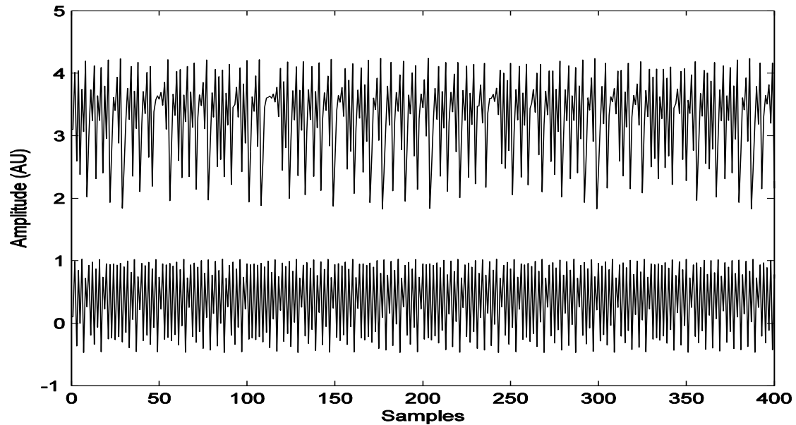
Figure 2.1: Simulated signal generated by using the Henon model with different complexity degrees ( CD ). Top: CD = 0.1 , Bottom: CD = 0.9 .
