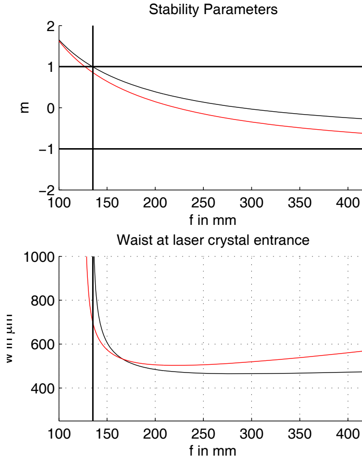
Figure 5.11: The stability diagram (upper panel, see Equation (5.14)) and the mode sizes (lower panel) in the laser crystal as a function of the thermal lens focal length f_{th} . The black (red) lines denote the horizontal (vertical) direction. The vertical line indicates the limit of cavity stability. The resonator remains stable down to f_{th,min} = 135 \text{ mm} .
