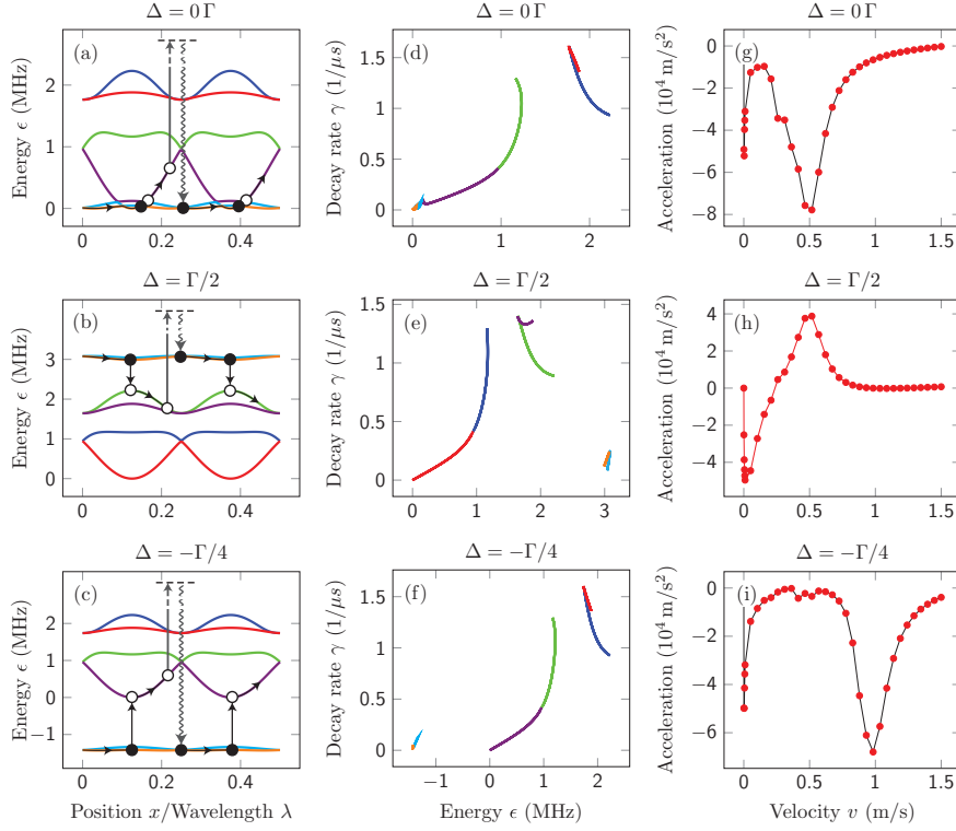
FIG. 6. (Color online) Cooling mechanism around the Raman condition in a simplified model. Optical Bloch equation simulation for ^6\text{Li} subjected to a 1D bichromatic lattice with linear orthogonal polarizations near D_1 resonance. The cooling lattice and repumping lattice are displaced by \pi ( \lambda/4 ). I_{\text{cool}} = 15I_{\text{sat}} , I_{\text{rep}} = 0.75I_{\text{sat}} , \delta_{\text{cool}} = 4\Gamma . (a–c) Dressed states as functions of the position, in units of the D_1 optical wavelength. The two dressed F = 1/2 levels (light blue and orange) are nearly flat in all the graphs due to the small I_{\text{rep}} . (d–f) Decay rate of dressed states as a function of their energy shifts. Here the two dressed F = 1/2 levels span a very small energy range and have a low decay rate. (g–i) Velocity-dependent optical force for an atom dragged at velocity v . (a, d, g) \Delta = 0 ; (b, e, h) \Delta = \Gamma/2 ; (c, f, i) \Delta = -\Gamma/4 . Note the negative sign of the force in (g) and (i), implying cooling, and the anticooling force for velocities near 0.5 m/s in (h).
