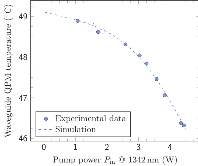
Fig. 5. (Color online) Optimal crystal mount temperature T_{\text{mount,opt}} during SHG process in dependence of the fundamental IR pump power P_\omega coupled to the waveguide. The crystal mount temperature is adjusted for every pump power value in order to maximize the corresponding SH power.
