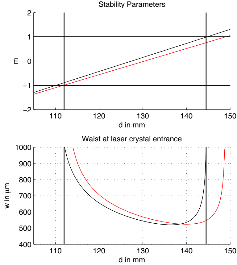
Figure 5.12: (Upper Panel) The stability parameters of the laser cavity as a function of the distance d_{cu} between the curved mirrors M_3 and M_4 . The thermal focal length is fixed to 170 mm. (Lower Panel) The mode sizes in the laser crystal w_{h(v)} , the black (red) lines denoting the horizontal (vertical) direction, whereas the vertical lines indicate the range of stability.
