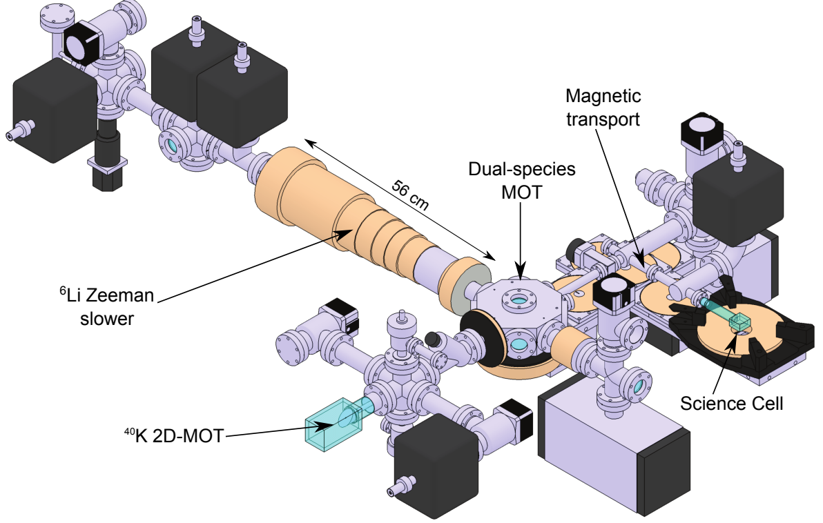
Figure 2.1: 3D-CAD model of the vacuum assembly. A Zeeman slower for ^6\text{Li} and a 2D-MOT for ^{40}\text{K} serve as atom sources for the dual-species MOT contained in the octagonal MOT-chamber. A magnetic transport transfers the cloud to the glass science cell featuring improved vacuum quality and large mechanical and optical access.
