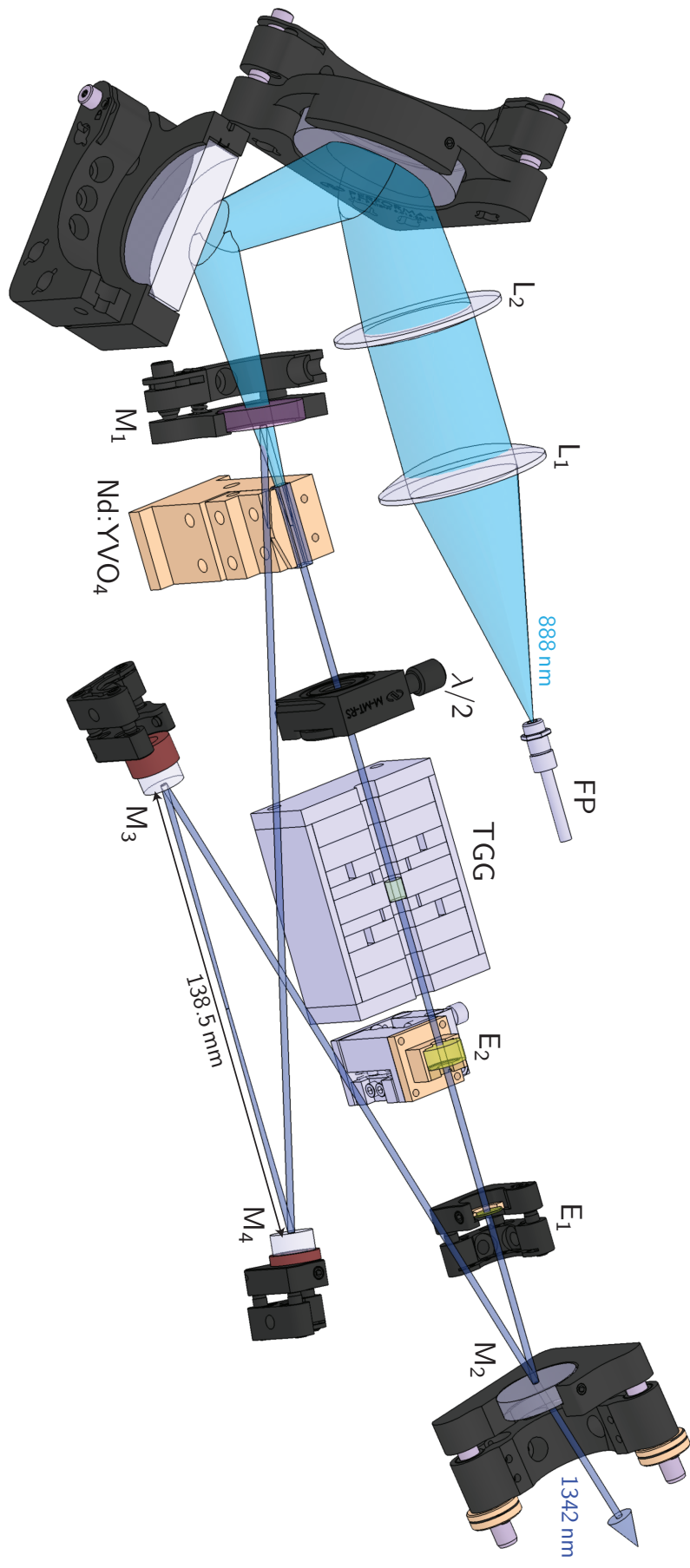
Figure 5.1. – Setup of the 1342 nm laser source from [140]. Two lenses, L_1 and L_2 , image the output of the pump source, a fiber-coupled diode laser bar (FP) emitting at 888 nm, into the \text{Nd:YVO}_4 gain medium. The ring resonator consists of four mirrors M_{1-4} in bow-tie configuration, which are all highly reflective at 1342 nm except M_2 serving as partly transmitting output coupling mirror. A Faraday rotator (TGG) in combination with a half-wave plate ( \lambda/2 ) enforces unidirectional operation. Insertion of two etalons E_{1-2} allows for single-longitudinal-mode behavior and wavelength tunability. For a technical drawing of the cavity setup see Figure 5.10.
