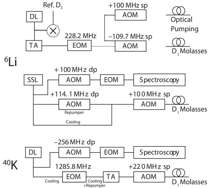
Figure 2.6: Laser systems of the D_1 molasses cooling schemes for ^6\text{Li} and ^{40}\text{K} . The frequencies and amplitudes of the various beams are controlled by AOMs in single pass (sp) or double pass (dp) configuration. EOMs creates the repumping frequency in the ^{40}\text{K} setup and in the diode laser (DL) ^6\text{Li} setup. The EOMs in the spectroscopy phase modulate a sample of the beam for the frequency-lock of the lasers. Single mode polarization maintaining fibers transmit the beams to the main experimental table. The indicated AOM frequencies correspond to the beam frequencies required for the molasses cooling, see Figure 2.5.
