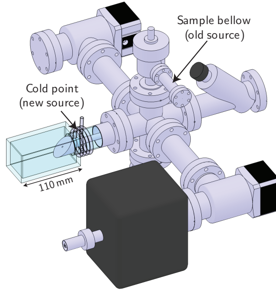
Figure 2.9: The ^{40}\text{K} 2D-MOT vacuum assembly. The cold point serves as new potassium source, since the bellows originally containing the sample became depleted. The old source region is heated to \sim 120^\circ\text{C} , the glass cell to \sim 80^\circ\text{C} and all intermediate parts to at least 100^\circ\text{C} to establish a temperature gradient. The cold point water temperature can be regulated by means of a chiller in order to control the 2D-MOT pressure, see Figure 2.10.
