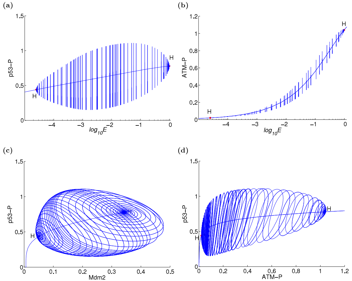
Figure 3.7. (a) Bifurcation diagram for the nuclear p53-P and (b) for the nuclear ATM-P with respect to increasing E ; E is in the logarithmic scale. Bars plotted on figures (a) and (b) are the heights (showing maximum and minimum) of the amplitudes of stable limit cycles. (c) p53-P vs. Mdm2 limit cycles occurring for values of the damage signal E between the two Hopf bifurcation points. (d) The same in the p53-P vs. ATM-P phase plane. The equilibrium curves in (c) and (d) are the curves joining the two Hopf bifurcation points H, constituting stable, then unstable, and then stable equilibrium branch again, with the stable limit cycles surrounding the unstable equilibrium points. The plotted concentrations are dimensionless.
