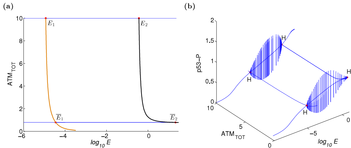
Figure 3.11. (a) The evolution curves of both Hopf bifurcation points (curves in brown and black colours). The plotted Hopf points E_1 and E_2 are computed for ATM_{TOT} = 10 \mu M , the Hopf points \bar{E}_1 and \bar{E}_2 are computed for ATM_{TOT} = 0.78 \mu M . E is in the logarithmic scale. (b) Bifurcation diagram of p53-P with respect to changing ATM_{TOT} and E .
