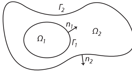
Figure 4.1. Cell scheme: the nucleus \Omega_1 , the cytoplasm \Omega_2 , the nuclear membrane \Gamma_1 and the cell membrane \Gamma_2 ; n_1 and n_2 are the unit normal vectors oriented outward from \Omega_1 and \Omega_2 , respectively.
