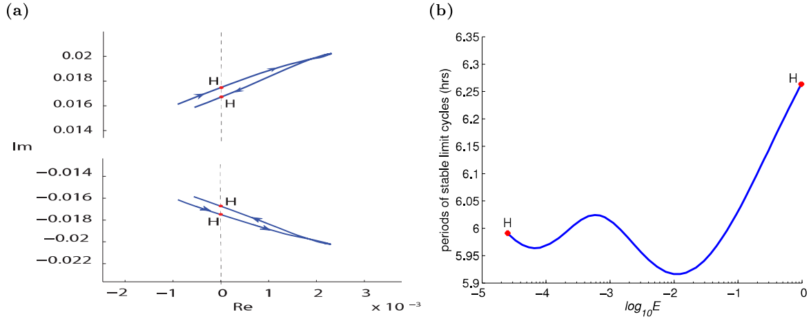
Figure 3.6. (a) A pair of eigenvalues crossing the imaginary axis for E = 2.5 \times 10^{-5} and E = 0.97 , revealing thus the existence of two Hopf bifurcation points. (b) Evolution of the period of stable limit cycles maintaining between the two Hopf bifurcation points; E is in the logarithmic scale.
