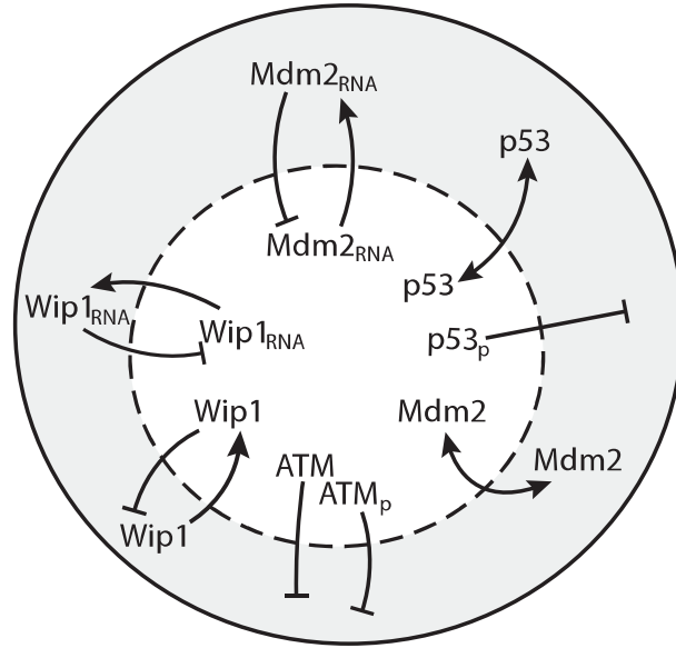
Figure 3.1. Assumptions on the localisation and exchange of the considered proteins between the nucleus and the cytoplasm made in our model. mRNA variables are denoted on this figure by the additional subscript RNA , and similarly the subscript p denotes a phosphorylated protein. The proteins p53 and Mdm2 are assumed to migrate freely (i.e., without diffusion limitations, resulting in homogeneous concentrations) within each of the two compartments. T-shaped lines mean impossible transport in the T-end direction.
