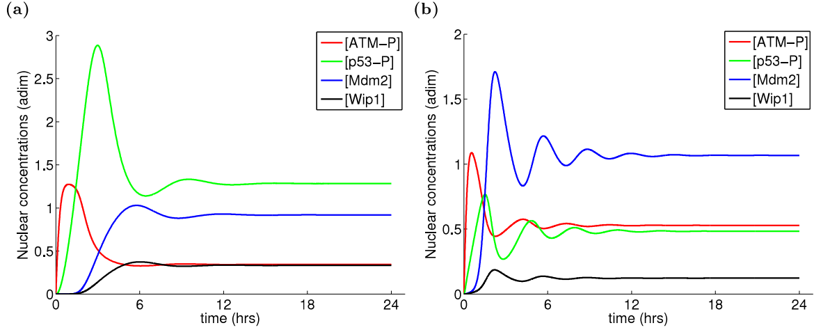
Figure 3.10. (a) Nuclear ATM, p53, Mdm2 and Wip1 (adim) concentrations over a 24 hour-long time interval, E = 0.1 \mu M , in the case when Mdm2-mediated ubiquitination of p53 is inhibited, k_{ub} = 0 . (b) Nuclear ATM, p53, Mdm2 and Wip1 (adim) concentrations over a 24 hour-long time interval and E = 0.1 \mu M in the case when only one compartment is considered.
