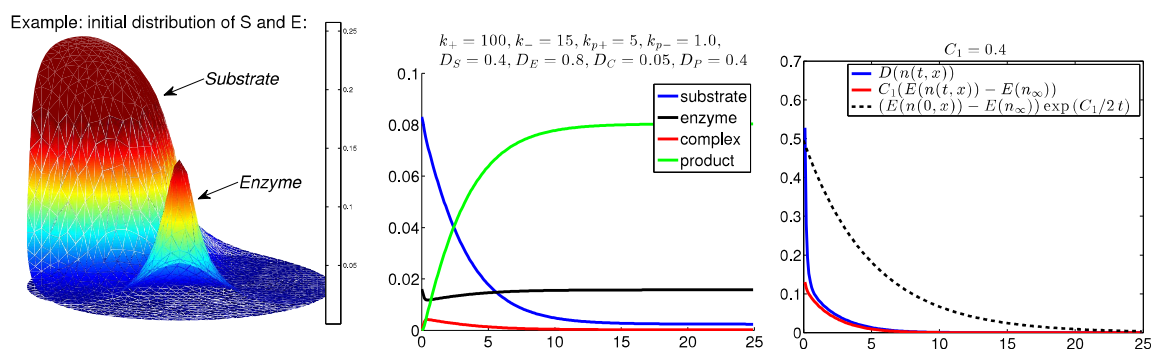
Figure 8.4. An example of 2D FreeFem++ simulation of the reversible enzyme reaction, see also the following section. On the left: initial distribution of the substrate S and the enzyme E . In the middle: evolution of the total concentrations ( \int_{\Omega} n_i , i \in \{S, E, C, P\} ) of the species appearing in the enzyme reaction. On the right: entropy dissipation, relative entropy and an exponential bound appearing in (8.48) and (8.51). The dimensionless parameters are chosen as follows: reaction rates k_+ = 100 , k_- = 15 , k_{p+} = 5 , k_{p-} = 1 , diffusions D_S = 0.4 , D_E = 0.8 , D_C = 0.05 , D_P = 0.4 .
