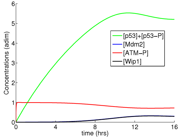
Figure 5.13. Solution of the 2D PDE system following DNA damage producing the transiting signal E = 1 in the case when both compartments are merged together. The plotted concentrations are the total concentrations in the nucleus.
