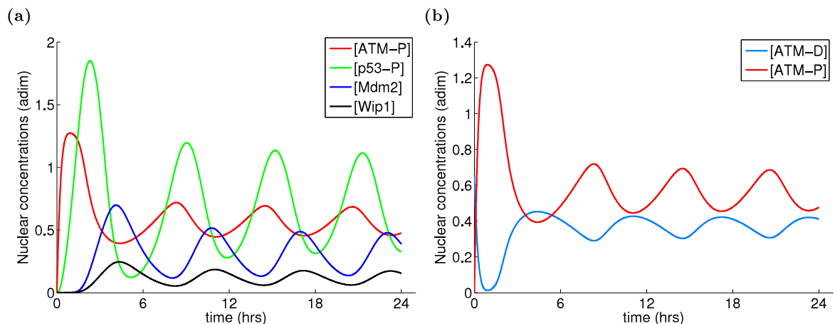
Figure 3.2. (a) Nuclear ATM, p53, Mdm2 and Wip1 (adim) concentrations over a 24 hour-long time interval. (b) Evolution of the ATM monomerisation and dimerisation with the total concentration of ATM, ATM_{TOT} = 1.3 \mu M , and E = 0.1 \mu M (where E is a hypothetical damage signalling molecule launching ATM activation).
