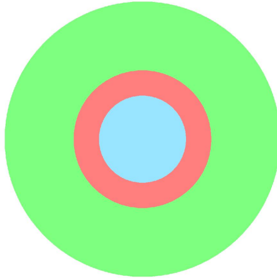
Figure 4.3. 2D cell used in simulations of the Leloup–Goldbeter PDE model. The cell is represented by the nucleus (central zone, blue) and the cytoplasm constituted of the endoplasmic reticulum (perinucleic annulus, red) where no translation is allowed and the translation zones (peripheral, green) denoted by \chi_{tra} in (4.5). The nucleus, thus shown as an inner disc, has radius \sqrt{10} \mu m in this case. The endoplasmic reticulum is an annulus with radii \sqrt{10} \mu m and 5 \mu m . The rest of the cytoplasm is an annulus with radii 5 \mu m and 10 \mu m .
