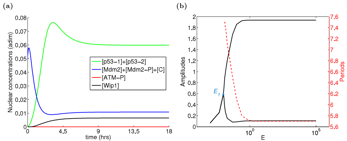
Figure 6.8. (a) Solution of the RD PDE system (6.3)-(6.4) modelling p53 dynamics with a dual function of Mdm2 toward p53 in normal conditions ( E = 0 ); (b) Bifurcation diagram for the nuclear p53 concentration (p53-1 and p53-2) with respect to the varying signal E (plotted in the logarithmic scale). The bifurcation point E_1 is the point on the black curve where the curve bifurcates into two paths. The curve for E < E_1 shows attained steady states and plotted two curves for E > E_1 are the heights (showing maximum and minimum) of the amplitudes of stable limit cycles. The red curve shows periods of oscillations depending on E . The plotted nondimensionalised concentrations are the total concentrations in the nucleus. The used parameters are in Tables 6.2 and 5.2.
