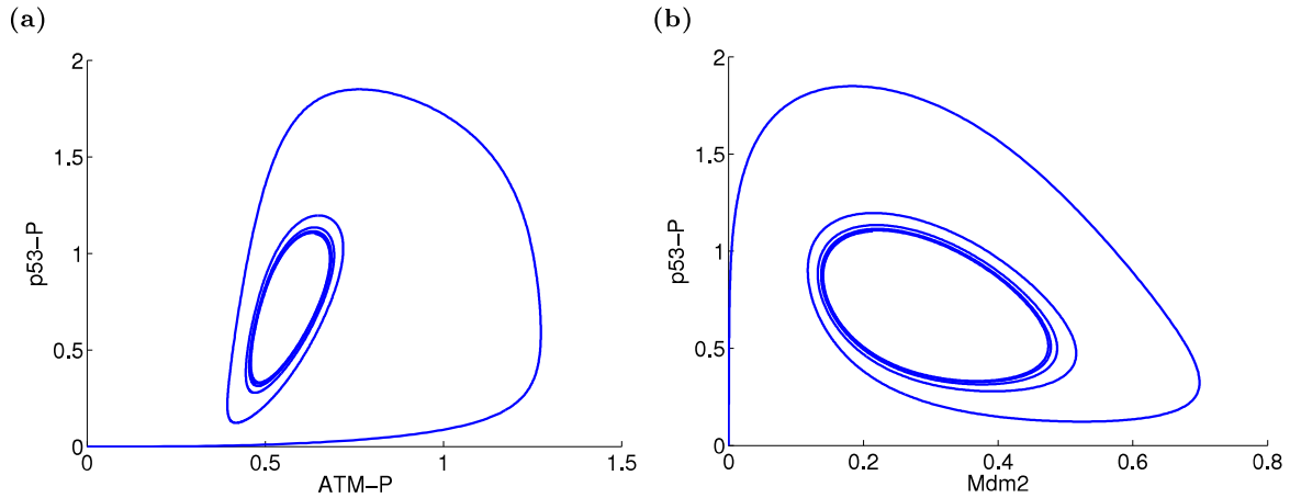
Figure 3.3. Phase plane curves relative to the involved nuclear proteins with E = 0.1 \mu M (where E is a hypothetical damage signalling molecule launching ATM activation): (a) ATM-P and p53-P (b) Mdm2 and p53-P.
