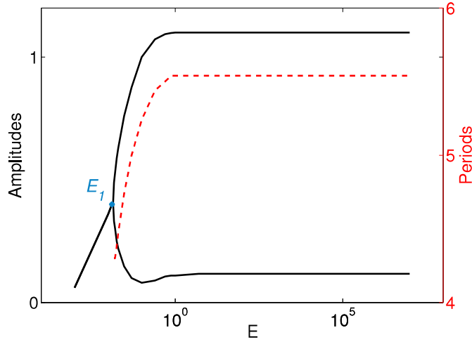
Figure 5.11. Bifurcation diagram for nuclear p53 (p53 and p53-P) with respect to the varying signal E in the 2D PDE system with the parameters in Tables 5.5 and 5.2; E is plotted in the logarithmic scale. The bifurcation point E_1 is the point on the black curve where the curve bifurcates into two paths. The curve for E < E_1 shows attained steady states and plotted two curves for E > E_1 are the heights (showing maximum and minimum) of the amplitudes of stable limit cycles. The red curve shows periods of oscillations depending on E .
