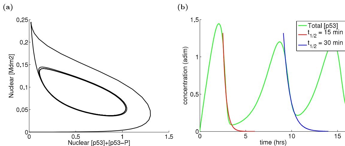
Figure 5.7. Solution of the 2D PDE system for the fixed set of parameters in Tables 5.5 and 5.2: (a) phase portrait of dimensionless nuclear concentrations of p53 (p53 and p53-P) with respect to Mdm2; (b) decay of the total (nuclear and cytoplasmic) p53 concentration in the cell with wt Mdm2 corresponds to the half-life of 15 and 30 minutes, respectively, in the first and the second pulse.
