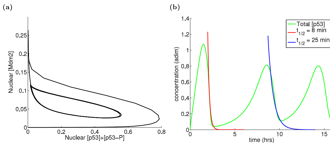
Figure 5.8. Solution of the 3D PDE system for the fixed set of parameters in Tables 5.5 and 5.2: (a) phase portrait of dimensionless nuclear concentrations of p53 (p53 and p53-P) with respect to Mdm2; (b) decay of the total (nuclear and cytoplasmic) p53 concentration in the cell with wt Mdm2 corresponds to the half-life of 8 and 25 minutes, respectively, in the first and the second pulse.
