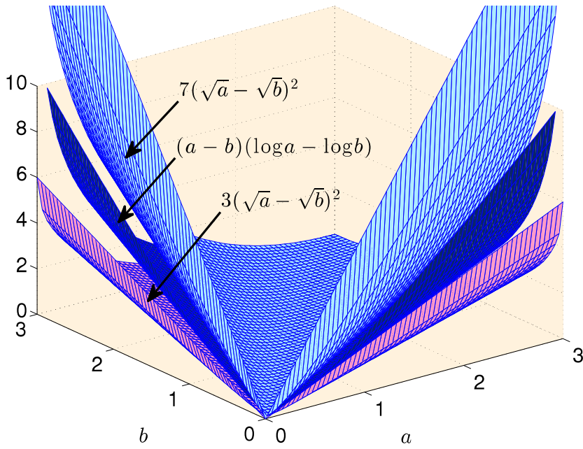
Figure 8.2. Plots of the three function appearing in the inequality L_1(\sqrt{a} - \sqrt{b})^2 \leq (a - b)(\log a - \log b) \leq L_2(\sqrt{a} - \sqrt{b})^2 for L_1 = 3 and L_2 = 7 for the clarity of the picture. The inequality is actually true for better rates, e.g., for L_1 = 4 and L_2 = 5 (the picture would not be very clear for these constants).
