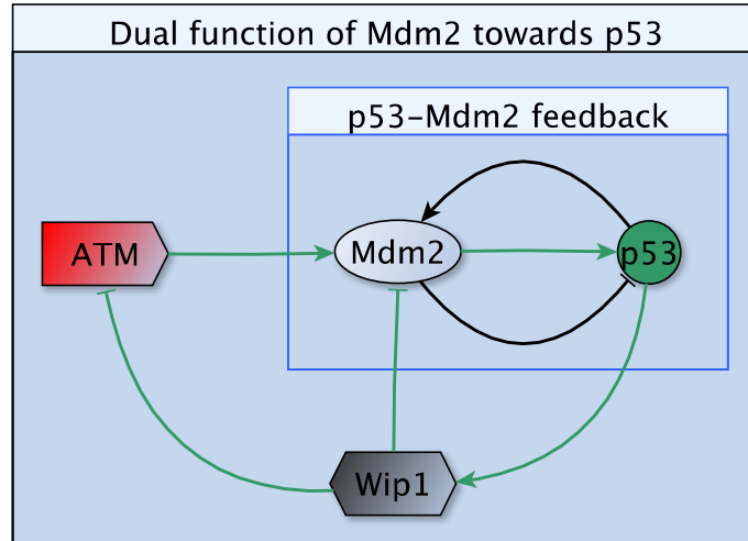
Figure 6.12. The model for the dual function of Mdm2 towards p53 relies on the two negative feedback loop: the classical p53 \rightarrow Mdm2 \dashv p53 where p53 transcriptionally induces Mdm2 and Mdm2 in turn degrades p53, and the loop between ATM and Wip1 through the cascade involving p53 and Mdm2, i.e. ATM-P \rightarrow Mdm2 \rightarrow p53 \rightarrow Wip1 \dashv ATM-P , where Mdm2, after being phosphorylated by ATM, enhances synthesis of p53 which in turn transcriptionally activates Wip1 (and also Mdm2) which inactivates ATM.
