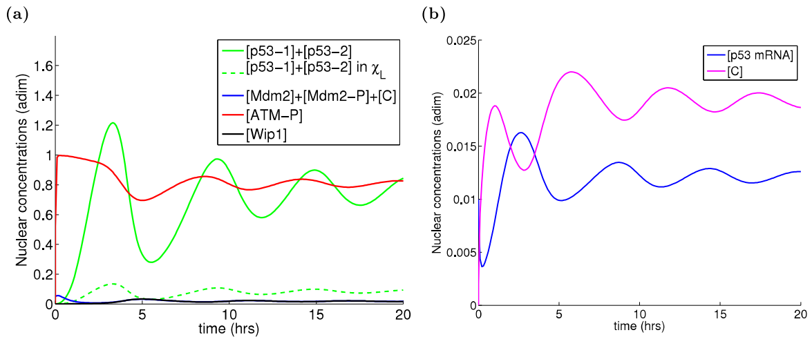
Figure 6.7. Solution of the RD PDE system (6.3)-(6.4) modelling p53 dynamics with a dual function of Mdm2 toward p53. Plotted curves are the concentrations in 20 hrs of DDR in response to the stress signal E = 1 for the decreased translation rate for p53-2 so that k_{tp-1} = k_{tp-2} = 1 , other fixed parameters in Tables 6.2 and 5.2: nondimensionalised (a) nuclear concentrations of total p53 (p53-1 and p53-2), total Mdm2 (Mdm2, free Mdm2-P and Mdm2-P bound to C ), ATM-P and Wip1; green dashed line shows the concentration of p53 in the DNA locus \chi_L (that is the transcriptionally active p53); (b) total cellular “free” p53 mRNA and p53 mRNA bound to the complex C . The plotted concentrations are the total concentrations in the nucleus and cytoplasm, respectively.
