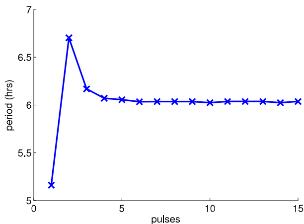
Figure 3.5. The periods of the fifteen p53-P pulses produced by the ODE model within E = 0.1 \mu M . The length of the first pulse is 5.16 hours, the p53-P stable limit cycle is of the period \sim 6 hours.
