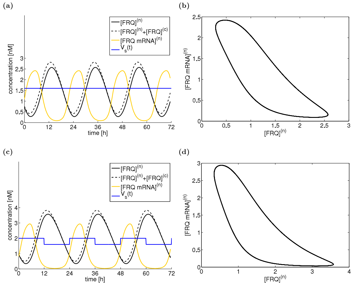
Figure 4.2. The concentrations of the nuclear FRQ, its mRNA, and the sum of the nuclear and cytoplasmic FRQ in (a) continuous darkness, V_s = 1.6 \text{ nM h}^{-1} , and in (c) 12:12 light:dark cycle, V_s = 2 \text{ nM h}^{-1} and 1.6 \text{ nM h}^{-1} every 12 hours. Concentrations are solutions to the PDE model (4.5) with the Kedem–Katchalsky BC (4.7) and (4.8). Received period in (a) is 21.5 hours, in (c) 23.5 hours. Subplots in (b) and (d) show stable limit cycles of the concentrations. The parameters used in the PDE model (4.5) are in Table 4.1. The plotted concentrations are scaled over the total volume of the computational domain (nucleus or cytoplasm).
