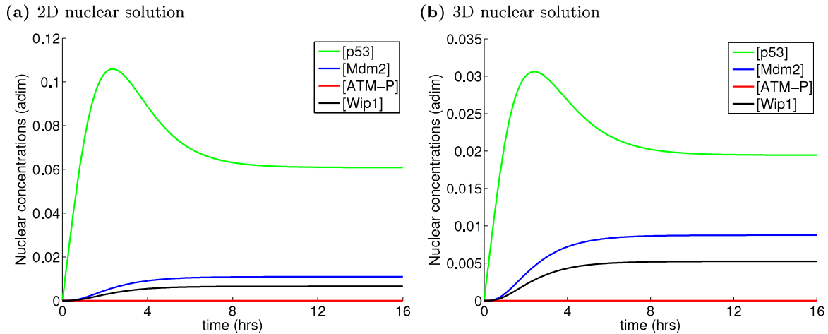
Figure 5.5. Solution of the PDE system within 16 hrs under normal conditions, E = 0 , for the fixed set of parameters in Tables 5.5 and 5.2: nondimensionalised nuclear (a) 2D, (b) 3D concentrations. The plotted concentrations are the total concentrations in the nucleus and cytoplasm, respectively. Without any ATM-P in the system, there is obviously no p53-P produced, thus unphosphorylated p53 is plotted only.
