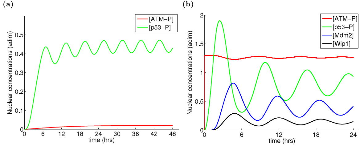
Figure 3.8. (a) Nuclear p53-P and ATM-P (adim) concentrations from the ODE system for E = E_1 = 2.5 \times 10^{-5} \mu M . The concentration of ATM-P converges to the equilibrium point (which is equal to 0.02) and the concentration of p53-P tends to a stable limit cycle. (b) Nuclear ATM-P, p53-P, Mdm2 and Wip1 (adim) concentrations for E = 10 \mu M . The oscillations of ATM-P are of small amplitude, getting even smaller with further increasing E ; ATM_{TOT} = 1.3 \mu M .
