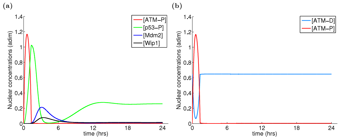
Figure 3.9. (a) Nuclear ATM, p53, Mdm2 and Wip1 (adim) concentrations over a 24 hour-long time interval following ATM inhibition after one full pulse. (b) Evolution of the ATM monomerisation and dimerisation with the total concentration of ATM, ATM_{TOT} = 1.3 \mu M , and E = 0.1 \mu M , following ATM inhibition after one full pulse.
