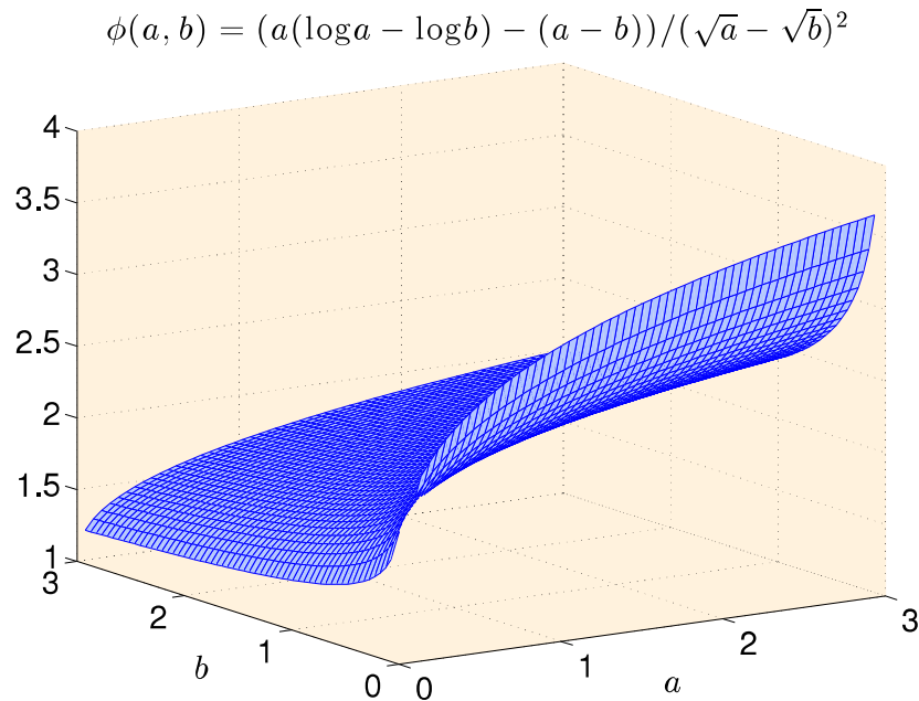
Figure 8.1. Graph of the function \Phi(a, b) for a, b \in [0, 3] .
