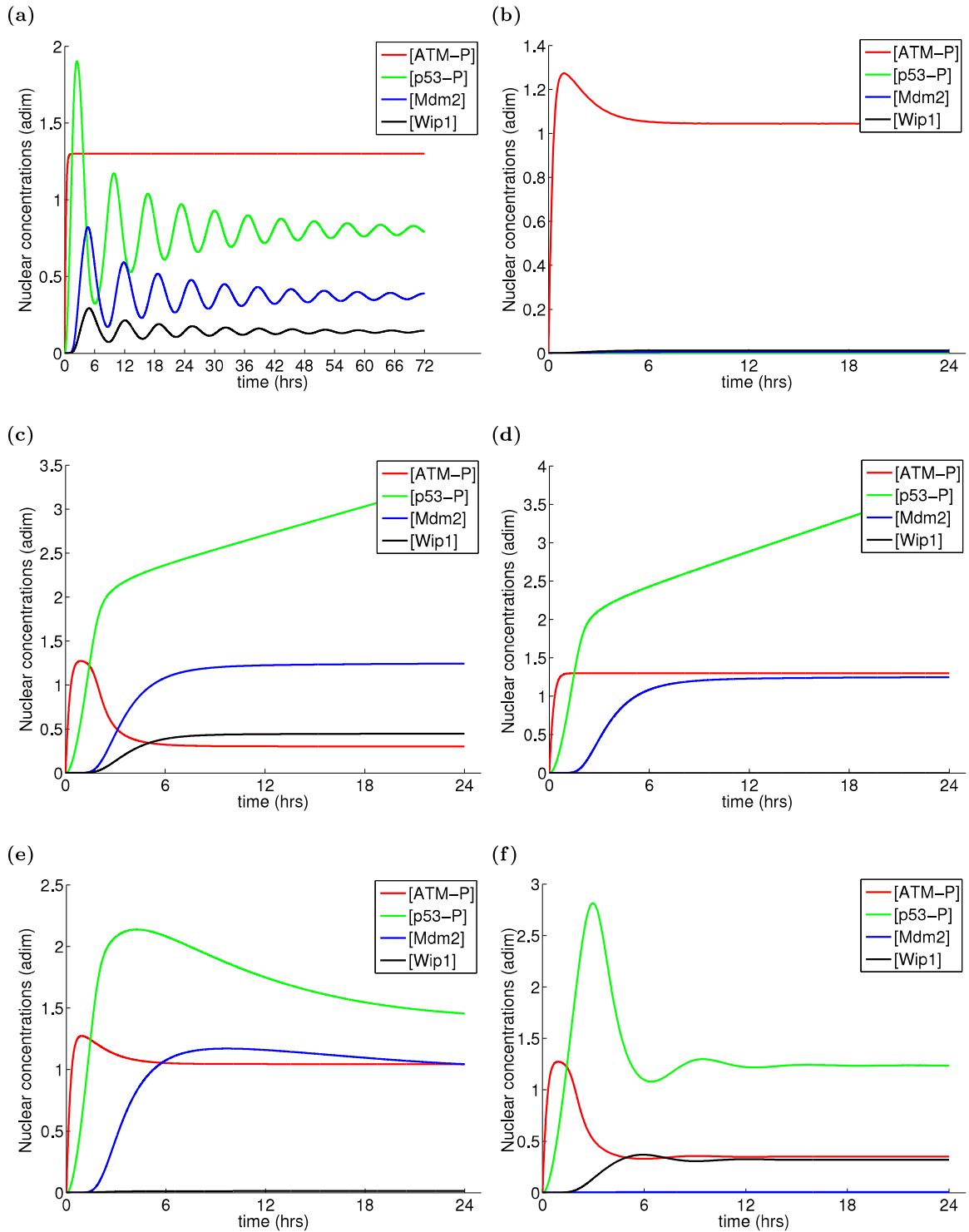
Figure 3.12. Nuclear ATM, p53, Mdm2 and Wip1 (adim) concentrations in the case of (a) inhibition of the negative feedback Wip1 \dashv ATM , k_{dph2} = 0 in (3.4); (b) inhibition of the positive feedback ATM \rightarrow p53 , k_{ph1} = 0 in (3.14); (c) inhibition of the negative feedback Wip1 \dashv p53-P , k_{dph1} = 0 in (3.14); (d) inhibition of the positive feedback p53-P \rightarrow Wip1 , k_{Spw} = 0 and k_{Sw} = 0 ; (e) inhibition of the positive feedback p53-P \rightarrow Wip1 , k_{Spw} = 0 and k_{Sw} = 0.03 ; and (f) inhibition of the positive feedback p53-P \rightarrow Mdm2 , k_{Spm} = 0 and k_{Sm} = 0.005 .
