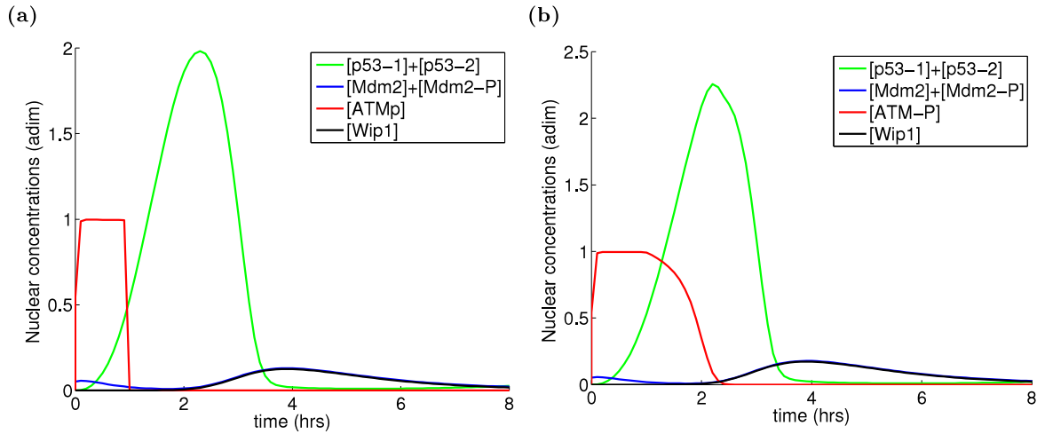
Figure 6.10. Solution of the RD PDE system (6.3)-(6.4) modelling p53 dynamics with the dual function of Mdm2 toward p53 when (a) ATM-P signalling is inhibited 1 hour after damage and (b) the damage-transmitting signal E is inhibited after one hour. The plotted nondimensionalised concentrations are the total concentrations in the nucleus.
