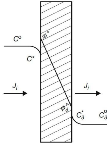
Figure 2.3. Passive transport throughout the nuclear membrane: initial concentrations C^0 and C_\delta^0 of a specie in two compartments divided by a membrane of the thickness \delta . Due to interaction of the species with the membrane, the actual concentrations outside of the both sides of the membrane are C^* and C_\delta^* and inside of the membrane \phi^* and \phi_\delta^* . These values are generally different and satisfy \phi^* = HC^* and \phi_\delta^* = HC_\delta^* where H is a characteristic parameter dependent on interaction of the species with the membrane. For the flux J , Fick's first law then implies J = -D \frac{d\phi}{dy} \approx -D \frac{\phi_\delta^* - \phi^*}{\delta} = -\frac{DH}{\delta} (C_\delta^0 - C^0) , where D is a diffusion rate of a transported substrate through the membrane and the difference of concentrations C_\delta^0 - C^0 is the driving force for the exchange of the substrate. The coefficient p = DH/\delta is the permeability rate (measured in \mu m/s ) and it is the property of membrane. For more details see [112], p. 8–9. Figure taken from [112], copyright by Elsevier.
