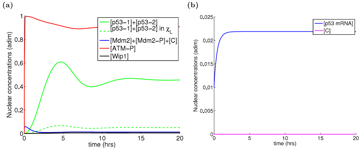
Figure 6.6. Solution of the RD PDE system (6.3)-(6.4) modelling p53 dynamics with a dual function of Mdm2 toward p53. Plotted curves are the concentrations in 20 hrs of DDR in response to the stress signal E = 1 in the case when no complex C formation is allowed (i.e., k_a = 0 ) for the parameters in Tables 6.2 and 5.2: nondimensionalised (a) nuclear concentrations of total p53-1 (no p53-2 is produced), total Mdm2 (Mdm2 and Mdm2-P), ATM-P and Wip1; green dashed line shows the concentration of p53 in the DNA locus \chi_L (that is the transcriptionally active p53); (b) total cellular “free” p53 mRNA and p53 mRNA bound to the complex C . The plotted concentrations are the total concentrations in the nucleus and cytoplasm, respectively.
