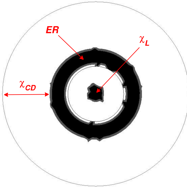
Figure 6.3. A scheme of the cell used in the model: the cell is represented by a disc with radius 10\ \mu m . It consists of the nucleus represented by an inner disc of radius 3\ \mu m and the cytoplasm containing the rest of the cell. Within the cytoplasm there is an endoplasmic reticulum (ER) where no translation of the mRNAs occurs. The ER is represented by an annulus with radii 3\ \mu m and 5\ \mu m . Translation of the mRNAs is supposed to occur outside of the ER, thus in an annulus \chi_{CD} with radii 5 and 10\ \mu m . Inside the nucleus there is a small disc \chi_L of radius 1\ \mu m which represents the DNA locus where production of all mRNA content occurs.
