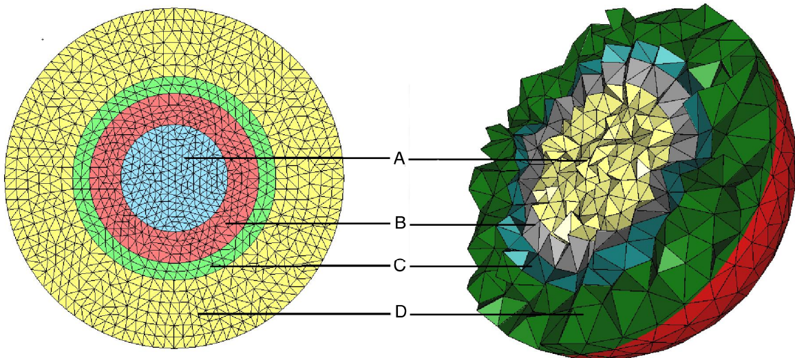
Figure 5.4. The 2D and 3D cell is represented by a disc and by a 3D ball, respectively, with radius 10 \mu\text{m} . The nucleus, A, is shown as an inner disc and an inner ball, respectively, with radius 3 \mu\text{m} . The endoplasmic reticulum B, where no production of the proteins occurs, is an annulus with radii 3 \mu\text{m} and 5 \mu\text{m} ; the ring-shaped area C, where the basal production of p53 is assumed to occur, is an annulus with radii 5 and 6 \mu\text{m} , respectively, and the rest of the cytoplasm, D, is an annulus with radii 6 and 10 \mu\text{m} . Translation of the mRNAs is supposed to occur in C+D. The 2D and 3D cell triangulations are generated by FreeFem++ , [62].
