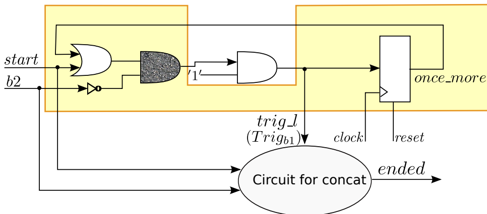
FIGURE 6.19: Implementation of b1[*]; b2
