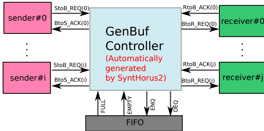
FIGURE 4.2: GenBuf circuit interface
