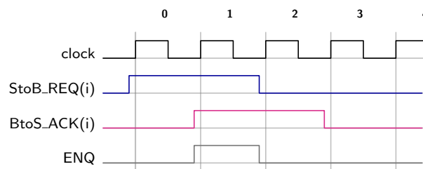
FIGURE 4.4: An example timeline of a GenBuf to sender handshake
