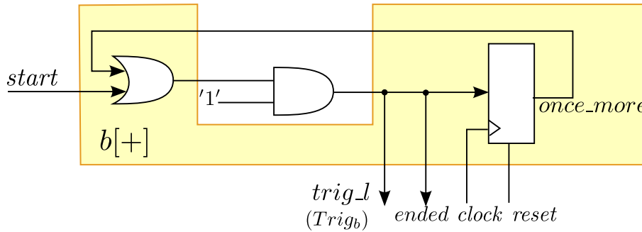
FIGURE 6.18: Implementation of b[+]
