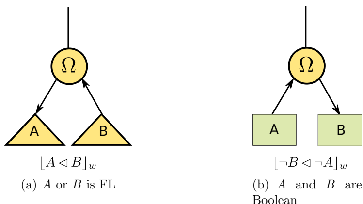
FIGURE 7.3: The representation of the [A \triangleleft B]_w dependency relation
