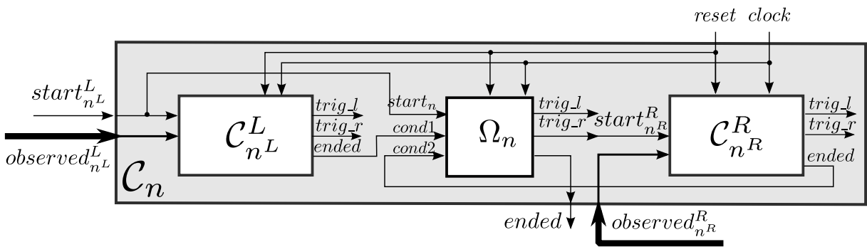
FIGURE 8.10: Recursive construction of circuit \mathcal{C}_n ( \Omega_n \in \{;, :\} )
