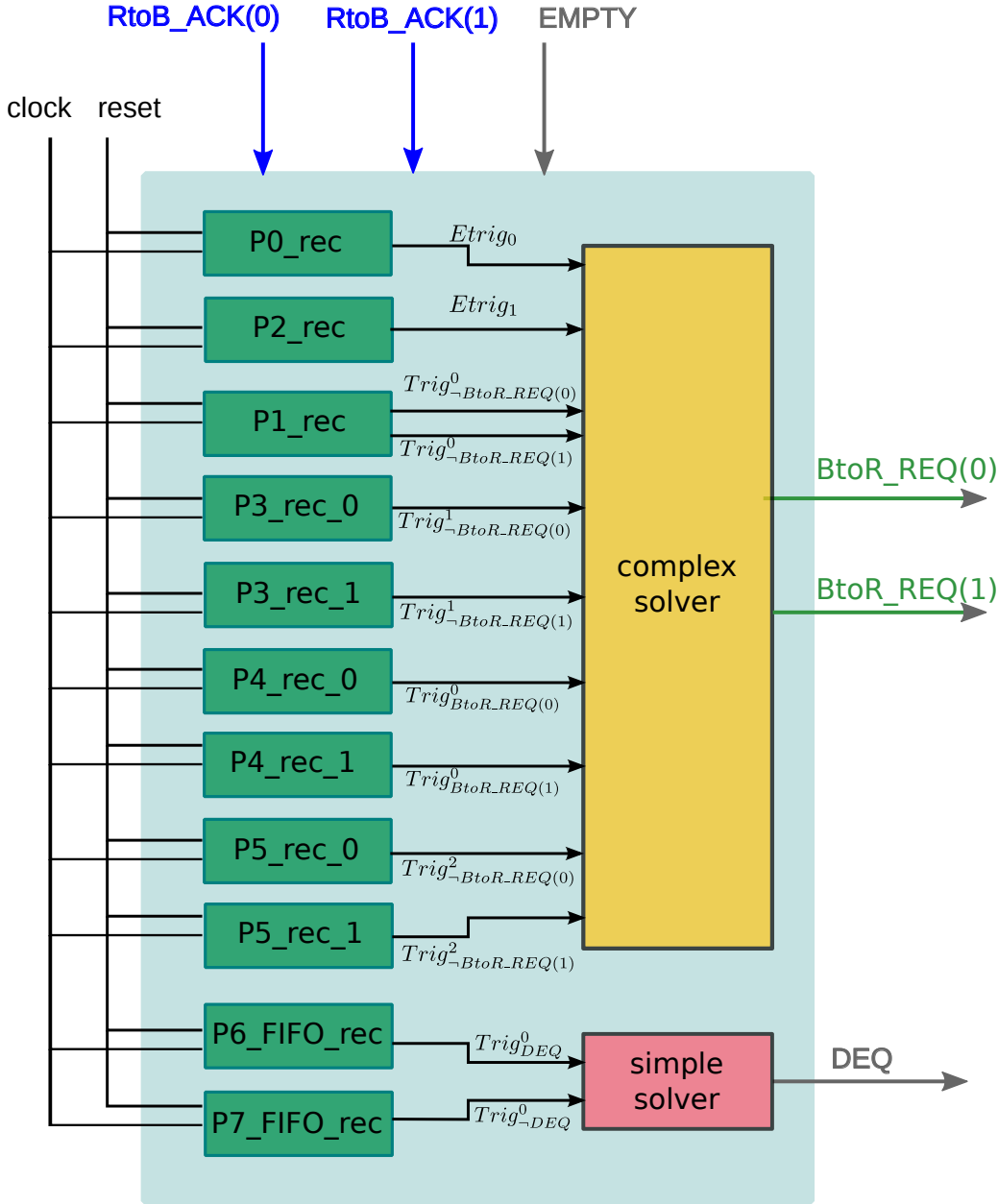
FIGURE 9.10: The final circuit of GenBufRec
