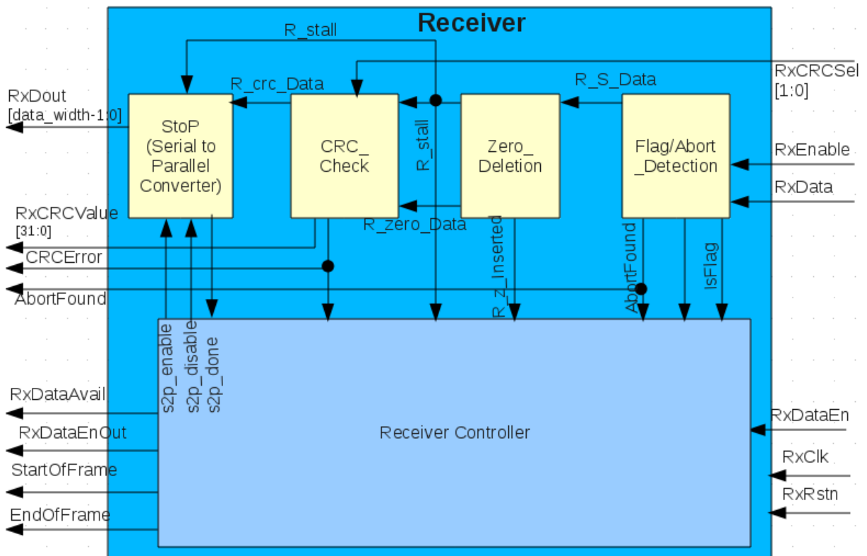
(b) Receiver
