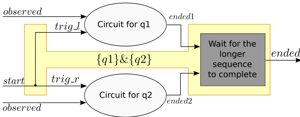
FIGURE 6.17: Implementation of \{q1\} \& \{q2\}
