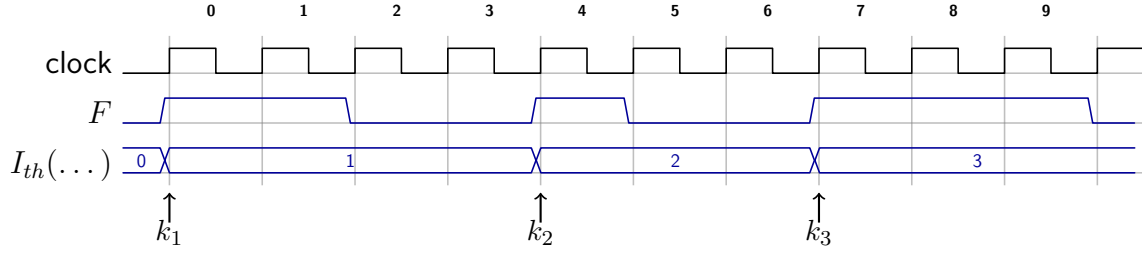
FIGURE 5.4: Illustration of function I_{th}([F \triangleleft true]_w^{k_i})
