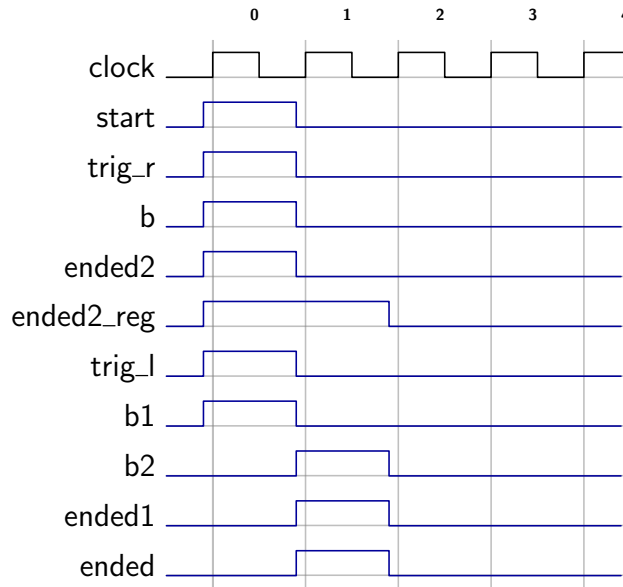
FIGURE 6.16: Timing diagram of \{b1; b2\} \& b
