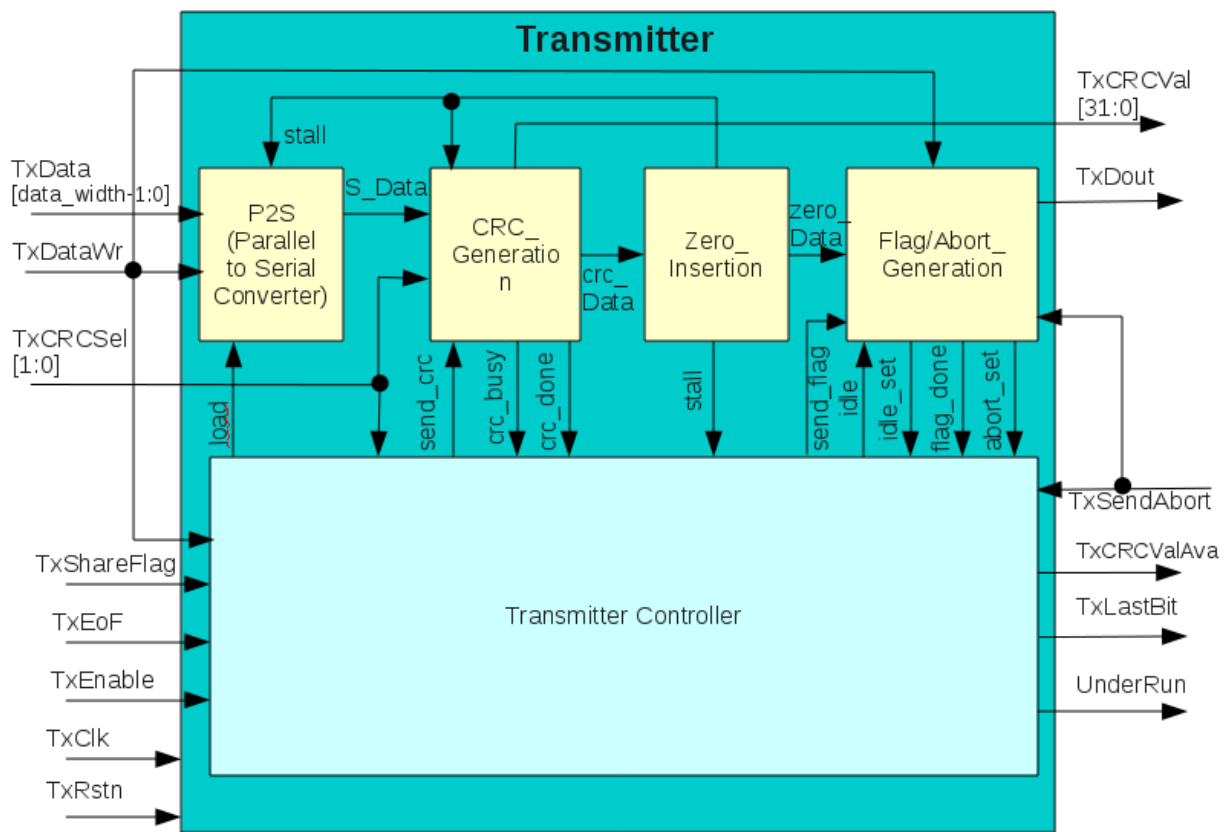
(a) Transmitter
