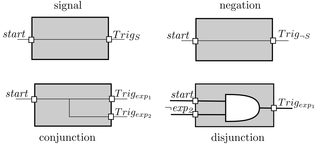
FIGURE 5.3: Boolean reactant
