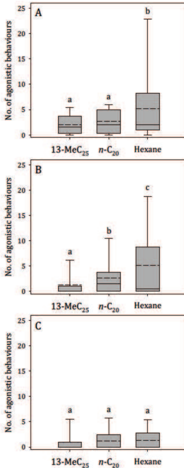
Figure 2. Total number of agonistic behaviours performed by focal workers towards nestmates with different treatments (13-MeC 25 , n-C 20 and solvent) in each condition. (A) High-ranking focal ants are confronted to low-ranking treated stimuli. (B) High-ranking focal ants are confronted to high-ranking treated stimuli. (C) Low-ranking focal ants are confronted to low-ranking treated stimuli. Box plots represent 10th, 25th, 50th (median), mean (dotted line), 75th and 90th percentiles. Sample sizes of individuals are N = 12 for each box plot. Different letters denote statistical differences.
