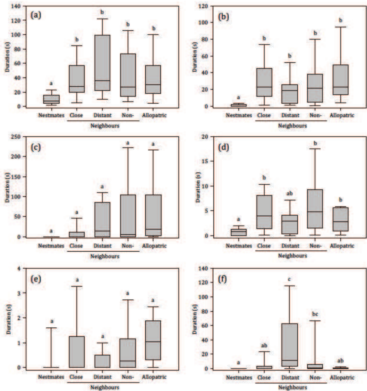
Figure S2. Duration (s) of each behaviour in dyadic encounters between ants originating from nests separated by various categories of spatial distance in N. apicalis morph 4. (a) Antennation. (b) Antennal boxing. (c) Transport. (d) Mandible opening. (e) Biting. (f) Stinging. Box plots represent 10th, 25th, 50th (median), 75th and 90th percentiles. Sample sizes of encounters are N = 10 for each box plot, except for distant neighbours encounters where N = 9 . Different letters denote statistical differences.
