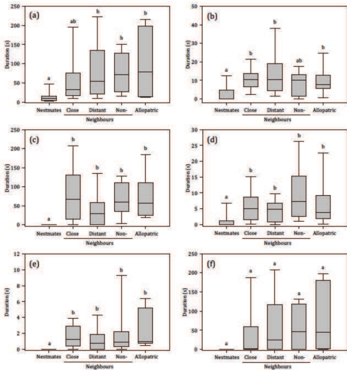
Figure S3. Duration (s) of each behaviour in dyadic encounters between ants originating from nests separated by various categories of spatial distance in N. verenae morph 1. (a) Antennation. (b) Antennal boxing. (c) Transport. (d) Mandible opening. (e) Biting. (f) Stinging. Box plots represent 10th, 25th, 50th (median), 75th and 90th percentiles. Sample sizes of encounters are N = 10 for each box plot. Different letters denote statistical differences.
