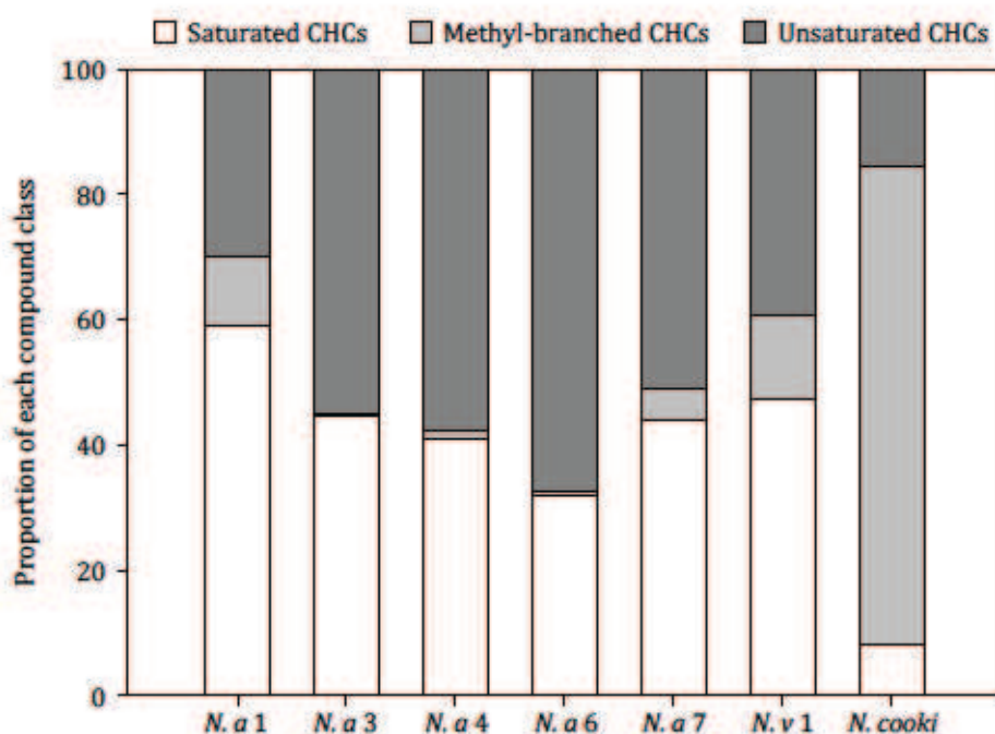
Figure 1. Mean proportion of each major class of CHCs in the chemical profiles of all morphs. N. a , N. apicalis ; N. v , N. verenae .
