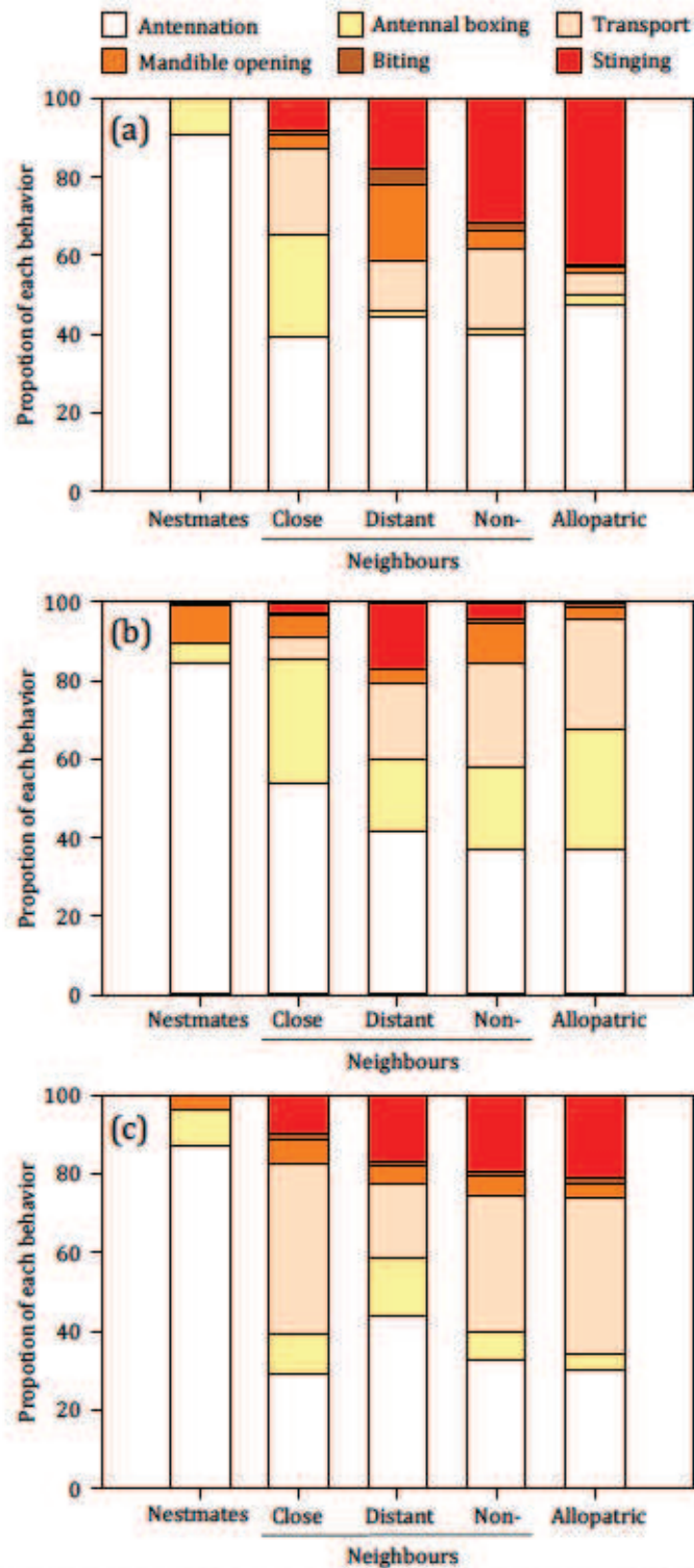
Figure 2. Proportion of all behaviours (duration) during dyadic encounters between ants originating from nests separated by various categories of spatial distance. (a) N. apicalis morph 7. (b) N. apicalis morph 4. (c) N. verenae morph 1. Sample sizes of encounters are N = 10 for each bar, except for allopatric encounters in (a) and distant neighbours encounters in (b) where N = 9 .
