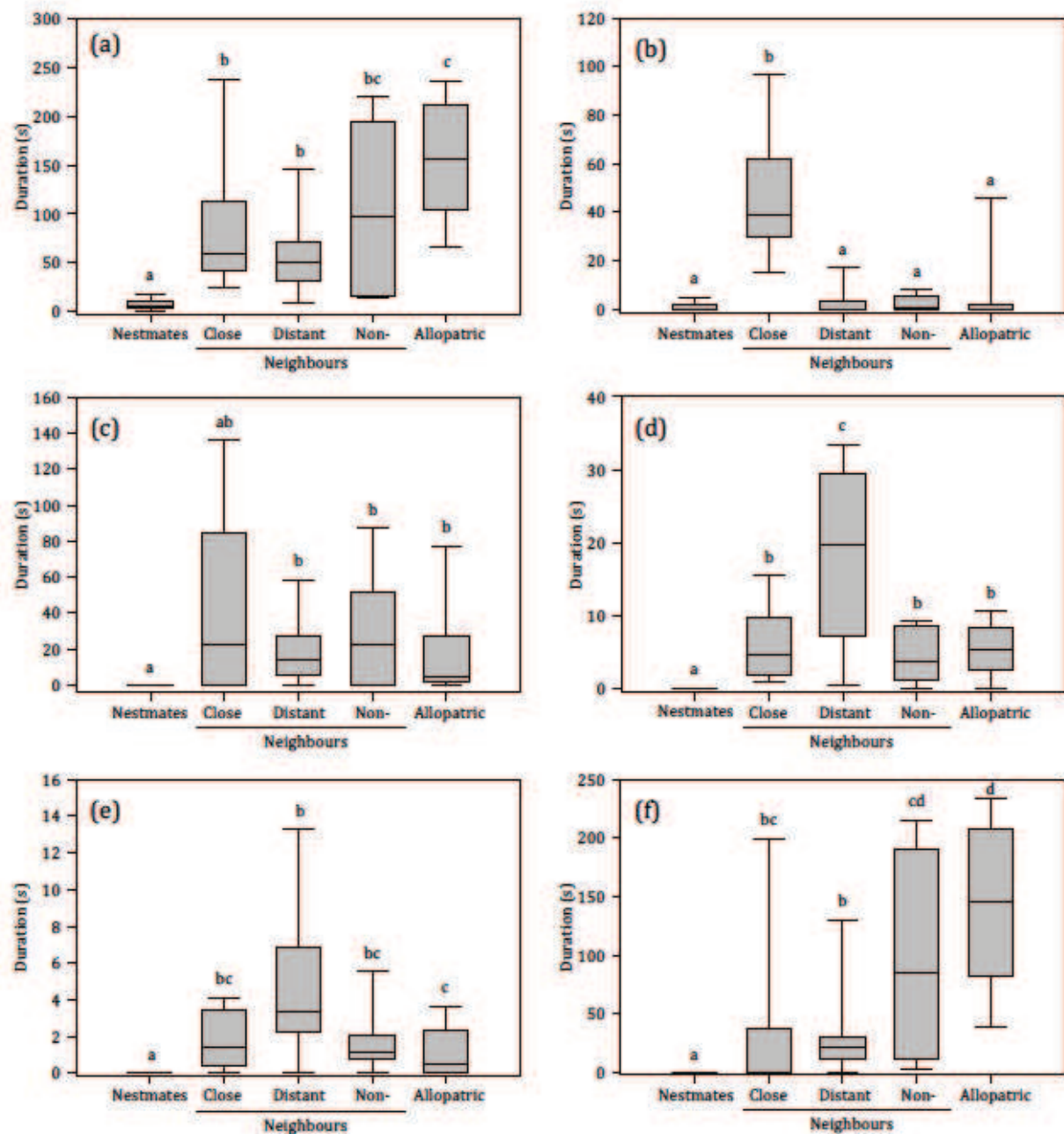
Figure S1. Duration (s) of each behaviour in dyadic encounters between ants originating from nests separated by various categories of spatial distance in N. apicalis morph 7. (a) Antennation. (b) Antennal boxing. (c) Transport. (d) Mandible opening. (e) Biting. (f) Stinging. Box plots represent 10th, 25th, 50th (median), 75th and 90th percentiles. Sample sizes of encounters are N = 10 for each box plot, except for allopatric encounters where N = 9 . Different letters denote statistical differences.
