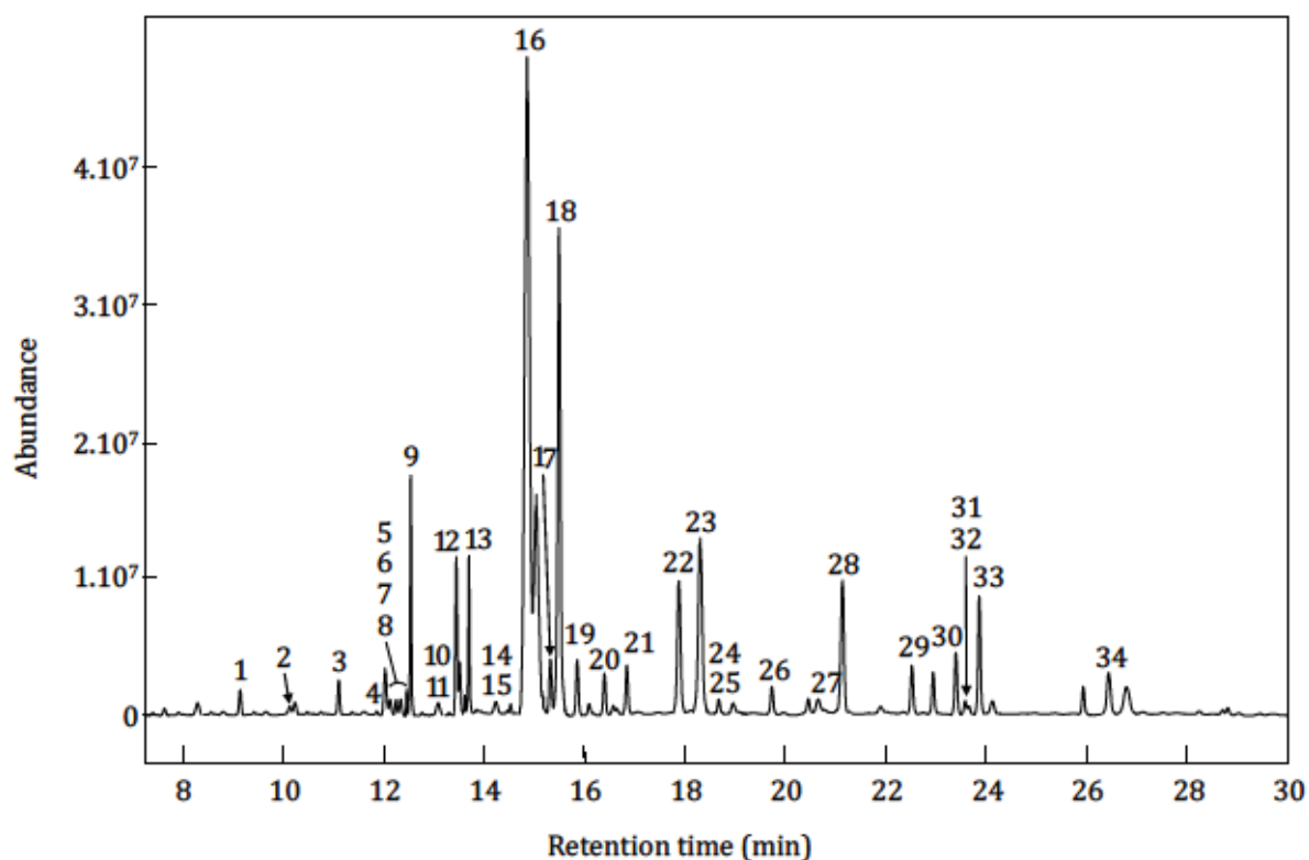
Figure A1. Chromatogram of the cuticular hydrocarbon profile of a moderately fertile N. apicalis worker. Peaks used in the statistical analysis are indicated by numbers: 1 = unidentified; 2 = 10-MeC 19 ; 3 = n -C 20 ; 4 = unidentified; 5 = C 21:1 ; 6 = C 21:1 ; 7 = C 21:1 ; 8 = C 21:1 ; 9 = n -C 21 ; 10 = 11-MeC 21 ; 11 = 9-MeC 21 ; 12 = C 22:2 ; 13 = n -C 22 ; 14 = 11-MeC 22 ; 15 = 9-MeC 22 ; 16 = C 23:2 ; 17 = C 23:1 ; 18 = n -C 23 ; 19 = 11-MeC 23 ; 20 = C 24:2 ; 21 = n -C 24 ; 22 = C 25:2 ; 23 = n -C 25 ; 24 = 13-MeC 25 ; 25 = 11-MeC 25 ; 26 = n -C 26 ; 27 = C 27:2 ; 28 = n -C 27 ; 29 = n -C 28 ; 30 = 2-MeC 28 ; 31 = C 29:2 ; 32 = C 29:1 ; 33 = n -C 29 ; 34 = n -C 31 .
