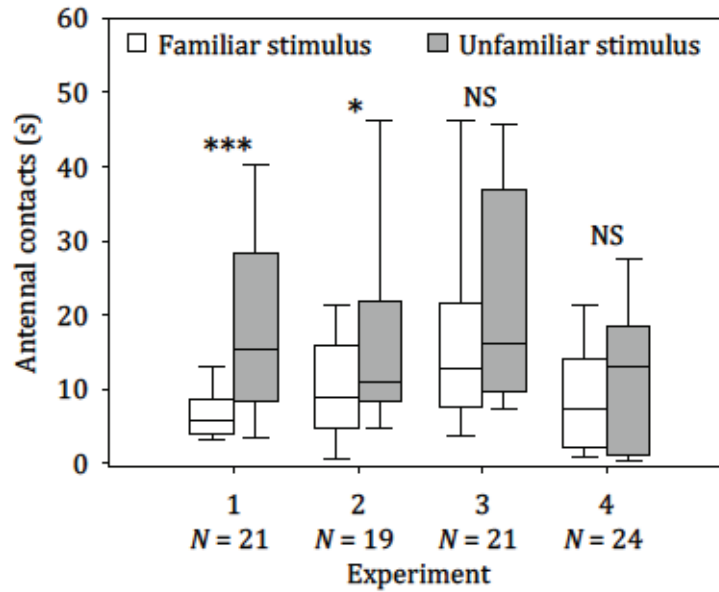
Figure 2. Duration of antennal contacts (s) towards the familiar and unfamiliar stimuli during discrimination tests in all experiments. In experiments 1–3, tested ants were high rankers and were confronted with a low- and a high-ranking nestmate (experiment 1), two high-ranking nestmates (experiment 2) or two low-ranking nestmates (experiment 3). In experiment 4, tested ants were low rankers and both stimuli were high-ranking nestmates. Box plots represent 10th, 25th, 50th (median), 75th and 90 th percentiles. Sample sizes of individuals are indicated below each box plot. *** P < 0.001 ; * P < 0.05 .
