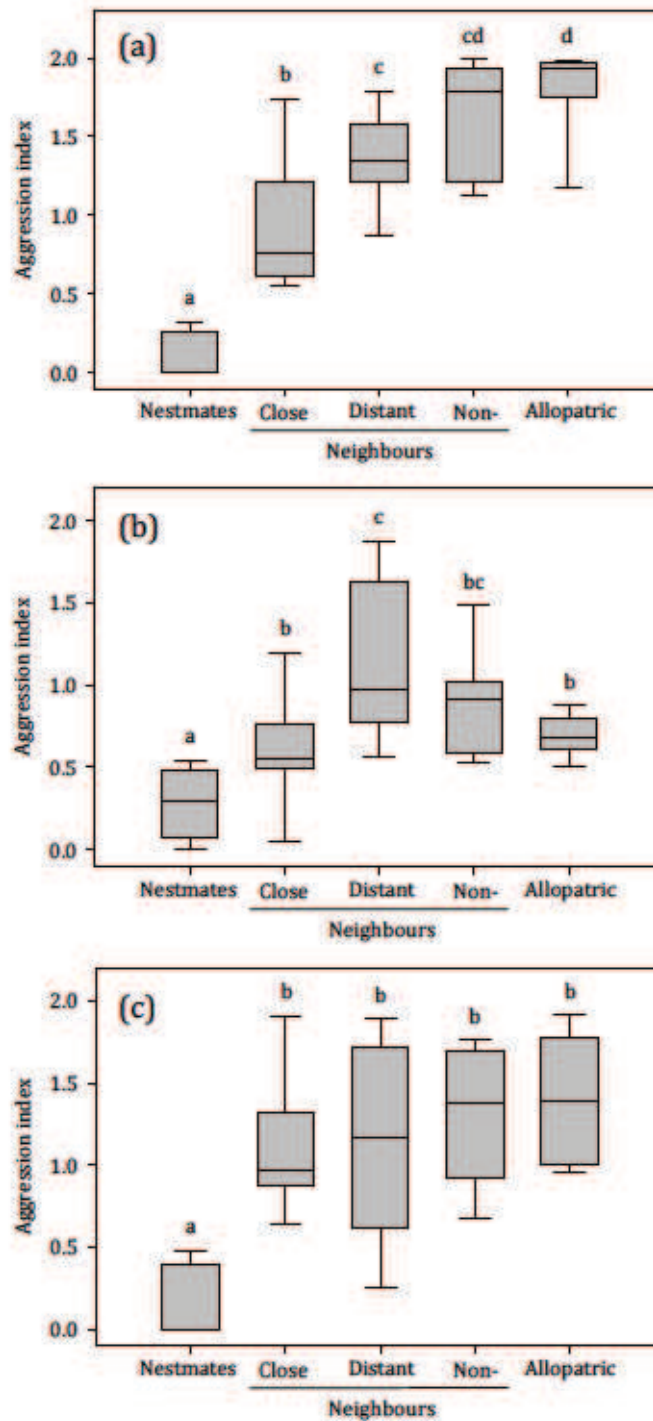
Figure 1. Aggression index in dyadic encounters between ants originating from nests separated by various categories of spatial distance. (a) N. apicalis morph 7. (b) N. apicalis morph 4. (c) N. verenae morph 1. Box plots represent 10th, 25th, 50th (median), 75th and 90th percentiles. Sample sizes of encounters are N = 10 for each box plot, except for allopatric encounters in (a) and distant neighbours encounters in (b) where N = 9 . Different letters denote statistical differences.
