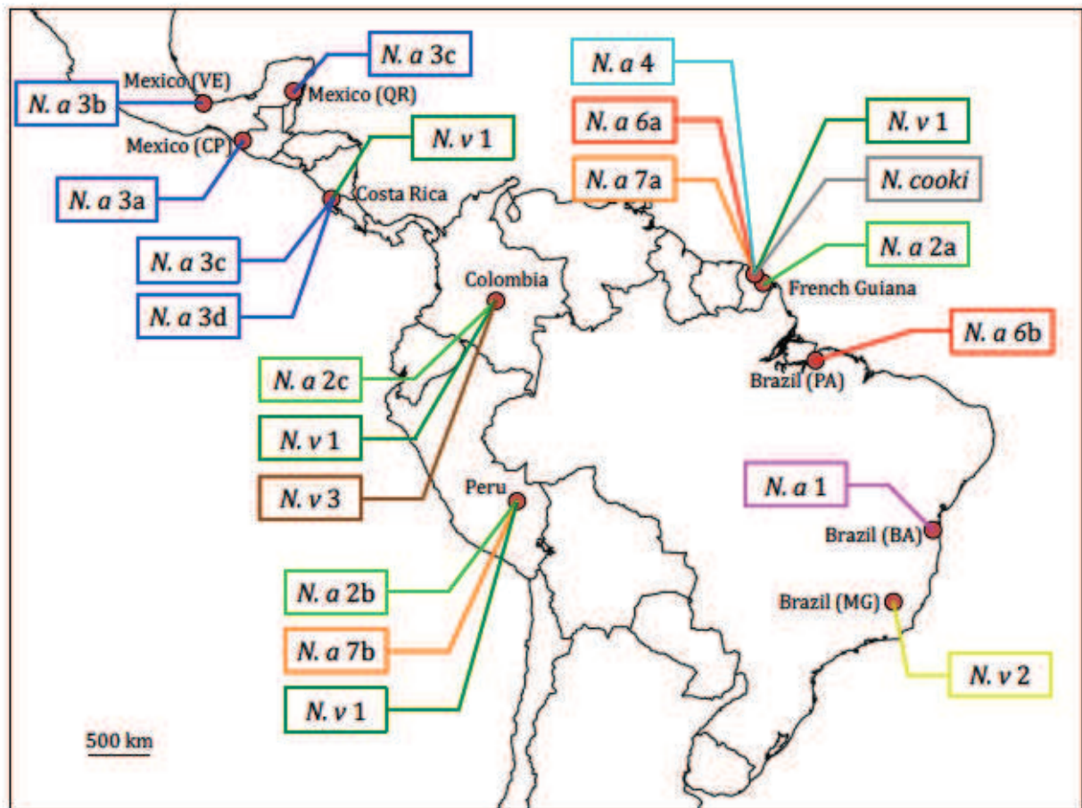
Figure 5. Geographical location of all morphs of the N. apicalis species complex sampled in this study.
