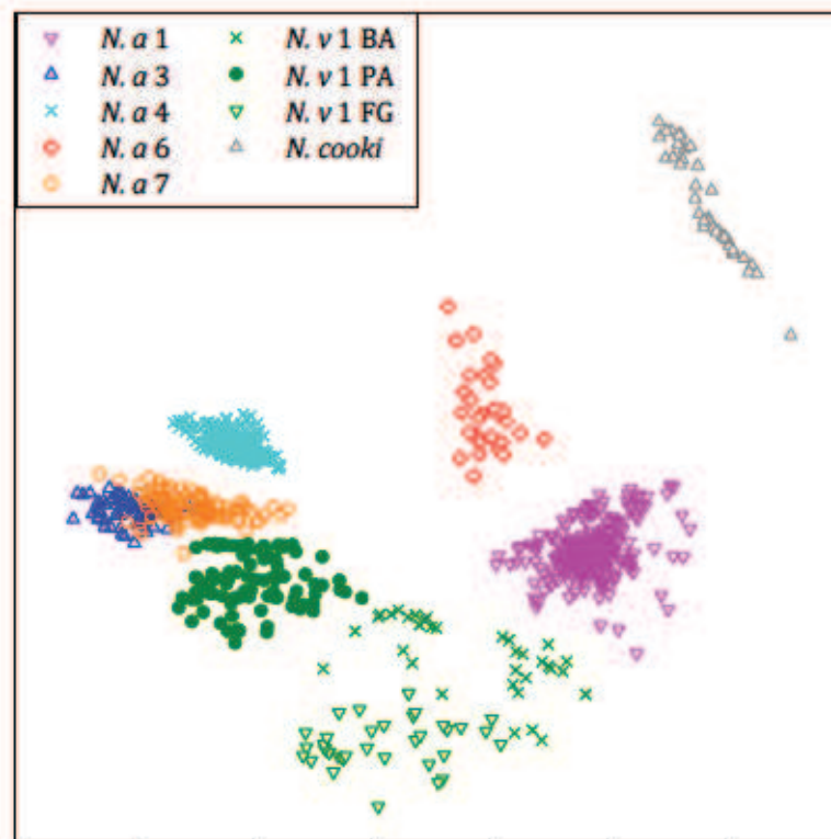
Figure 2. NMDS plot of the CHC profiles of all morphs and of geographic origin for N. verenae morph 1 (2D stress = 0.13). N. a , N. apicalis ; N. v , N. verenae ; BA, Bahia; PA, Pará; FG, French Guiana.
