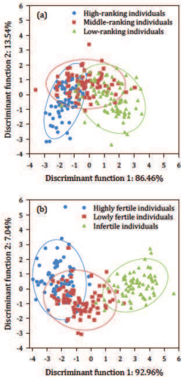
Figure A3. Discriminant function analyses showing the differences in the chemical profiles of 223 workers according to their (a) hierarchical rank and (b) ovarian development. Ellipses represent 90% confidence intervals around centroids. The percentage of variance explained is depicted on each axis.
