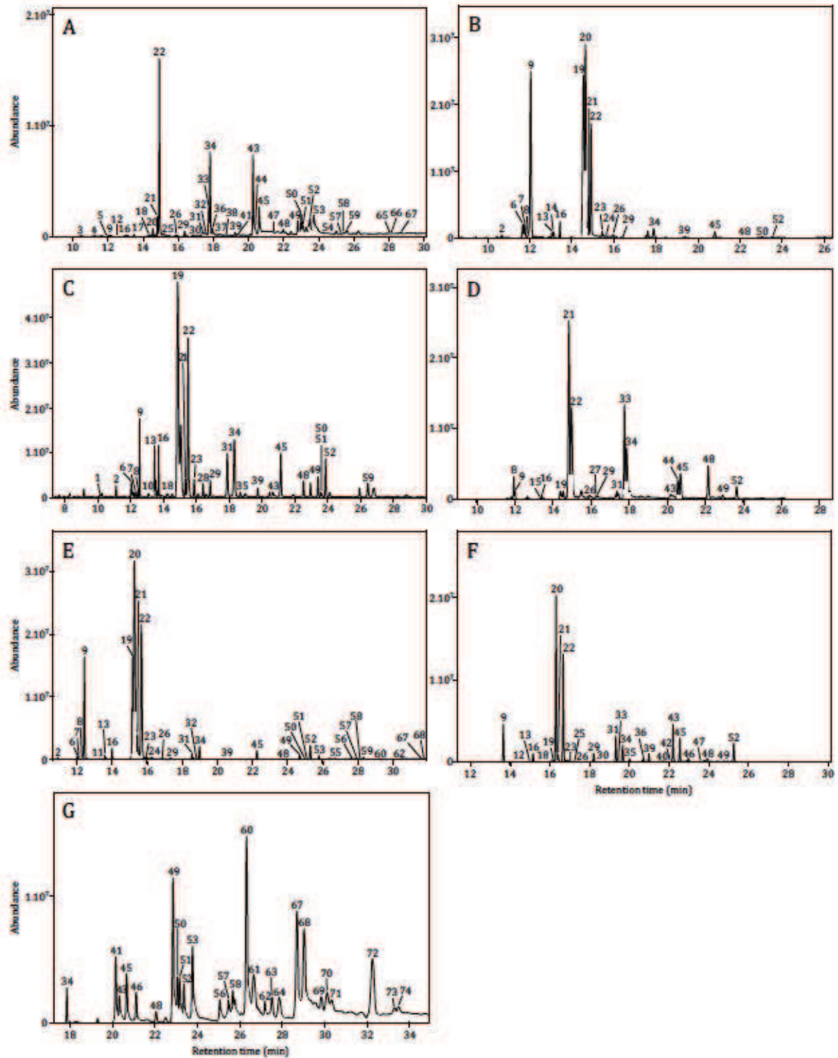
Figure S1. Chromatogram of the CHC profiles of moderately fertile workers in all morphs. A, N. apicalis morph 1. B, N. apicalis morph 3. C, N. apicalis morph 4. D, N. apicalis morph 6. E, N. apicalis morph 7. F, N. verenae morph 1 from Pará. G. N. cooki . Peaks used in the chemical analyses are indicated by numbers and refer to Table S1.
