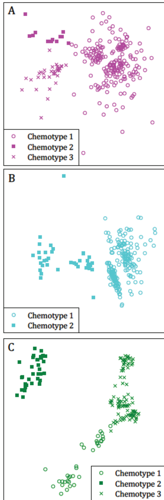
Figure S2. NMDS plot of the CHC profiles of chemotypes in (A) N. apicalis morph 1 (2D stress = 0.14), (B) N. apicalis morph 4 (2D stress = 0.10), and (C) N. verenae morph 1 (chemotype 1, Bahia; chemotype 2, French Guiana; chemotype 3, Pará; 2D stress = 0.08).
