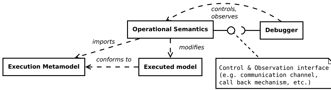
Figure 2.9: Typical architecture for interactive debugging.
