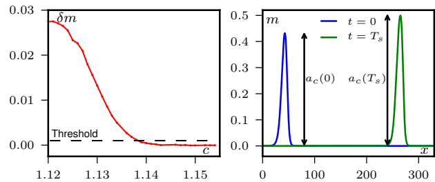
FIG. 13. Stability of homoclinic orbits in the hydrodynamic equations. \Delta a_c is the difference in the amplitude of the solution measured between t = 0 and t = T_s . The solution is declared to be linearly stable if \delta m(T_s) , defined in Eq. (53) is smaller than a threshold that we take at 10^{-3} . v_0 = \lambda = \xi = a_4 = \varphi_g = 1 , c = 1.125 (right)
