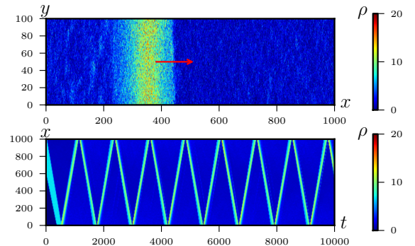
FIG. 21. Active Ising model with closed boundary conditions. Top: snapshot of the density field. Bottom: space-time graph (averaged in the y -direction) showing the liquid domain bouncing back and forth in the box. Parameters: \beta = 1.9 , \rho_0 = 3 , D = 1 , \varepsilon = 0.9 . See supplementary movies in [49].
