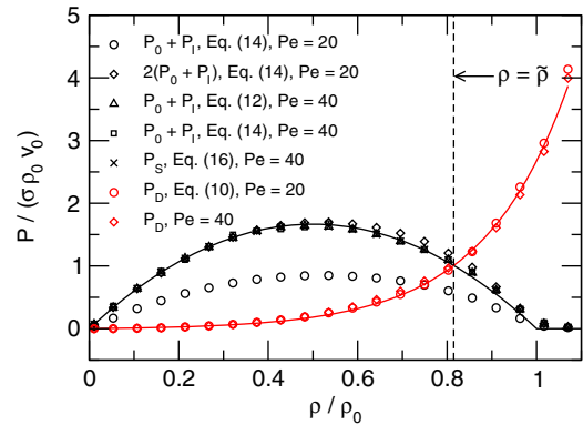
FIG. 1 (color online). Numerical measurements of P_0 + P_I , P_S , and P_D in single-phase ABP simulations at Péclet number Pe \equiv 3v_0/(D_r\sigma) = 40 , where \sigma is the particle diameter. Expressions (12), (14), and (16) for P_0 + P_I and P_S show perfect agreement. Also shown are data for Pe = 20 , unscaled and rescaled by factor 2. This confirms that P_S = P_0 + P_I is almost linear in Pe ; small deviations arise from the Pe dependence of the correlators. In red is P_D for Pe = 20, 40 , with no rescaling. Pe was varied using D_r , at fixed v_0 and with D_t = D_r\sigma^2/3 . Solid lines are fits to piecewise parabolic ( P_S ) and exponential ( P_D ) functions used in the semiempirical equation of state. \rho_0 is a near-close-packed density at which v(\rho) vanishes and \tilde{\rho} is the threshold density above which P_D > P_S . See the Supplemental Material [39] for details.
