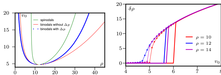
Fig. 1. The phase diagram ( left ) predicted by the theory without the \Delta\mathbf{p} term (red and green lines) are only qualitatively affected by the \Delta\mathbf{p} term (blue). Hysteresis loops ( right ), showing the first order nature of the transition, can be seen on approach to the critical point by ramping up (solid lines) or down (connected symbols). D = 0.25 , v_1 = 0.25 , \phi = 4 , \tau = 1/D_r = 1 .
