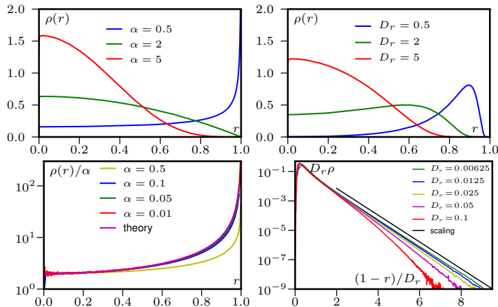
Fig. 2. SPPs in a harmonic trap ( v = \kappa = 1 in simulation units). As \Phi = \kappa\tau increases, \rho(r) goes from a Gaussian centered on r \simeq 0 to a distribution peaked at r \simeq v/\kappa ; this holds for both RTPs (top left) and for ABPs (top right). As \Phi diverges, the density of RTPs in the bulk scales as 1/\Phi (bottom left), while the density of ABPs in the bulk scales exponentially with D_r , and the profile \rho(r) decreases exponentially with the distance to the trap boundary (bottom right).
