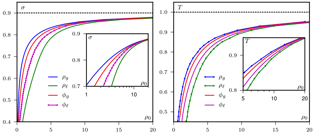
FIG. 17. Phase diagram of the Visek (left) and Ising (right) hydrodynamic equations. The spinodal lines \varphi_g and \varphi_l are known exactly except \varphi_l in the Visek hydrodynamic equation which we computed numerically by looking at the stability of systems of size 50 \times 50 . The binodals \rho_g and \rho_l are the coexisting densities of phase-separated (heteroclinic) solutions as explained in the text. The dashed line indicate the asymptote above which only disordered solutions exist. Insets are close-ups on the high-density regions with a logarithmic scale on the x -axis. Parameters: v_0 = D = 1 = r = 1 (Ising), v_0 = 1 (Visek).
