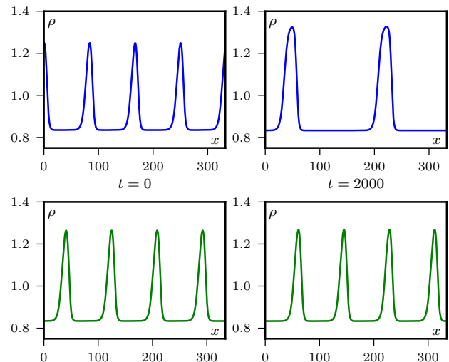
FIG. 15. Evolution of two propagative solutions in the hydrodynamic equations (7-8). The initial conditions are stable limit cycles of the dynamical system (13) for m(z) . Top row: unstable solution with c = 1.135 , \rho_g = 0.8351 . Bottom row: stable solutions with c = 1.14 , \rho_g = 0.8341 . System size 340 \times 100 , dt = 0.1 , dx = 0.4 . v_0 = \lambda = \xi = a_4 = \varphi_g = 1 .
