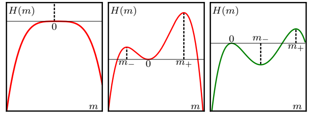
FIG. 4. The green potential can give rise to physical (positive, non-exploding) solutions while the red ones are ruled out by our conditions (C1) (left) and (C2) (center).
