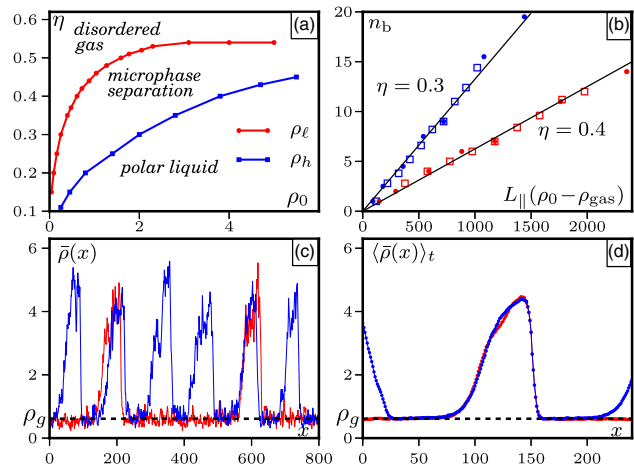
FIG. 2 (color online). (a) Phase diagram of the Vicsek model. The binodals \rho_\ell(\eta) and \rho_h(\eta) mark the limit of the coexistence region. (b) Number of bands vs L_{||}(\rho_0 - \rho_{\text{gas}}) varying either the excess density for L_x \times L_y = 2000 \times 100 (squares) or the system size along the direction of propagation (dots) for \rho_0 = 0.6 ( \eta = 0.3 ) or \rho_0 = 1.2 ( \eta = 0.4 ). The straight black lines are guides for the eyes. (c) Density profiles of Fig. 1 averaged along the transverse direction \mathbf{e}_\perp , \bar{\rho}(x_{||}) = \langle \rho(x_\perp, x_{||}) \rangle_{x_\perp} . (d) Time average of the band profiles shown in (c). A threefold increase of the excess density changes the number of bands but not the gas density or the shape of the bands. v = 0.5 , \eta = 0.4 , \rho_0 = 1.05 (red/light grey lines), \rho_0 = 1.93 (blue/dark grey lines).
