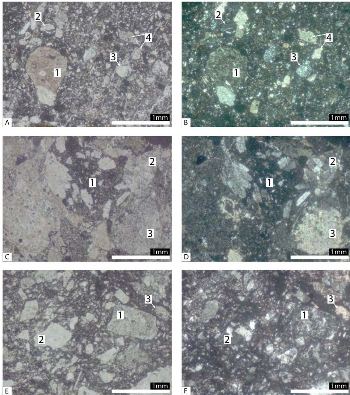
Figure S1. Thin-section micrograph of the analyzed volcaniclastic rocks samples. Left column: plane-polarized light; right column: cross-polarized light.
