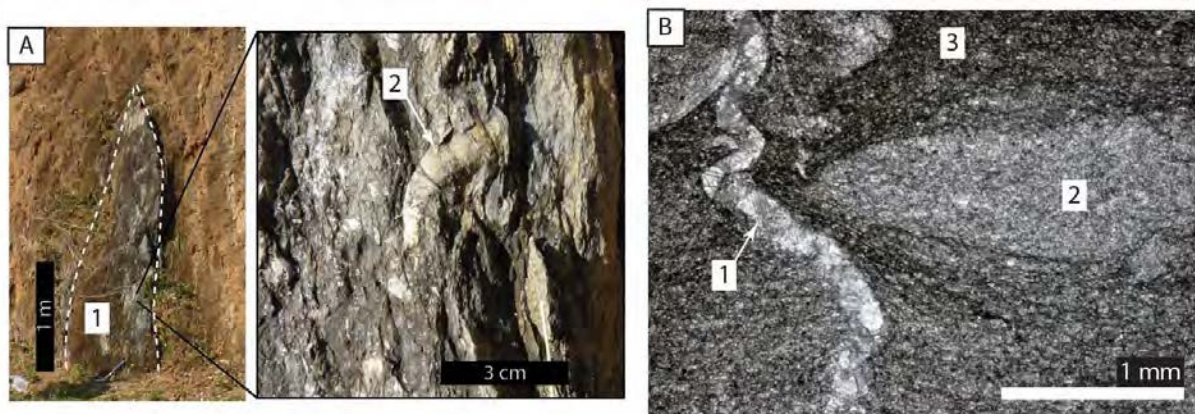
Figure 4.25. Formation de Yen Duyet.
