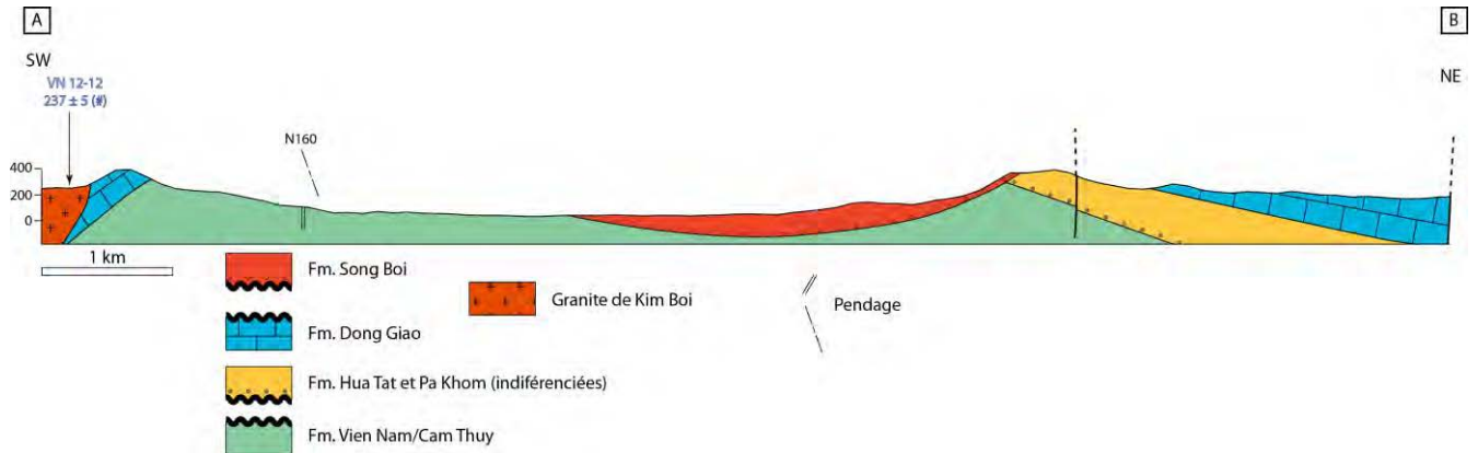
Figure 4.38. Coupe de Bac Phong.
