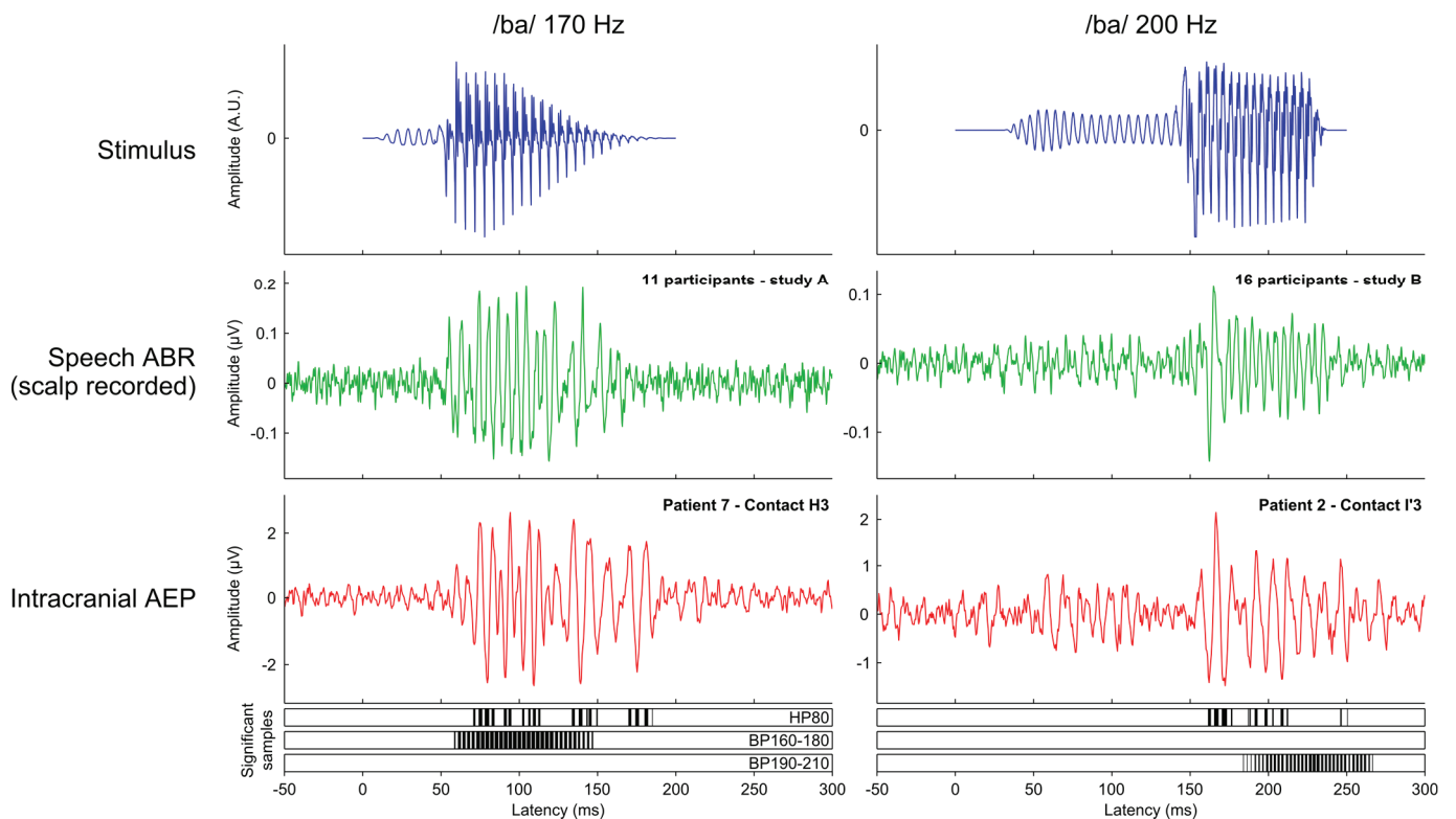
Fig. 1. Comparison between scalp-recorded Speech ABR and intracranial speech-evoked AEP exhibiting the cortical FFR. Data evoked by both ba170 and ba200 stimuli are presented on left and right columns, respectively. Below intracranial AEP, samples significantly emerging from baseline are shown for different filtering ( p < 0.05 , FDR-corrected; HP80 = 80-Hz high-pass filter; BP160-180 = 160-to-180-Hz band-pass filter; BP190-210 = 190-to-210-Hz band-pass filter).
