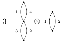
Figure 5.14: Another terms obtained by acting with the coproduct on the standard labeled TAG of Fig 5.12.
