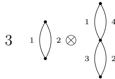
Figure 5.13: One of the terms obtained by acting with the coproduct on the standard labeled TAG of Fig 5.8.
