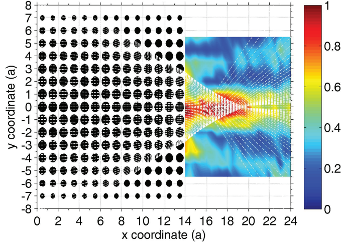
Figure 4.10: Experimental observation of normalized maximum displacement after a GRIN PC covering x = [0, 14a] . Dashed lines indicate ray trajectories both at the inner and behind the GRIN PC. Circles indicate the air holes.
