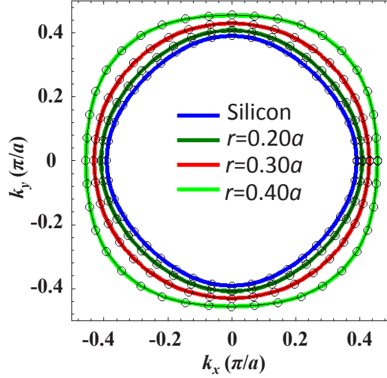
Figure 2.9: EFCs at 5 MHz (solid lines) and the corresponding fits derived from equation (2.20) (circular markers) for a PC with the square symmetry and for different sizes of the air holes.
