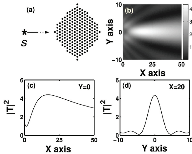
Figure 1.7: Acoustic focusing 42 by using a shaped PC featuring a positive index at the low frequencies: (a) scheme of geometric lens, (b) two-dimensional distribution of the measured intensity |T|^2 , (c) the intensity along the symmetric axis, and (d) the intensity along the transverse axis at the peak value in (c).
