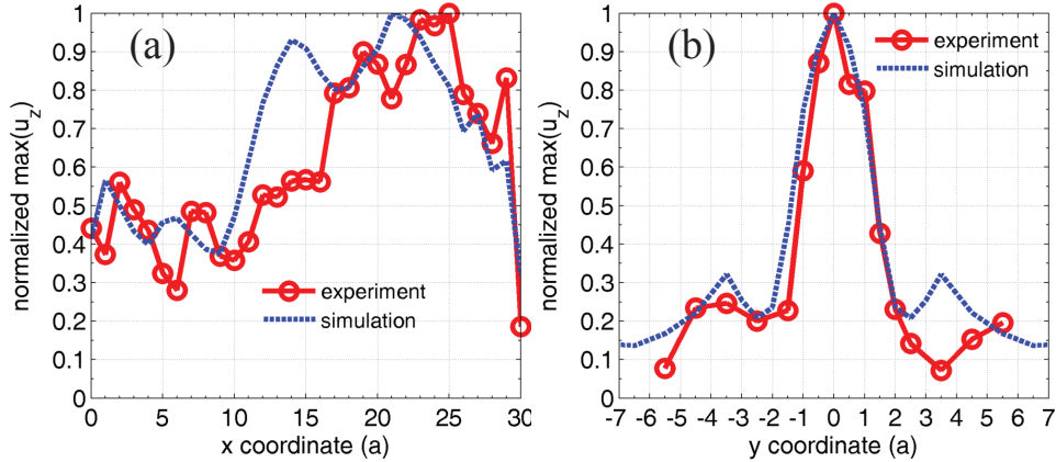
Figure 4.9: Focusing through a GRIN PC of 30 columns: (a) experimental (solid line) and numerical (dashed line) horizontal profile of normalized maxima of u_z at the symmetric layer of GRIN PC, and (b) experimental (solid line) and numerical (dashed line) transverse profile of normalized maxima of u_z at the focusing.
