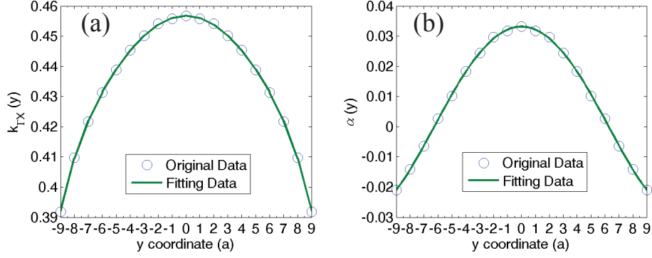
Figure A.1: Profiles of (a) wavenumber k_{\Gamma X} and (b) anisotropy coefficient \alpha . In both figures, the circles stand for discrete obtained by FEM while the solid lines indicate the fitting curves from equations (A.2) and (A.3).
