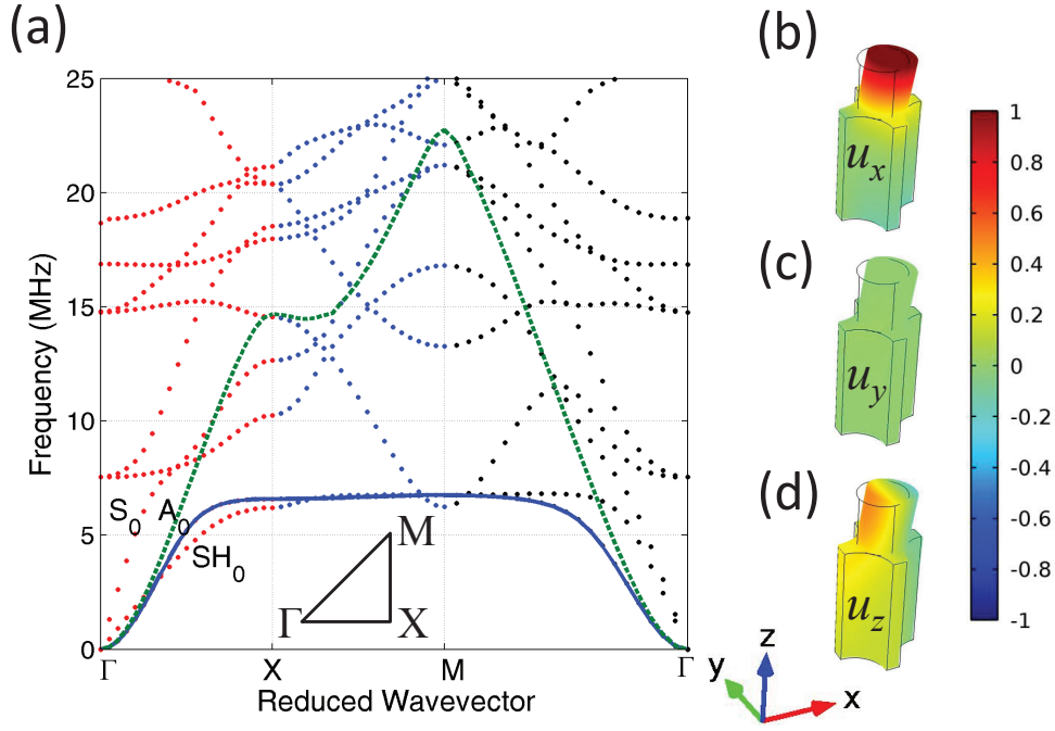
Figure 3.6: (a) Acoustic bands for a trampoline PC with a = 100 \mu\text{m} , h = 153 \mu\text{m} , h_p = 65 \mu\text{m} , r_a = 41.3 \mu\text{m} , r_p = 30 \mu\text{m} . Solid line and dashed line indicate A_0 mode bands of structures with and without silicon pillar, respectively. Normalized modal displacement of A_0 band of trampoline for (b) u_x , (c) u_y and (d) u_z along \Gamma X at k_{\Gamma X} = 0.586\pi/a . The modal deformation is also displayed in figures (b)-(d) in comparison to the initial shape of trampoline noted by solid lines.
