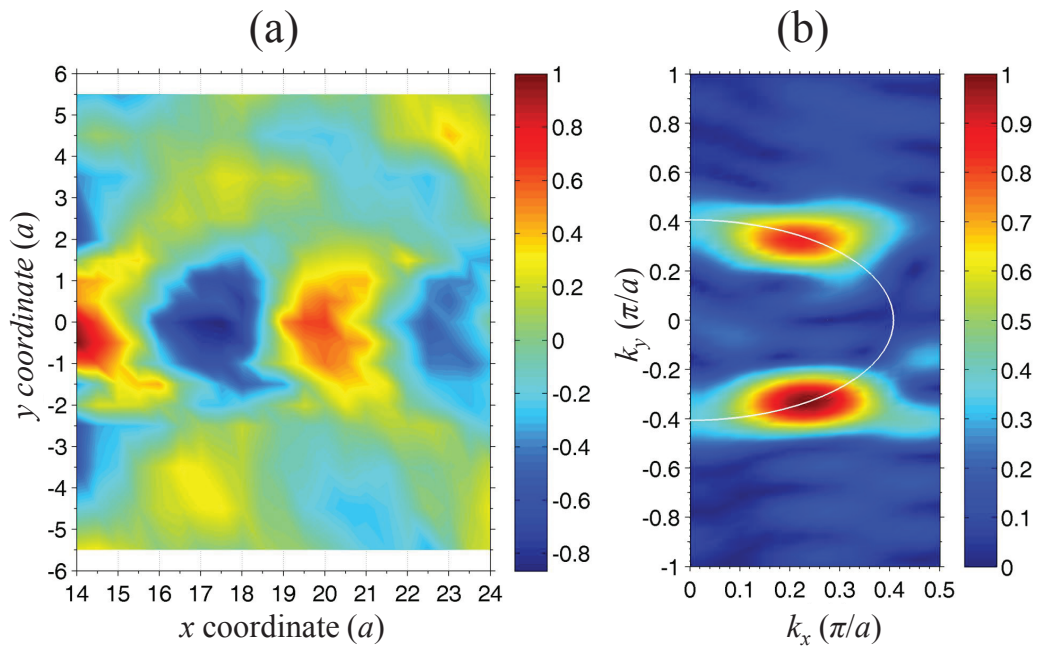
Figure 4.15: (a) Snapshot of the focusing and (b) the normalized two-dimensional Fourier transform of the snapshot image. The white solid line indicate the EFC of Rayleigh wave at 20 MHz.
