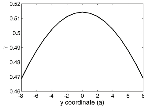
Figure A.6: Profile of \gamma against y -axis for the planer GRIN lens with a general hyperbolic secant profile as in equation (A.19) with n_0 = 1.116 , n_s = 1 , and \delta = 0.065^{-1} .
