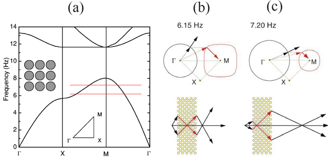
Figure 1.2: (a) Band structure of a PC. Two frequencies are chosen in the first branch at 6.15 Hz and 7.20 Hz. (b) The equal frequency contour at 6.15Hz for both the background medium (black line) and the PC (red line), and (c) the equal frequency contour at 7.20 Hz for both the background medium (black line) and the PC (red line). 13 The negative refraction lens is formed at the first branch through the relationship \mathbf{k} \cdot \mathbf{v}_g > 0 .
