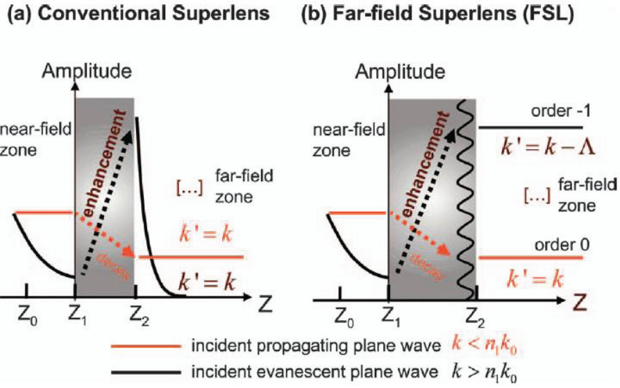
Figure 1.6: Transmitted properties of (a) conventional superlens versus (b) the far-field superlens. The conventional lens has enhanced the incident evanescent component. However the amplitude decreases quickly at the near field. The far-field superlens can also recover the incident evanescent component. Meanwhile, the evanescent component to propagating mode at the boundary through the angular spectrum. 10
