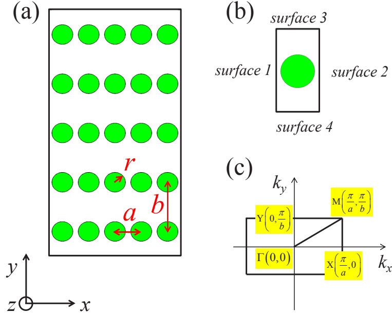
Figure 2.1: Scheme of (a) PC in rectangular lattice in the direct space, (b) unit cell, and (c) the corresponding \mathbf{k} vector in the reciprocal space.
