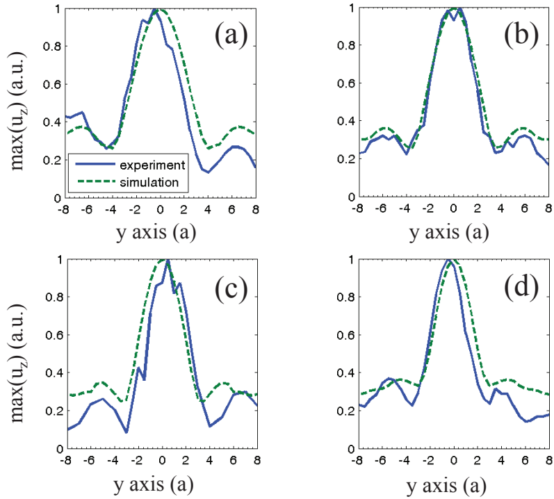
Figure 3.3: Numerical (dashed lines) and experimental (solid lines) maximum displacement profile along y -axis for GRIN PC with (a) 15, (b) 18, (c) 21 and (d) 24 layers, respectively.
