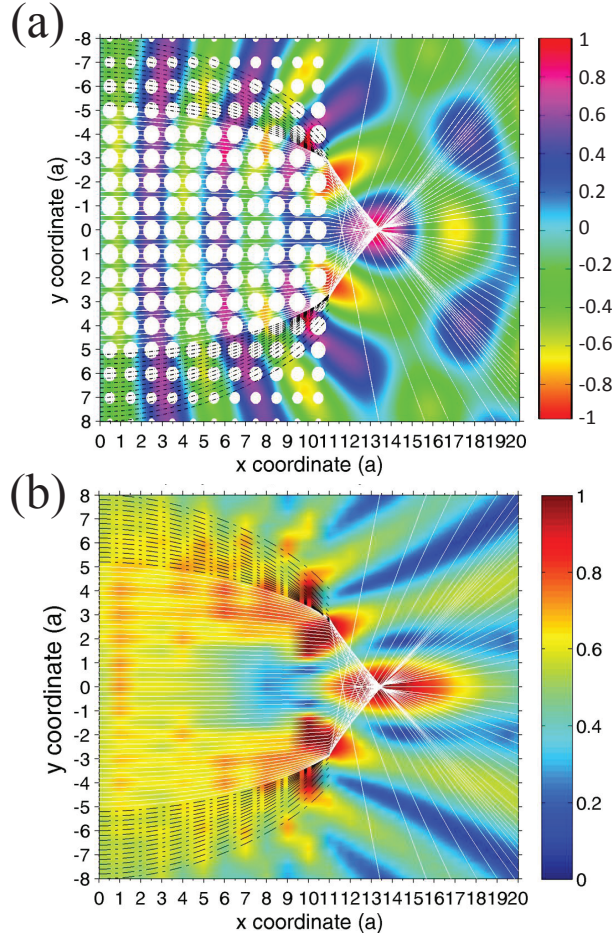
Figure 3.10: (a) Snapshot of numerical displacement u_z and (b) normalized maximum u_z both inside ( x = [0, 11a] ) and outside ( x = [11a, 20a] ) GRIN PC. The solid lines indicate ray trajectories of wave beams with a |k_y| < k_B at exit of GRIN PC ( x = 11a ); the solid lines illustrate ray trajectories of wave beams with a |k_y| > k_B at exit of GRIN PC. Accordingly these beams are no more propagating modes and ray trajectories shall not be sufficient after the exit where no ray trajectory is presented for these wave beams.
