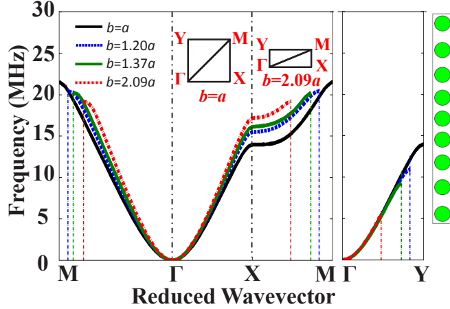
Figure 2.6: First dispersion band of Lamb mode A_0 propagating in a Si/air phononic plate with a rectangular lattice for different sizes of the unit cell along y -axis
