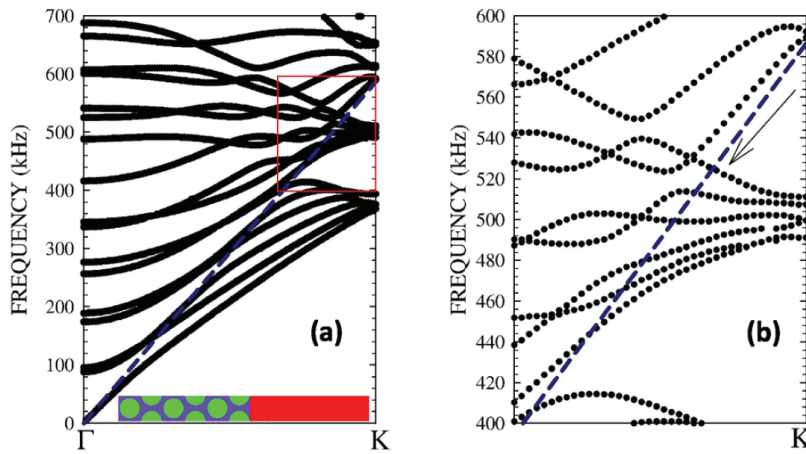
Figure 1.5: (a) Numerical investigation of the bound modes of a PC. The label indicates the used model while the dash line presents the sound line of background medium.(b) The zoom of the part in the box. The working frequency is 530 KHz, as shown in figure 1.4. 23
