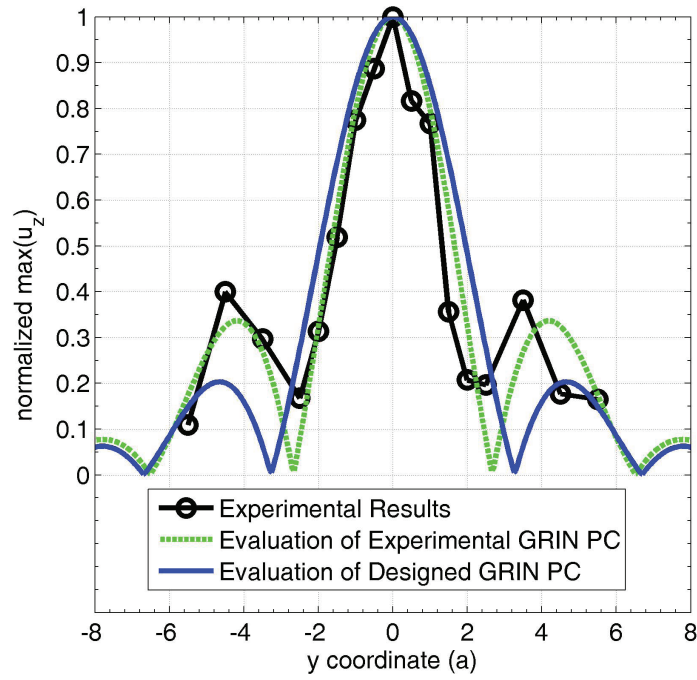
Figure 4.14: Transverse profile of maxima of |u_z| at the peak value of focus: experimental result (circles), evaluation by equation (4.3) for the actual sample of the GRIN PC (green dashed line) or the designed one (blue solid line).
