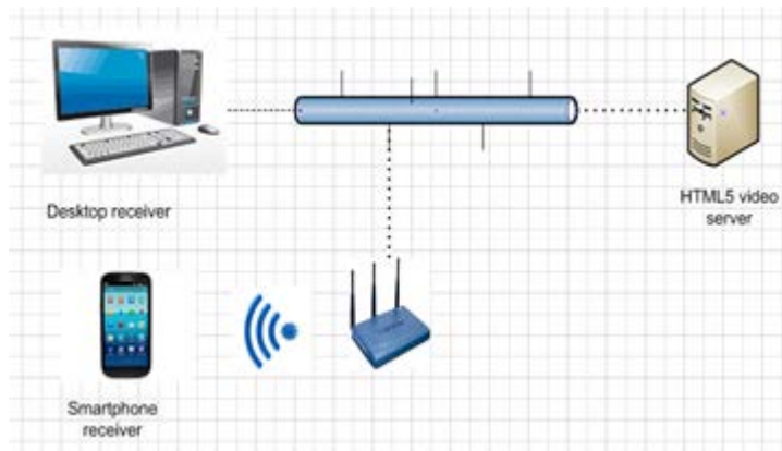
Figure 4.1: Experimental platform
