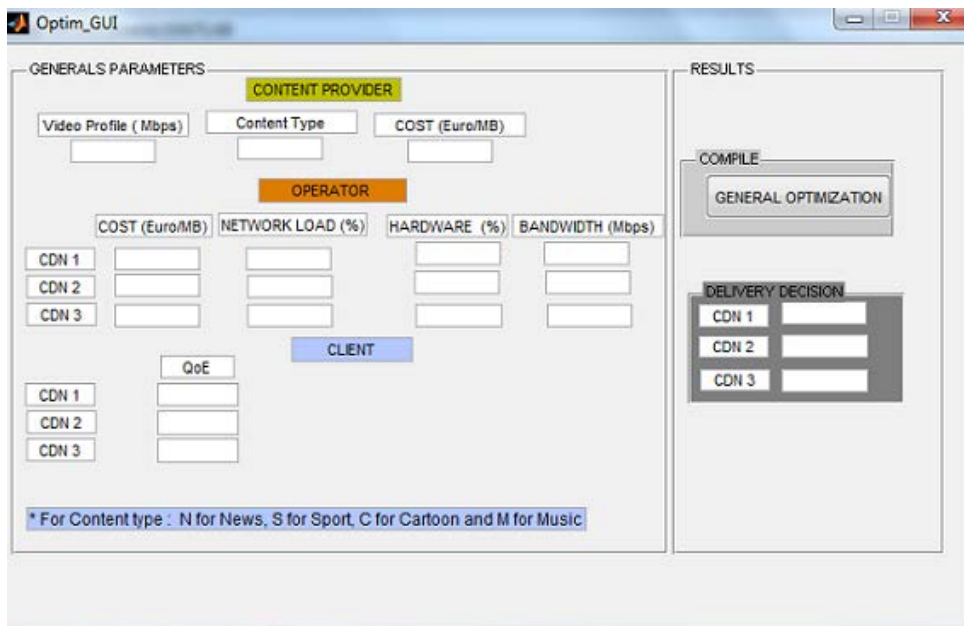
Figure A.2: GUI interface for U-VSDO approach
