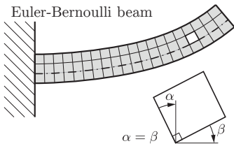
Figure 2.4: Derivation of Timoshenko and Euler Bernoulli beam. In the first part internal moments about the y -axis and shear forces due to the deformation of the beam are derived. With these results, in the second part, a set of two equations of motion is obtained for a distributed load. In the third part, considering a constant cross-section, the Timoshenko beam equation is derived and neglecting shear and rotational inertia, in the last part yields the Euler-Bernoulli equation.
