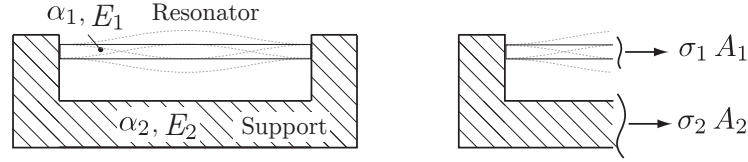
Figure 2.6: A doubly clamped beam with thermal expansion coefficient \alpha_1 and Young's modulus E_1 , being clamped in another material with \alpha_2 and E_2 . Equal elongations as well as balanced forces resulting from the inner thermal tensile stresses \sigma_i are assumed. A_i are the materials effective cross-sections. [MHc19]
