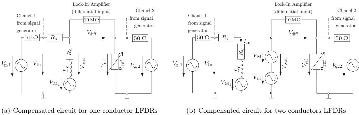
Figure 3.11: Equivalent circuits for compensating offset voltages.
