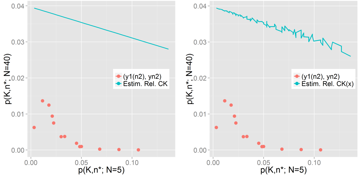
Figure 3.8: The left panel shows the estimated relationship for CK , \beta y_{1,x} . The right panel shows the relationship estimated for CK(x) , (\beta_0 + \beta_1 x)y_{1,x} . We add the estimated mean of the difference process to the relationship. We see that the slope is correct but the estimated mean of the difference is off.
