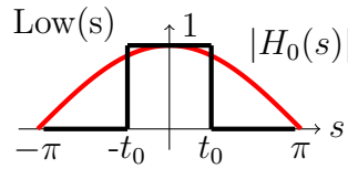
Figure B.2: The magnitude |H_0(s)| is plotted in red. The black function is an ideal low pass filter that cuts the signal at \pm t_0 .
