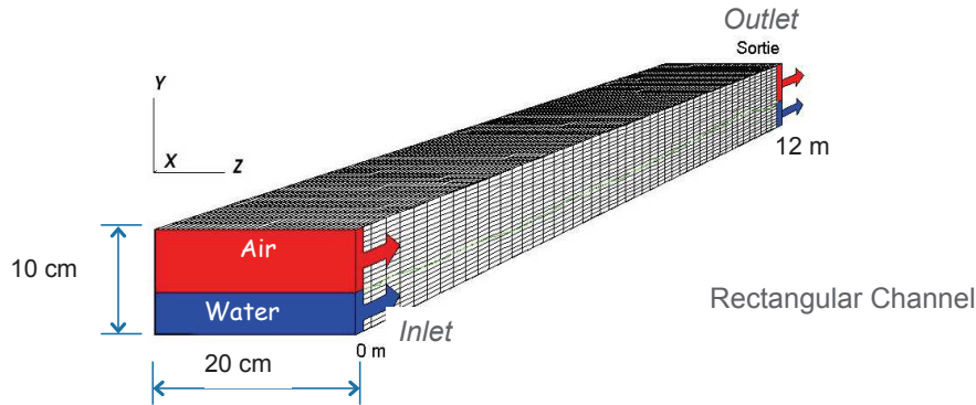
Figure 4.2: The domain in which we solve the flow equations. It has a 0.1 percent slope.
