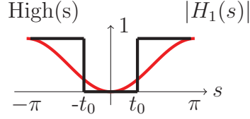
Figure B.3: The magnitude |H_1(s)| is plotted in red. The black function is an ideal high pass filter that cuts the signal inside [-t_0, t_0] .
