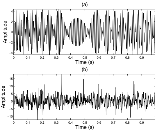
Figure 2.17: Temporal data of noise free signal (a) and with additional nonstationary noise (b).
