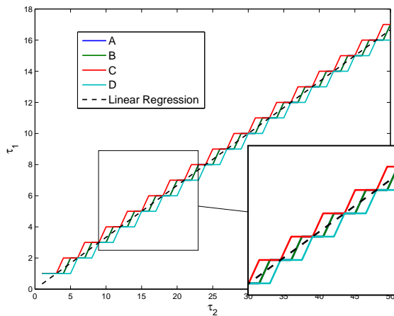
Figure 3.17: Sets of lags [\tau_1, \tau_2] that provide matches for the extremum points.
