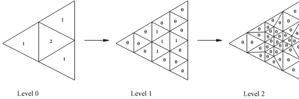
Figure 3.3: Mechanism of multi-level refinement in 2D
