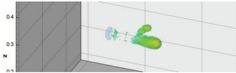
Figure 6.80: Net charge density at times t_1 = 1.68 \cdot 10^{-8} s, 3D view
