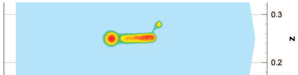
Figure 6.59: Electron density at times t_1 = 1.31 \cdot 10^{-8} s, isolines in a cut plane y = 0.25
