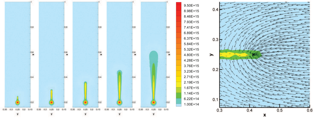
Figure 5.3: 2^{nd} order computation: Electron density (contour levels) at times t = 3.859 \cdot 10^{-8} s , t = 4.435 \cdot 10^{-8} s , t = 4.847 \cdot 10^{-8} s , t = 5.25 \cdot 10^{-8} s and t = 5.659 \cdot 10^{-8} s (end of computation), 2^{nd} order scheme, adapted grid; electron velocity vectors at a head of a discharge (right)
