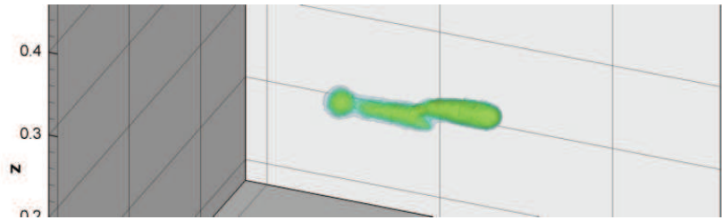
Figure 6.24: Electron density at times t_1 = 1.68 \cdot 10^{-8} s, 3D view
