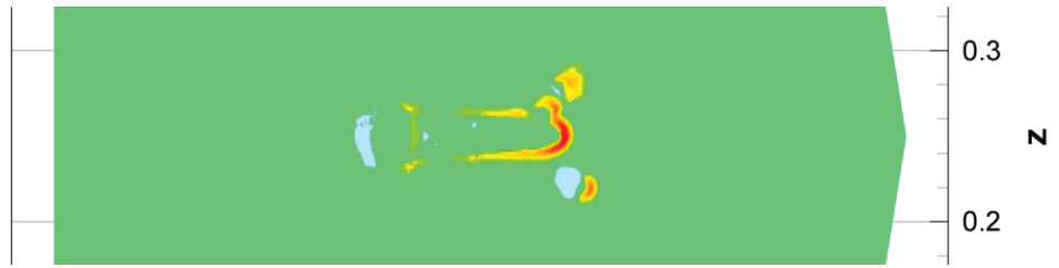
Figure 6.97: Net charge density at times t_1 = 1.36 \cdot 10^{-8} s, isolines in a cut plane y = 0.25
