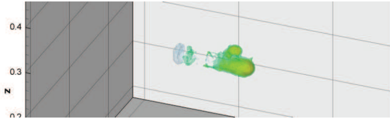
Figure 6.54: Net charge density at times t_1 = 1.47 \cdot 10^{-8} s, 3D view
