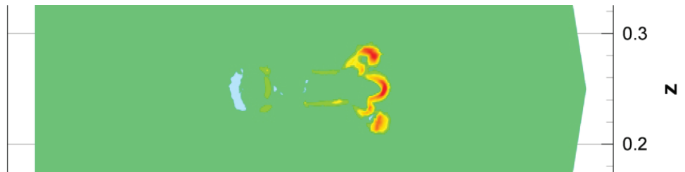
Figure 6.98: Net charge density at times t_1 = 1.47 \cdot 10^{-8} s, isolines in a cut plane y = 0.25
