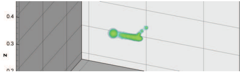
Figure 6.66: Electron density at times t_1 = 1.36 \cdot 10^{-8} s, 3D view
