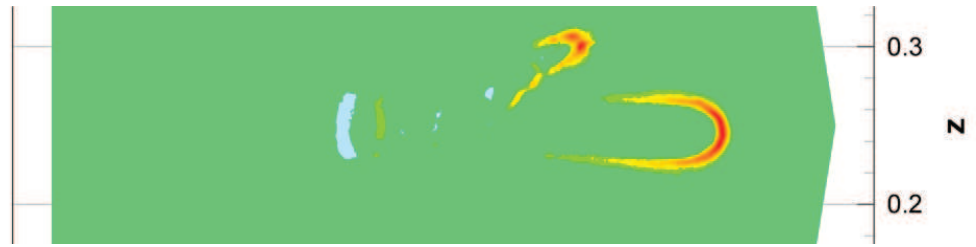
Figure 6.75: Net charge density at times t_1 = 1.89 \cdot 10^{-8} s, isolines in a cut plane y = 0.25
