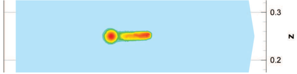
Figure 6.37: Electron density at times t_1 = 1.26 \cdot 10^{-8} s, isolines in a cut plane y = 0.25
