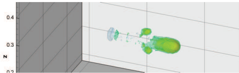
Figure 6.106: Net charge density at times t_1 = 1.89 \cdot 10^{-8} s, 3D view
