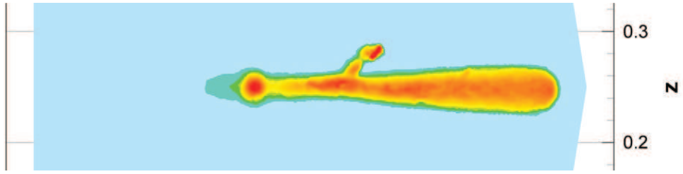
Figure 6.41: Electron density at times t_1 = 1.89 \cdot 10^{-8} s, isolines in a cut plane y = 0.25
