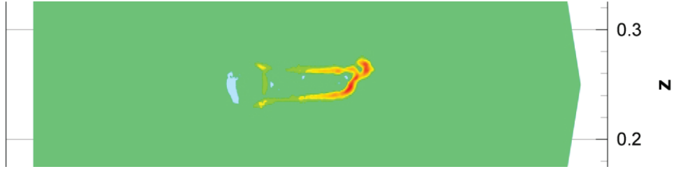
Figure 6.27: Net charge density at times t_1 = 1.31 \cdot 10^{-8} s, isolines in a cut plane y = 0.25
