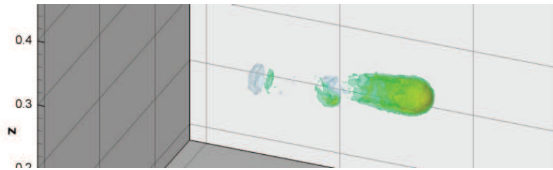
Figure 6.35: Net charge density at times t_1 = 1.89 \cdot 10^{-8} s, 3D view
