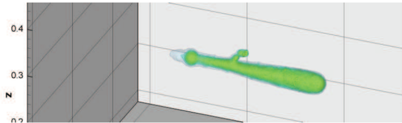
Figure 6.46: Electron density at times t_1 = 1.89 \cdot 10^{-8} s, 3D view
