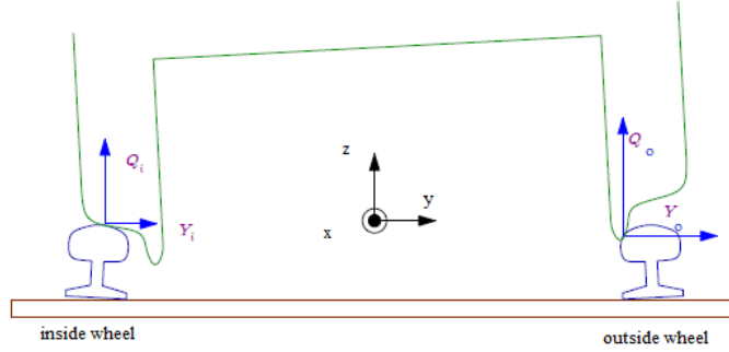
Figure 3.9: Lateral and vertical forces at the wheel-rail contact.
