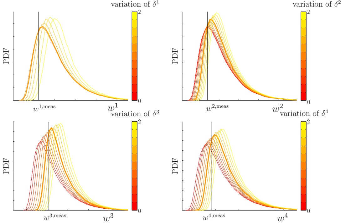
Figure 2.8: Graphs of the PDF, w^\kappa \mapsto p_{W^\kappa(\delta^\kappa)}(w^\kappa; \delta^\kappa) , as a function of \delta^\kappa (the bold line is obtained for \delta^\kappa = \delta^{\kappa,\text{opt}} ), for \kappa = 1, 2, 3, 4 .
