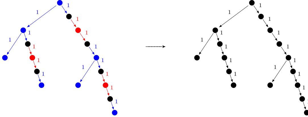
Figure 3.9: \mathcal{T}_2 and \mathcal{T}_2^{\text{unco}} in the proof of Theorem 3.3.
