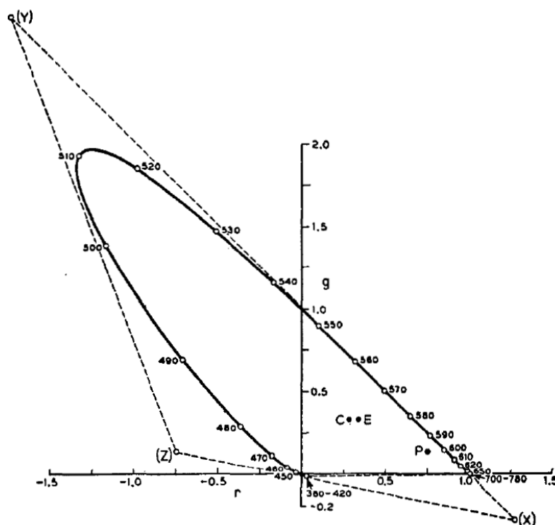
Figure 3.14: rg chromaticity diagram. Image from [LRT77].
