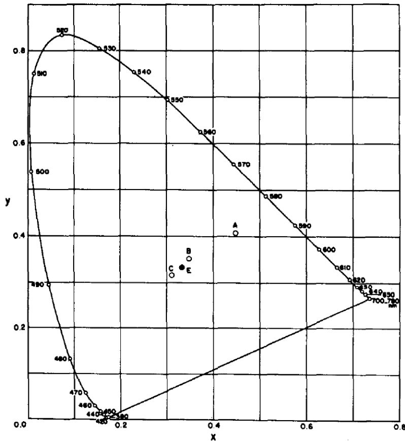
Figure 3.16: CIE xy diagram. Image from [LRT77].
