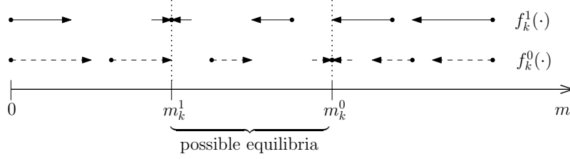
Figure 4.1: Representation of fluid equilibria and drift functions when m_k^1 < m_k^0 .
