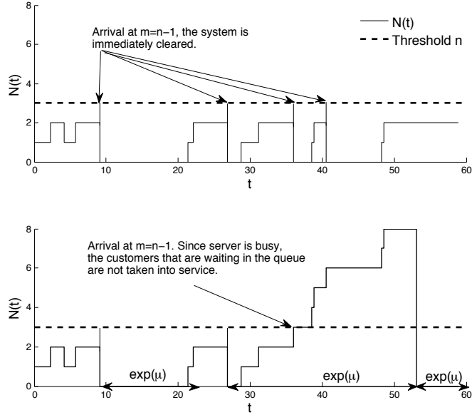
Figure 6.1: Simulation of process N(t) , number of waiting customers at time t , under threshold n = 3 . Above the \mu = \infty case, below the \mu < \infty case. Below \text{exp}(\mu) refers to the busy period of the server, which is exponentially distributed with rate \mu < \infty . As a consequence N(t) not only depends on n but also on the length of each busy period.
