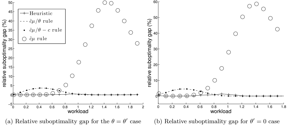
Figure 5.10: Performance comparison of policies for K = 3 .
