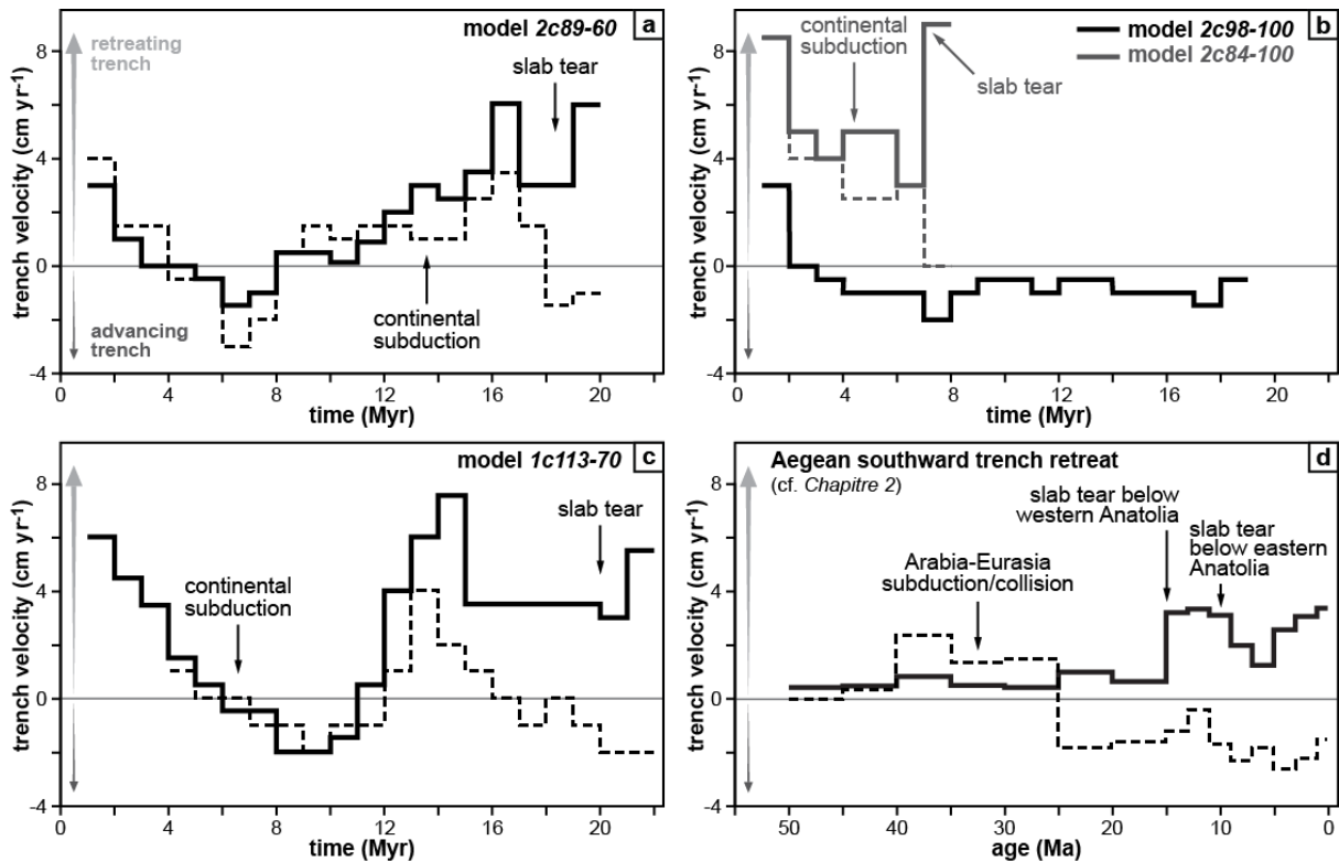
Figure 5.11: time-trench velocity diagram showing the trench migration of both oceanic and oceanic-continental subduction zones obtained from models 2c89-60 (a), 2c98-100 , 2c84-100 (b) and 1c113-70 (c) and from kinematic reconstructions of the eastern Mediterranean region (d) (cf. Chapitre 2 ). Solid and dashed lines correspond to only oceanic (or Hellenic) and oceanic-continental (or eastern Anatolia) subduction zones, respectively. Positive and negative distances correspond to retreating and advancing trench, respectively. The initiation of continental subduction and slab tearing processes are highlighted for each diagram.
