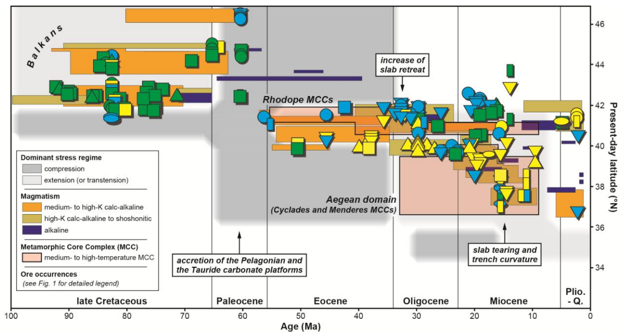
Figure 3.3: spatial and temporal distribution of magmatism and compiled mineral occurrences in the Balkan-Rhodope-Aegean-west Anatolian region since the late Cretaceous. On this latitude/age diagram are represented, for each domain, the dominant active stress regime within the upper plate, the magmatic activity, the exhumation stage of the main metamorphic core complexes (MCCs) and the compiled mineral occurrences.
