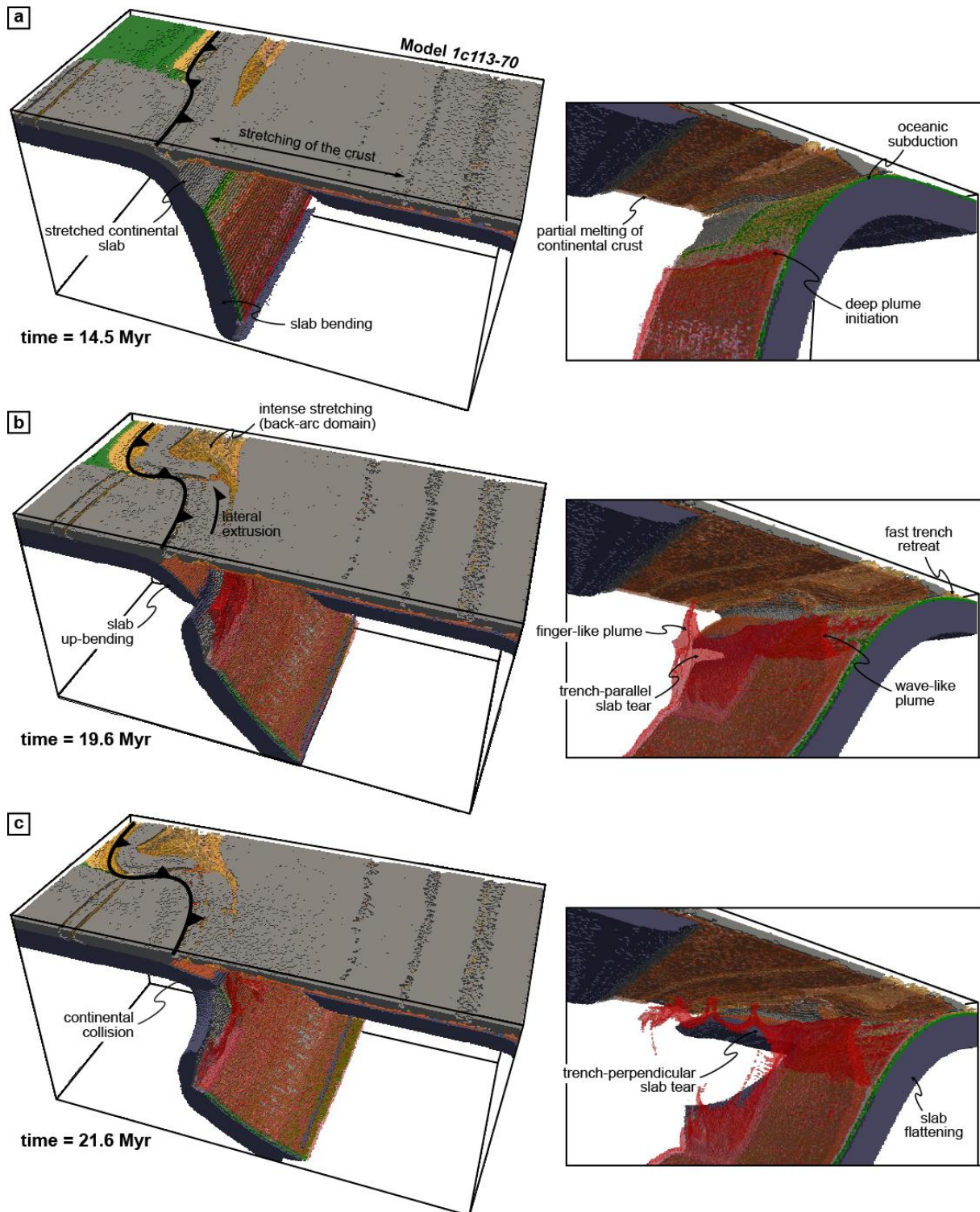
Figure 5.10: evolution of the model 1c113-70 (with a one-layer continental crust). (a, b, c) 3D lateral view of the subduction zone (left panels) and zoom on the mantle wedge (right panels) for selected time steps. Colors represent the different rock types (see figure 5.7 for detailed legend). Asthenosphere and other phases are cut off for clarity.
