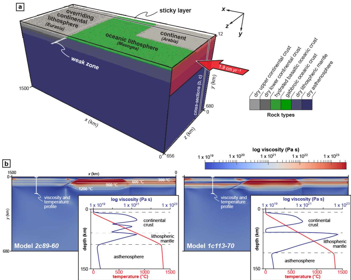
Figure 5.6: initial model setup. (a) 3D model domain with colors representing the different rock types. Air and sea water phases (composing the sticky layer) are cut off for clarity. (b) x - y viscosity cross-sections of the initial model domain with a two-layer (left panel) and one-layer (right panel) continental crust. White lines represent 300, 600, 900 and 1200 °C isotherms. Vertical viscosity (blue) and temperature (red) profiles are shown as inset for each model.
