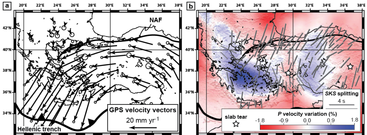
Figure 5.5: geophysical maps of the eastern Mediterranean region. (a) GPS velocities relative to stable Eurasia with 1\sigma confidence ellipses [ Reilinger et al. , 2006]. (b) Seismic tomographic model, showing the V_p anomalies at \sim 150 km depth [ Li et al. , 2008]. Slab tear suspected in the region are highlighted by white stars. Station-averaged SKS splitting data are also highlighted [ Paul et al. , 2014].
