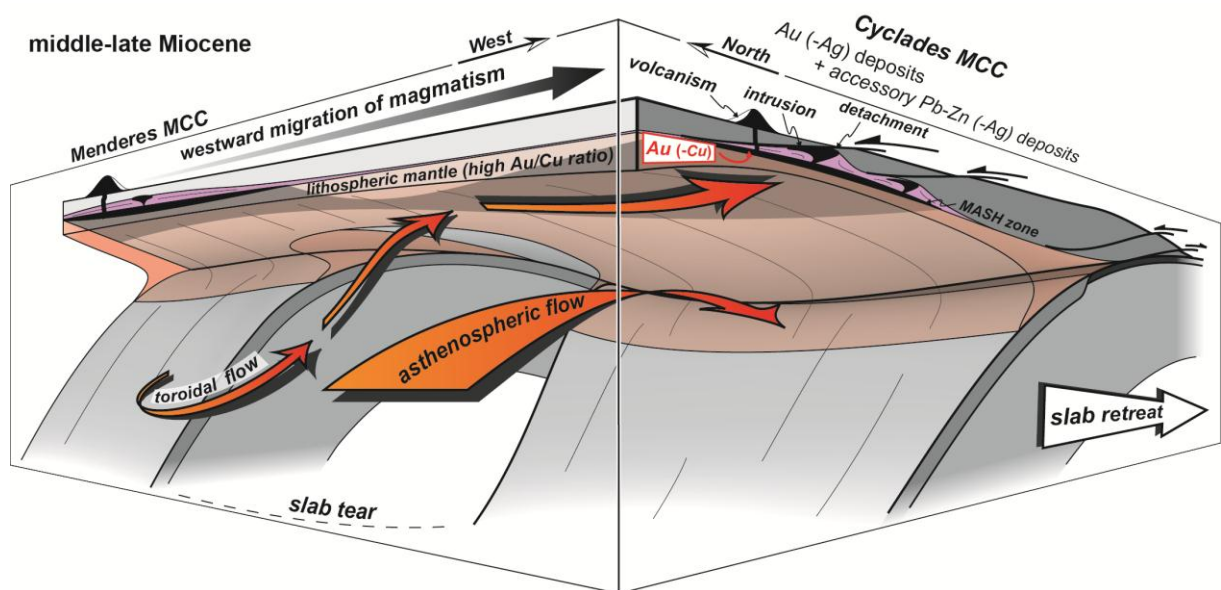
Figure 3.5: 3D lateral view from below of the Eastern Mediterranean subduction zone geometry in the middle-late Miocene. On this cartoon are shown the asthenospheric flows, resulting from both slab retreat and slab tearing. The asthenospheric flow with a dominant toroidal component (i.e. in a horizontal plane) thus results in the westward migration of magmatic activity and associated ore deposition, from the Menderes massif to the Cyclades.
