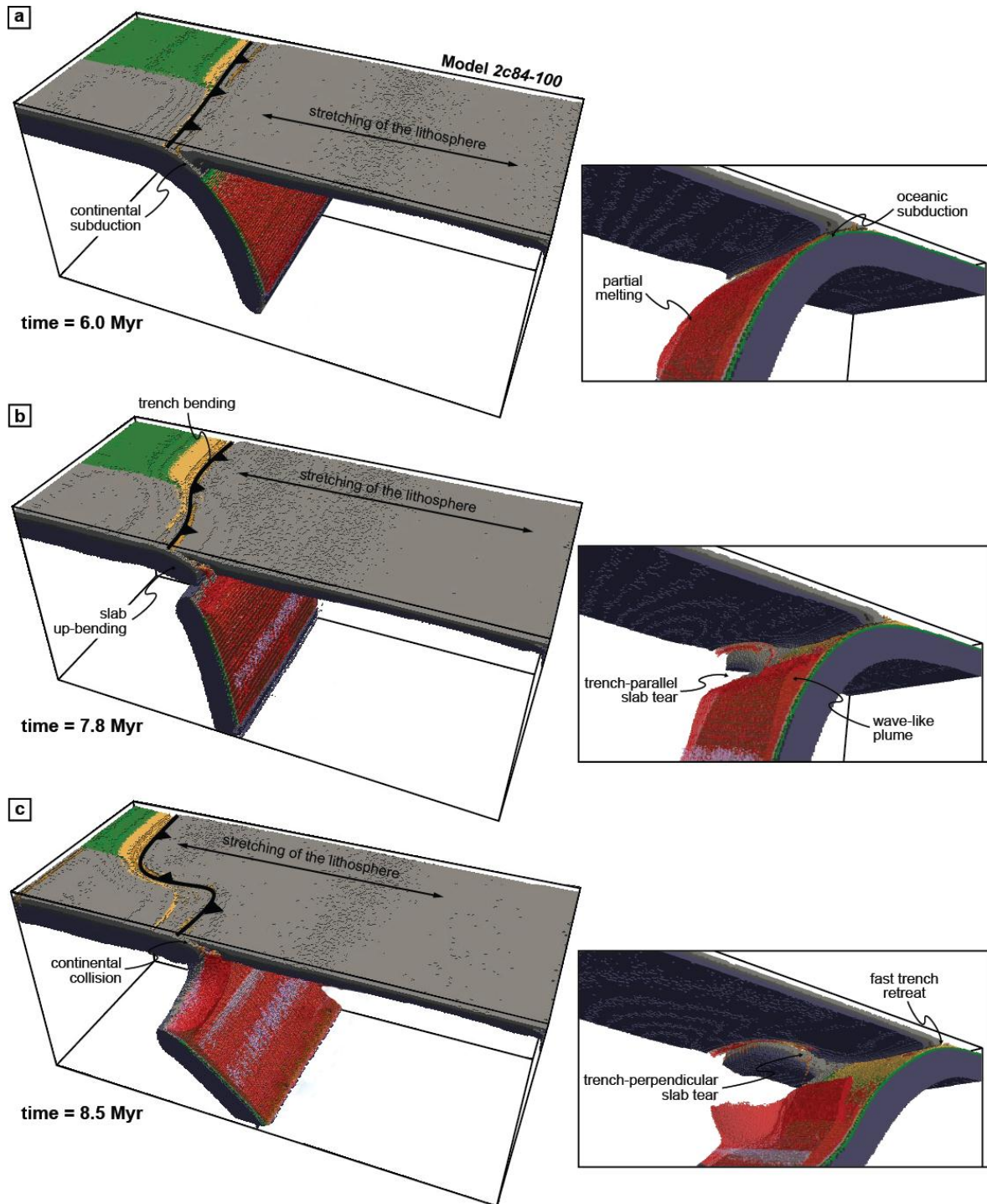
Figure 5.8: evolution of the model 2c84-100 . (a, b, c) 3D lateral view of the subduction zone (left panels) and zoom on the mantle wedge (right panels) for selected time steps. Colors represent the different rock types (see figure 5.7 for detailed legend). Asthenosphere and other phases are cut off for clarity.
