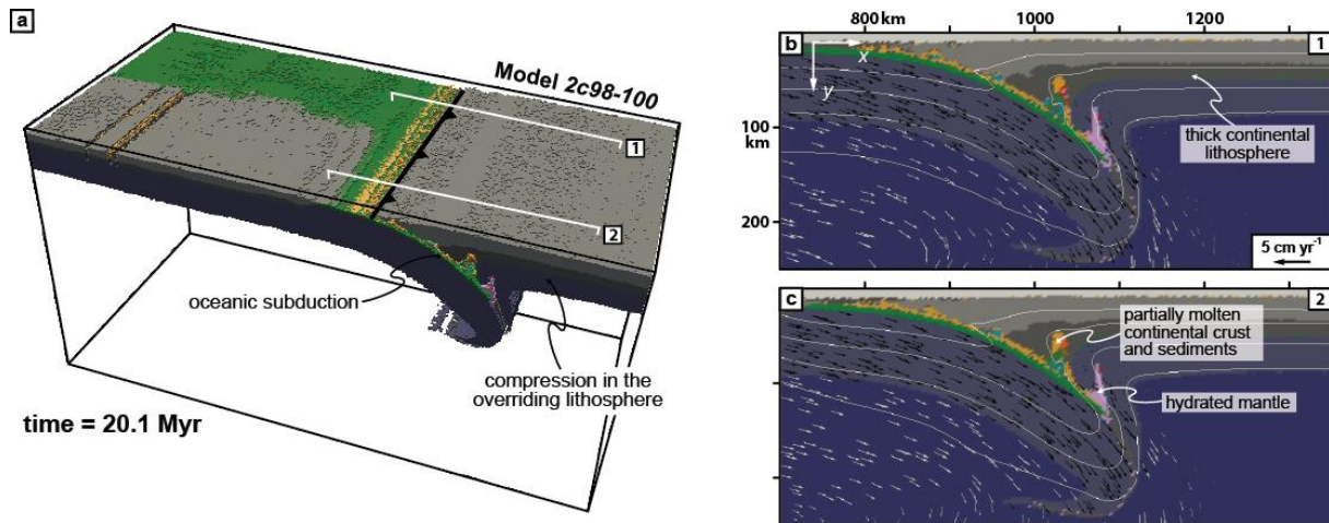
Figure 5.9: subduction geometry of the model 2c98-100 , displaying a relatively strong coupling between both interacting lithospheres. (a) 3D lateral view of the subduction zone, highlighting the compressional tectonics in the overriding continental lithosphere. (b, c) x - y cross-sections of the subduction zone, highlighting the restrained magmatic activity in the mantle wedge and the low velocity field in both the subducting lithosphere and the underlying asthenosphere (see figure 5.7 for detailed legend).
