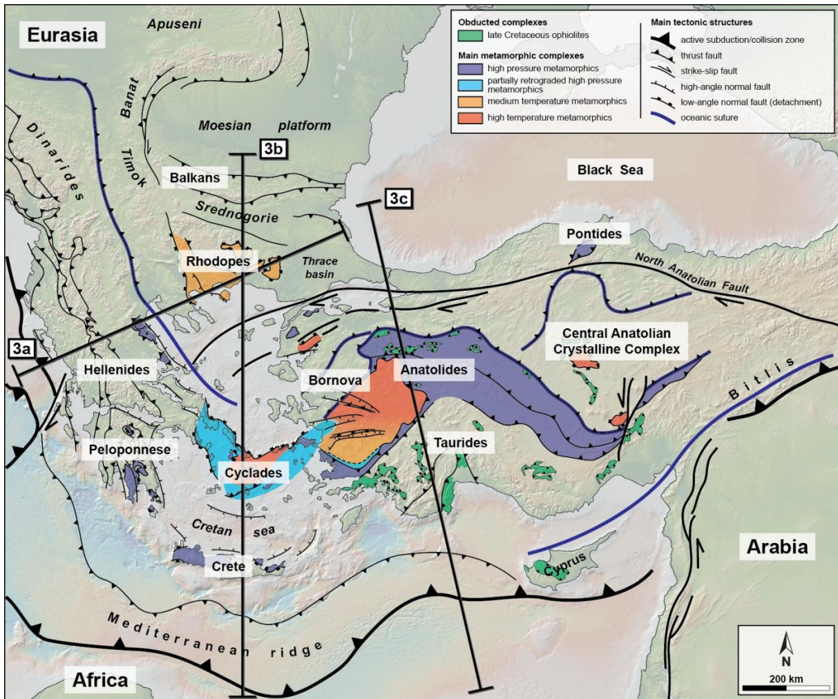
Figure 2.2: tectonic map of the eastern Mediterranean region highlighting the main tectono-metamorphic domains. Modified from Jolivet et al. [2013]. Base maps made with GeoMapApp ( https://www.geomapapp.org ).
