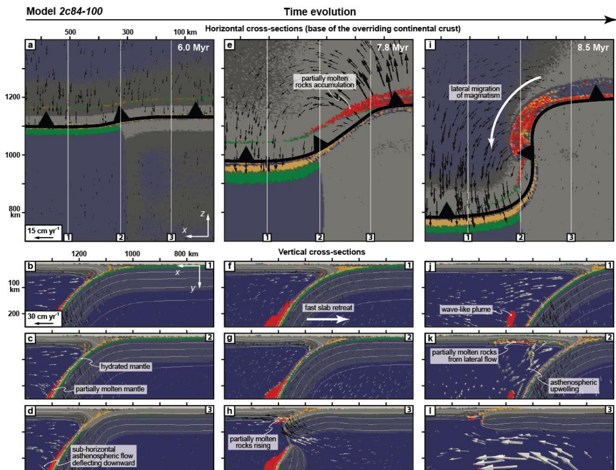
Figure 5.14: evolution of magmatism in model 2c84-100. x - z plan views (a, e, i) and x - y cross-sections (b, c, d, f, g, h, j, k, l) of the subduction zone for selected time steps. Colors represent the different rock types (see figure 5.7 for detailed legend). Black and white arrows represent velocity vectors in the continental crust (top panels) or lithospheric mantle (bottom panels) and the asthenosphere, respectively. Scale of velocity vectors is twice larger in top panels than in bottom panels. White lines (bottom panels) represent 300, 600, 900 and 1200 °C isotherms.
